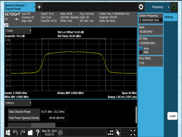
11N20SISO-Ant2-5180
