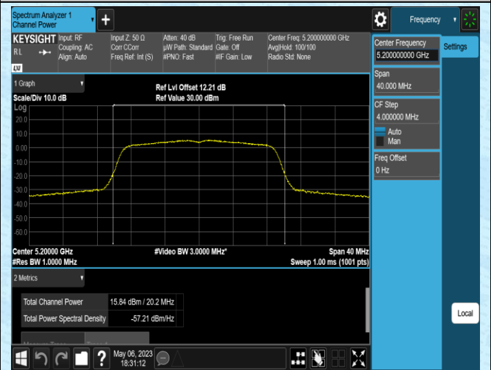
11N20SISO-Ant2-5200
