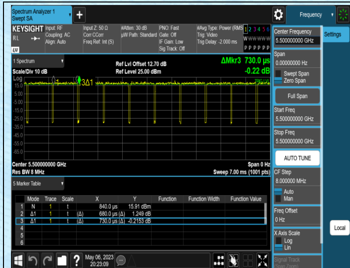
NTNV-11AC20MIMO-Ant1-5500
