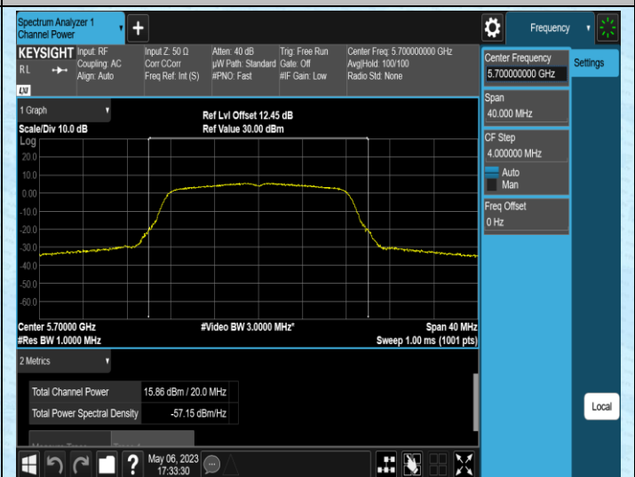
11A-Ant2-5700
