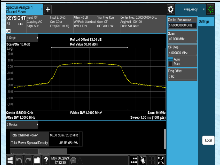
11A-Ant2-5580
