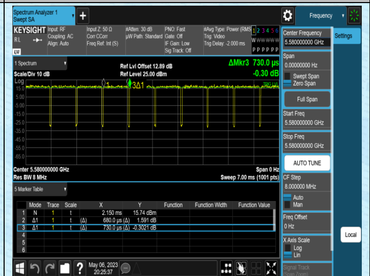
NTNV-11AC20MIMO-Ant2-5580
