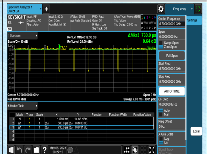
NTNV-11AC20MIMO-Ant2-5700
