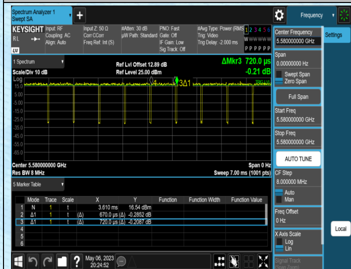
NTNV-11AC20MIMO-Ant1-5580
