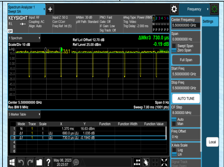
NTNV-11AC20MIMO-Ant2-5500
