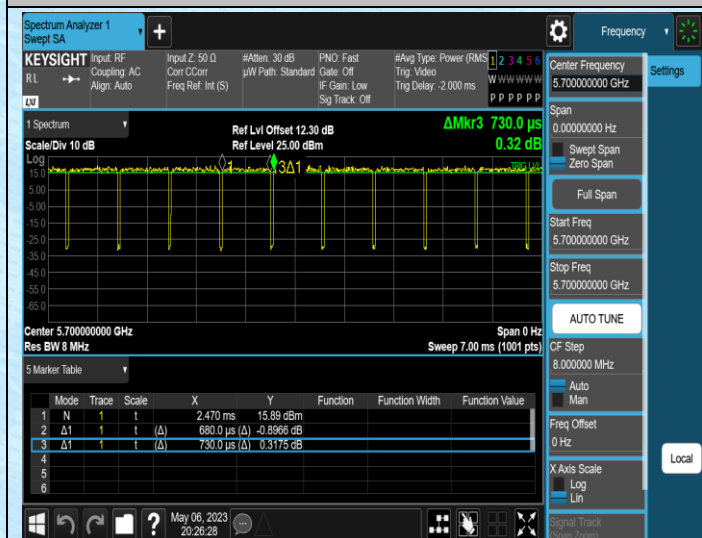
NTNV-11AC20MIMO-Ant1-5700
