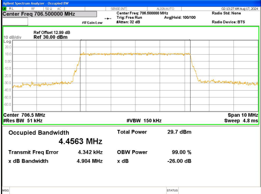
Band 17 5MHz/706.5/Low QPSK 25@0
