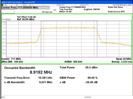
Band 17 10MHz/711.0/High QPSK 50@0
