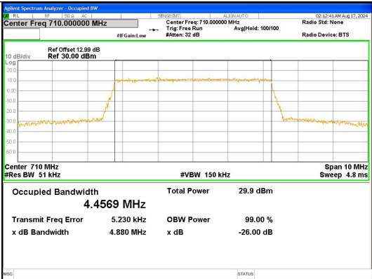
Band 17 5MHz/710.0/Mid QPSK 25@0
