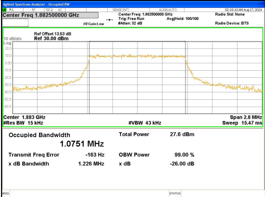
Band 25 1.4MHz/1882.5/Mid 16QAM 6@0
