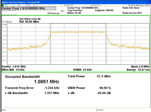
Band 25 1.4MHz/1914.3/High 16QAM 6@0
