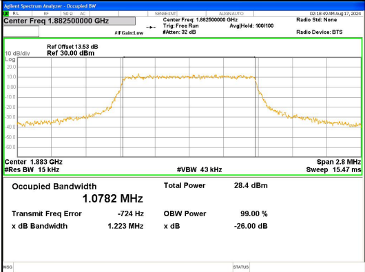
Band 25 1.4MHz/1882.5/Mid QPSK 6@0
