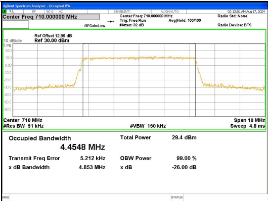
Band 17 5MHz/710.0/Mid 16QAM 25@0
