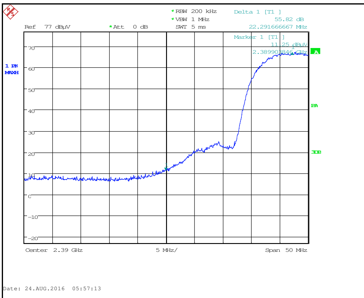
Plot 4-1: Lower Band Edge – 802.11b (Antenna #1)
