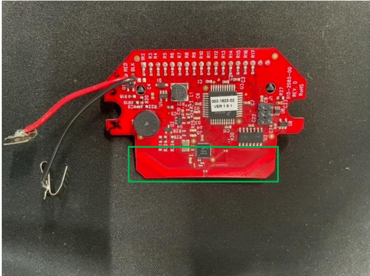
Figure 2: Top Side of the Wireless Remote Hand Control PCB Antenna location is denoted by the green square.
