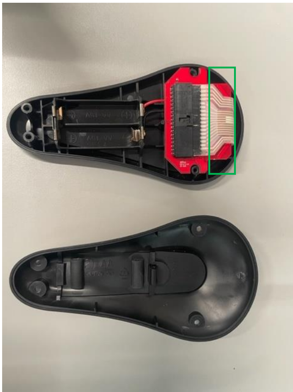
Figure 1: Inside of the Wireless Remote Hand Control Antenna location is denoted by the green square.
