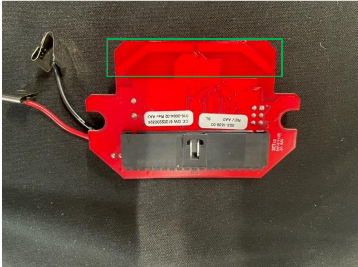
Figure 3: Bottom Side of the Wireless Remote Foot Control PCB Antenna location is denoted by the green square.
