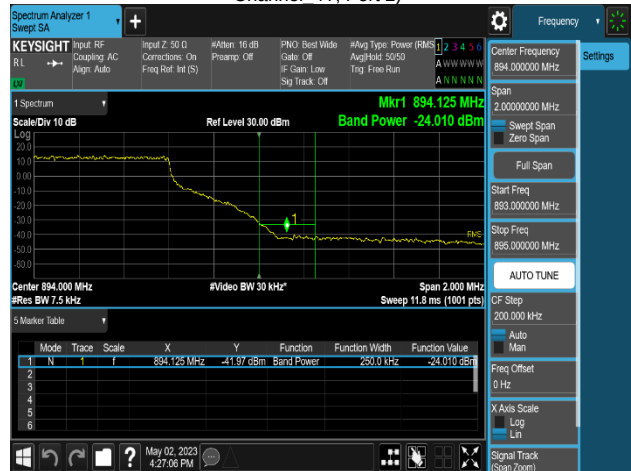
Plot 8-400. Band Edge Emission Summary Data Plot (MSR 2C_DSS B(n)5_1C_10M+NR n5_1C_15M_16QAM - High Channel 4T, Port 1)
