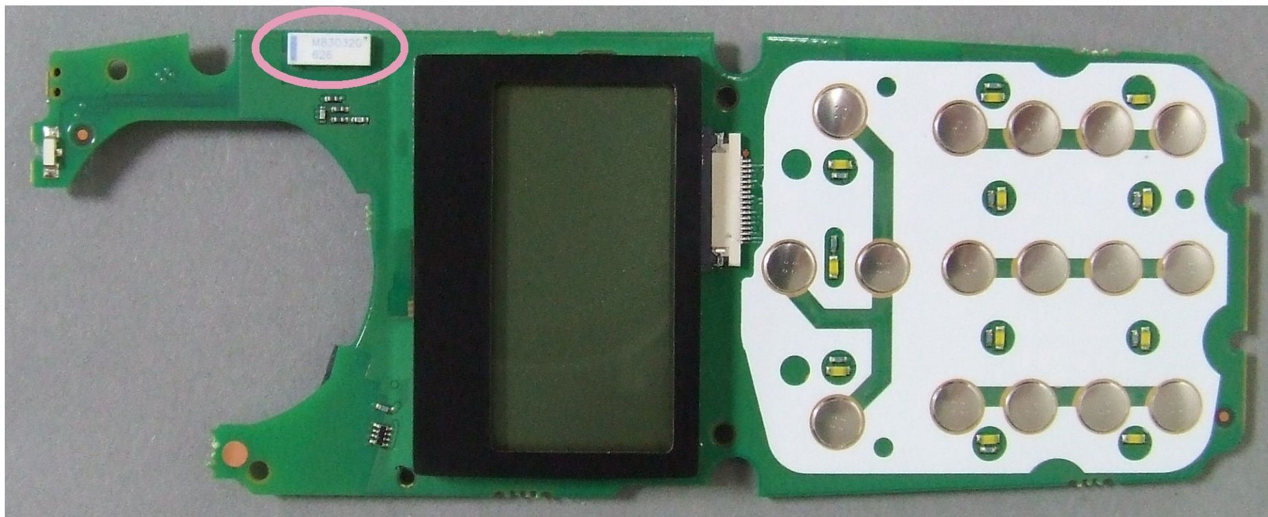
Photograph 02: Control PCB – bottom. BT antenna circled.
