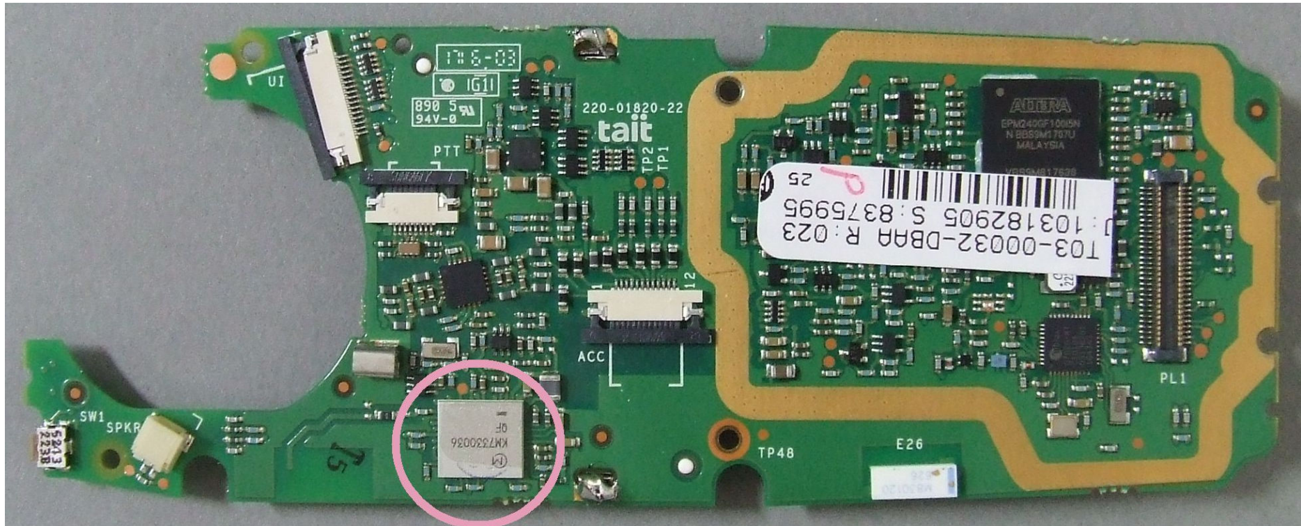
Photograph 01: Control PCB – top. BT module circled.
