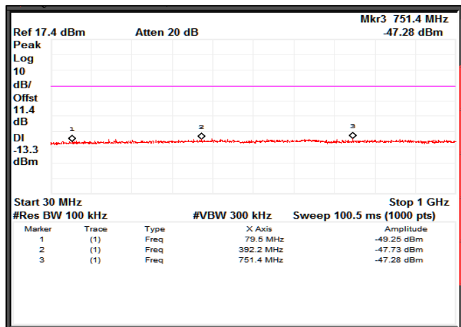
Channel Frequency 2480MHz Frequency Range 30 MHz – 1GHz
