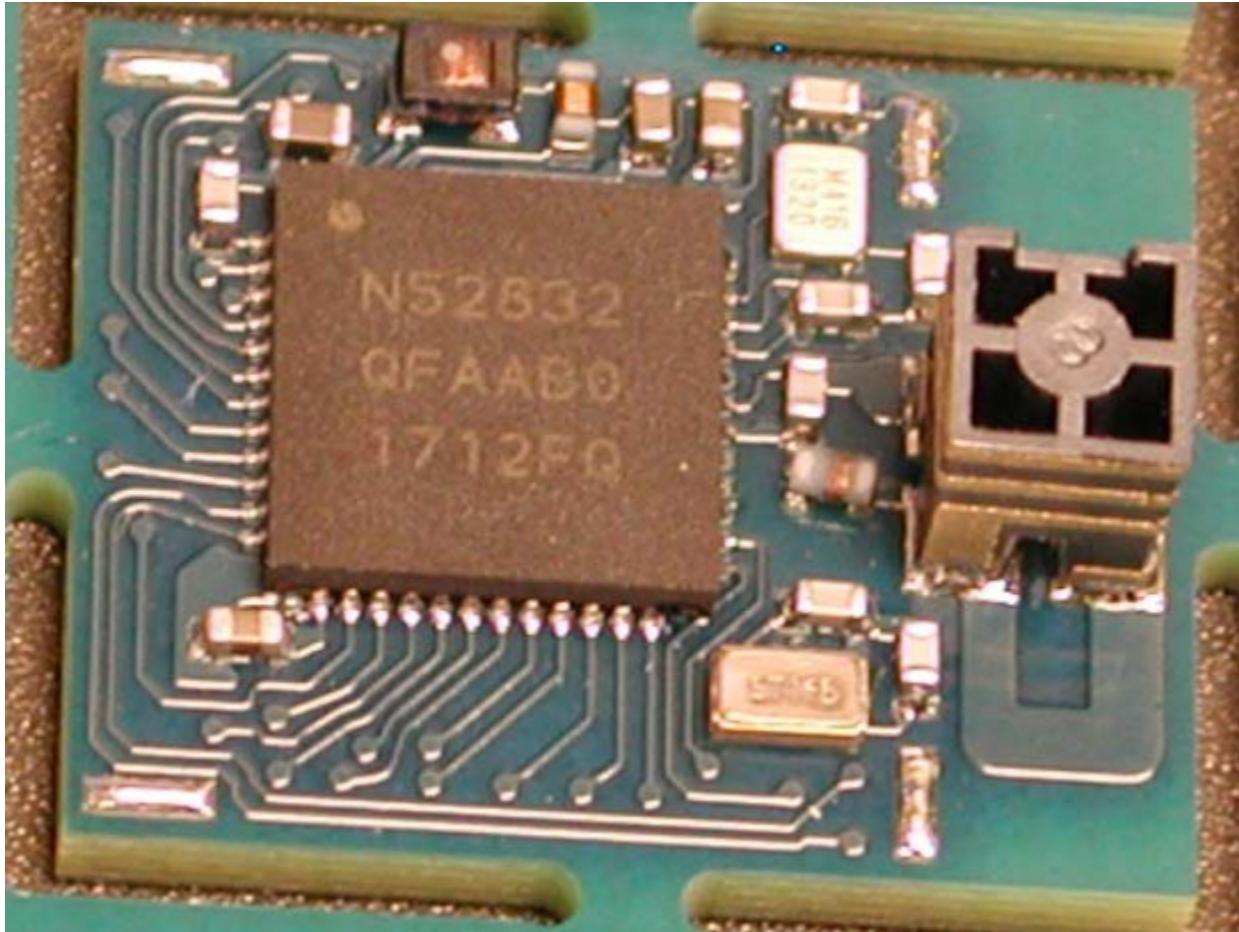
TOP PCB W/O SHIELD
