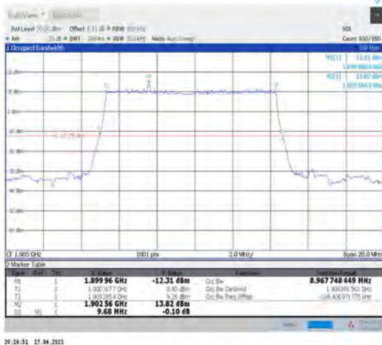
1-N2--15-10-H-2-DFT-PI2BPSK-Outer_Full-50@0-Ant1-8.968-9.680-≤10-PASS
