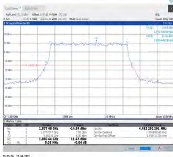
1-N2--15-5-M-3-DFT-16QAM-Outer_Full-25@0-Ant1-4.482-5.050-≤5-PASS
