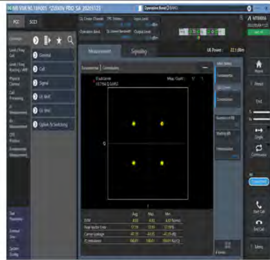
1-N2-PC3-15-20-M-6-CP-QPSK-Outer_Full-106@0-Ant1-see graph-PASS
