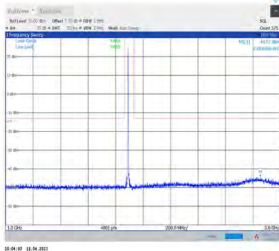
1-N2--15-20-H-1-DFT-PI2BPSK-Inner_1RB_Left- 1@1-1000-3000-Ant1--44.57--13-PASS
