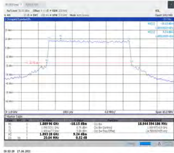
1-N2--15-20-H-7-CP-16QAM-Outer_Full-106@0-Ant1-18.945-20.040-≤20-PASS
