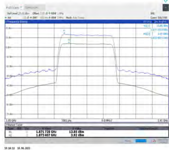
1-N2--15-20-M-2-CP-256QAM-Outer_Full-106@0-Ant1-9.93-100%-0.00-9.93-PASS-≤13
