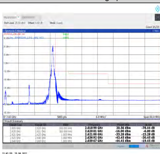
1-N38--30-20-H-5-CP-QPSK-Edge_1RB_Right-1@50- Ant1-PASS-see graph
