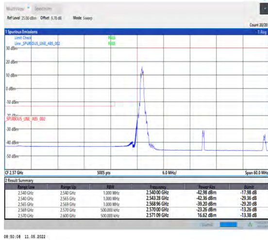
1-N38-PC2-30-30-L-4-CP-QPSK-Edge_1RB_Left-1@0 -Ant1-PASS-see graph
