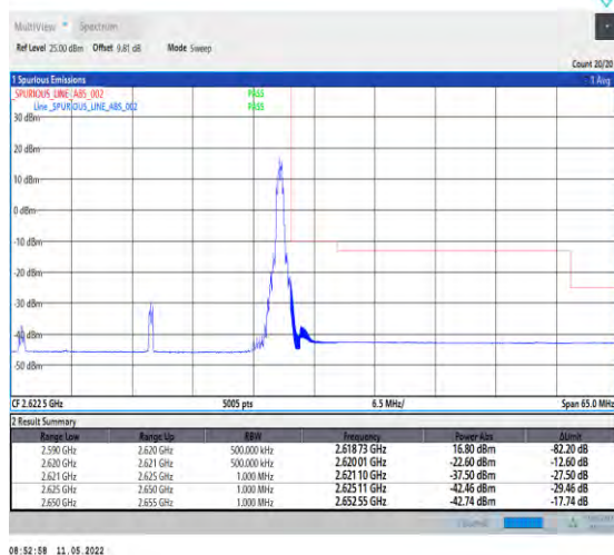
1-N38-PC2-30-30-H-5-CP-QPSK-Edge_1RB_Right-1@ 77-Ant1-PASS-see graph
