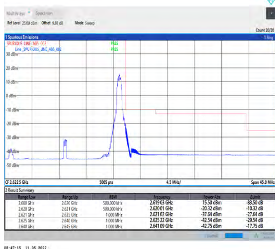
1-N38-PC2-30-20-H-5-CP-QPSK-Edge_1RB_Right-1@ 50-Ant1-PASS-see graph
