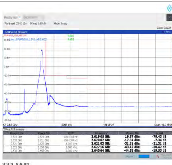
1-N38--30-10-H-2-DFT-PI2BPSK-Edge_1RB_Right-1@23-Ant1-PASS-see graph
