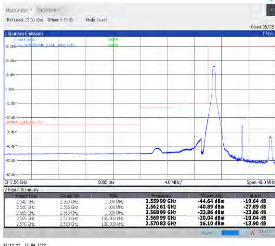
1-N38--30-10-L-4-CP-QPSK-Edge_1RB_Left-1@0-Ant1-PASS-see graph
