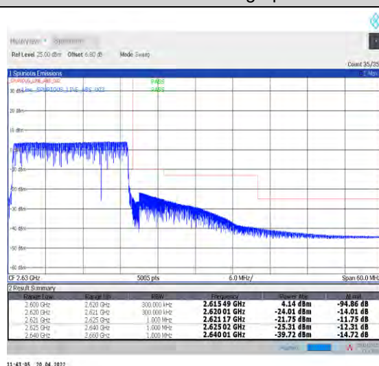
1-N38--30-20-H-6-CP-QPSK-Outer_Full-51@0-Ant1- PASS-see graph
