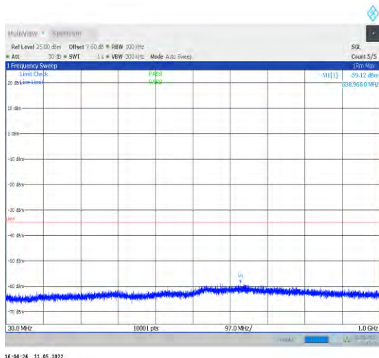
1-N38-PC2-30-40-M-1-DFT-QPSK-Edge_1RB_Left-1 @0-30-1000-Ant1--59.12--35-PASS
