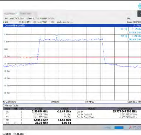
1-N38--30-40-M-3-DFT-16QAM-Outer_Full-100@0- Ant1-35.777-38.320-<40-PASS
