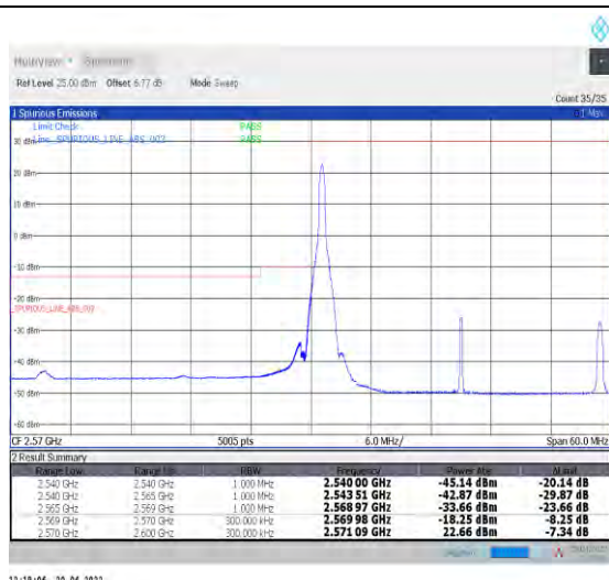
1-N38--30-30-L-1-DFT-PI2BPSK-Edge_1RB_Left-1@0-Ant1-PASS-see graph
