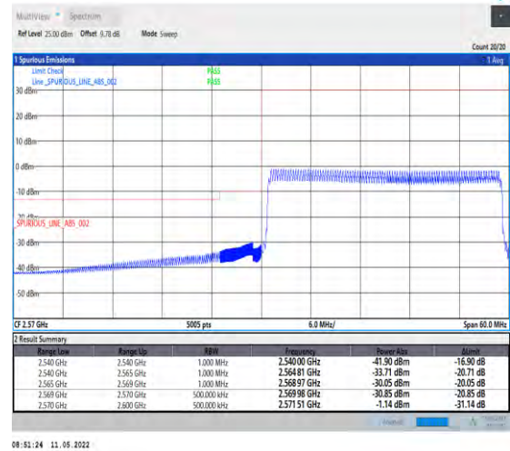
1-N38-PC2-30-30-L-6-CP-QPSK-Outer_Full-78@ 0-Ant1-PASS-see graph
