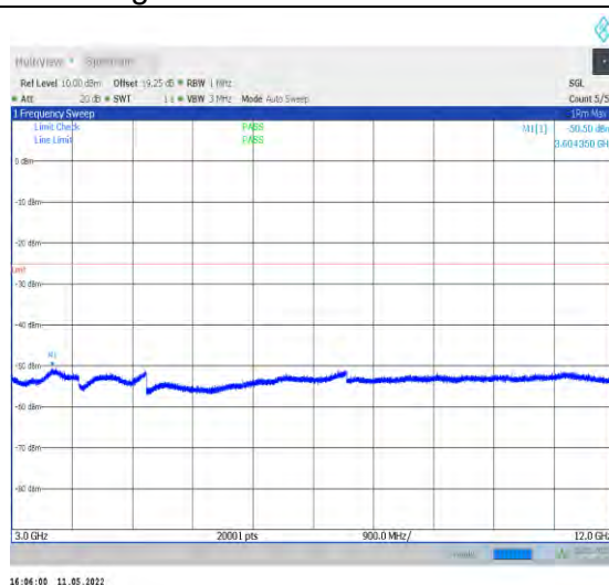
1-N38-PC2-30-40-H-1-DFT-QPSK-Edge_1RB_Left-1 @0-3000-12000-Ant1--50.50--25-PASS
