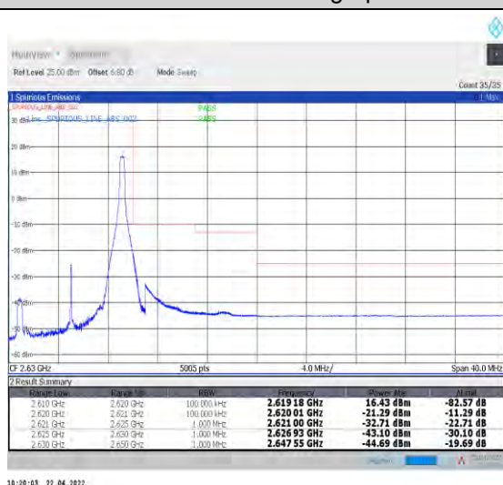
1-N38--30-10-H-5-CP-QPSK-Edge_1RB_Right-1@23-Ant1-PASS-see graph
