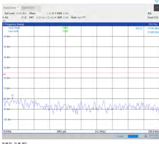
1-N38--30-40-M-1-DFT-PI2BPSK-Inner_1RB_Left-1 @1-0.009-0.15-Ant1--79.96--55-PASS
