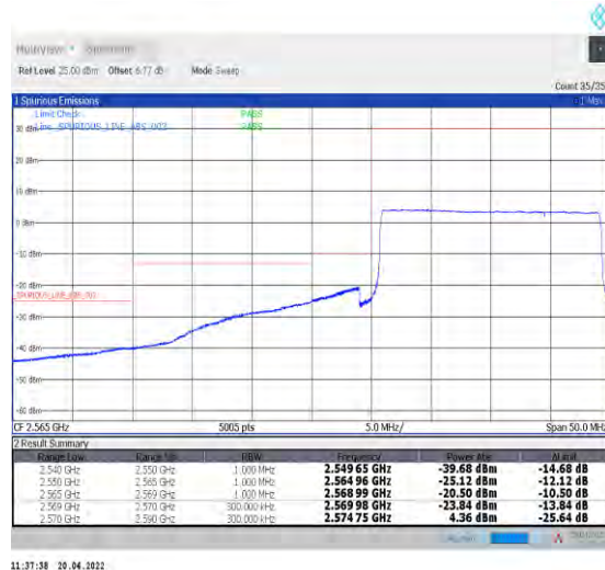
1-N38--30-20-L-6-CP-QPSK-Outer_Full-51@0-Ant1-PASS-see graph
