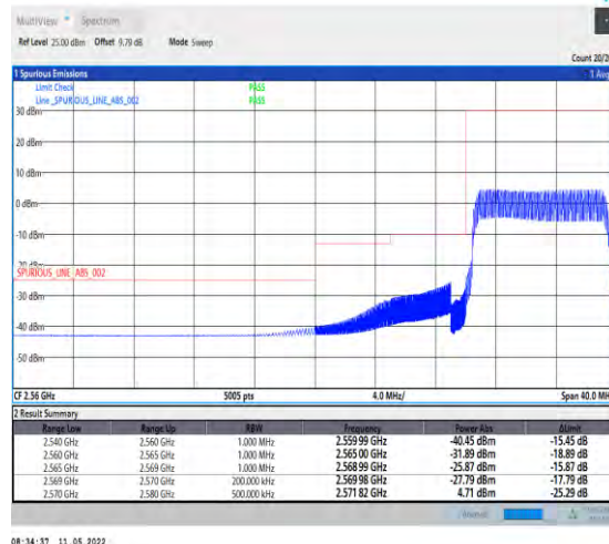
1-N38-PC2-30-10-L-6-CP-QPSK-Outer_Full-24@ 0-Ant1-PASS-see graph
