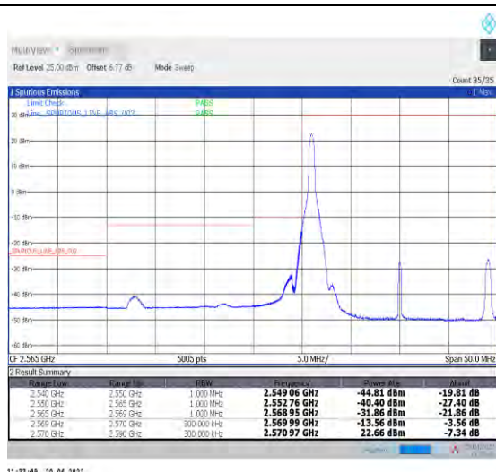
1-N38--30-20-L-1-DFT-PI2BPSK-Edge_1RB_Left-1@0-Ant1-PASS-see graph
