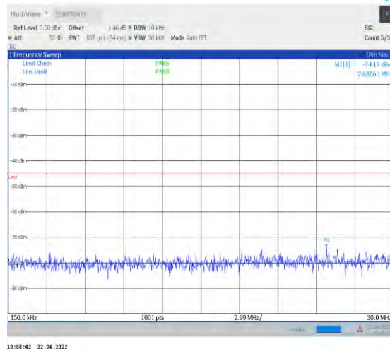
1-N38--30-40-H-1-DFT-PI2BPSK-Inner_1RB_Left-1 @1-0.15-30-Ant1--74.17--45-PASS
