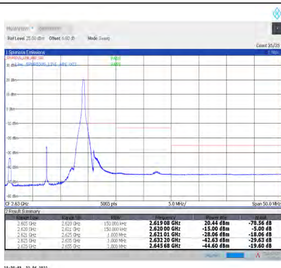
1-N38--30-15-H-2-DFT-PI2BPSK-Edge_1RB_Right-1@37-Ant1-PASS-see graph
