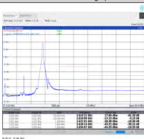
1-N38--30-15-H-5-CP-QPSK-Edge_1RB_Right-1@37-Ant1-PASS-see graph
