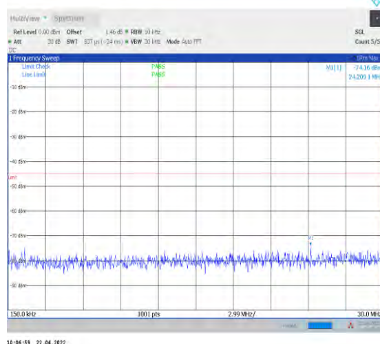
1-N38--30-40-M-1-DFT-PI2BPSK-Inner_1RB_Left-1 @1-0.15-30-Ant1--74.16--45-PASS
