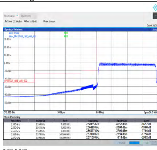
1-N38-PC2-30-20-L-6-CP-QPSK-Outer_Full-51@ 0-Ant1-PASS-see graph
