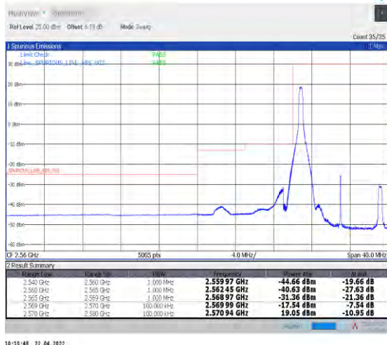
1-N38--30-10-L-1-DFT-PI2BPSK-Edge_1RB_Left-1@0-Ant1-PASS-see graph
