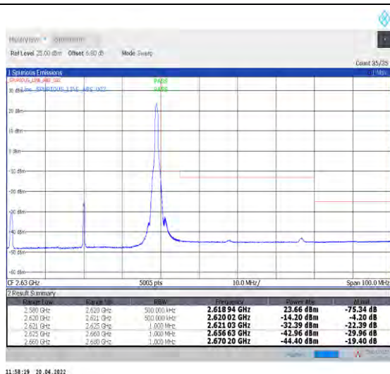
1-N38--30-40-H-2-DFT-PI2BPSK-Edge_1RB_Right-1@ 105-Ant1-PASS-see graph
