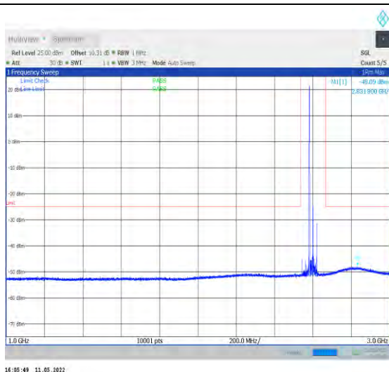
1-N38-PC2-30-40-H-1-DFT-QPSK-Edge_1RB_Left-1 @0-1000-3000-Ant1--48.09--25-PASS
