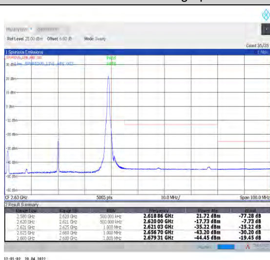
1-N38--30-40-H-5-CP-QPSK-Edge_1RB_Right-1@105 -Ant1-PASS-see graph
