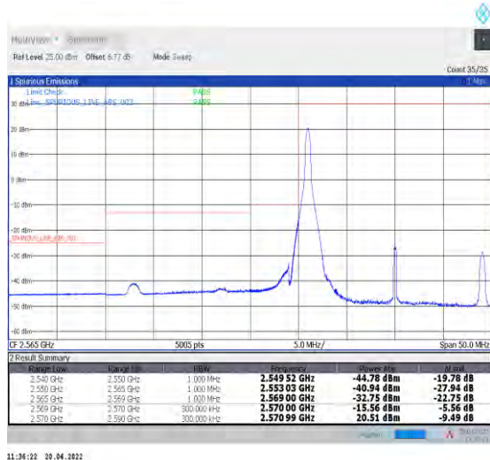
1-N38--30-20-L-4-CP-QPSK-Edge_1RB_Left-1@0-Ant1-PASS-see graph
