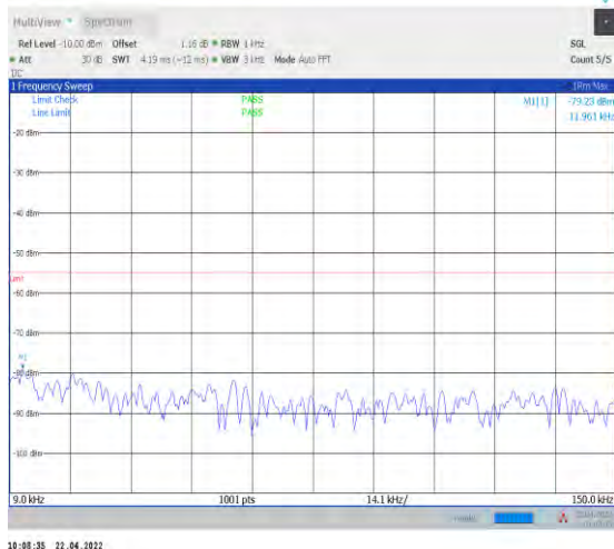
1-N38--30-40-H-1-DFT-PI2BPSK-Inner_1RB_Left-1 @1-0.009-0.15-Ant1--79.23--55-PASS
