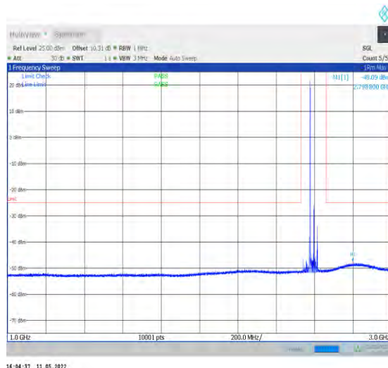
1-N38-PC2-30-40-M-1-DFT-QPSK-Edge_1RB_Left-1 @0-1000-3000-Ant1--48.09--25-PASS
