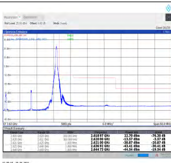
1-N38--30-20-H-2-DFT-PI2BPSK-Edge_1RB_Right-1@ 50-Ant1-PASS-see graph
