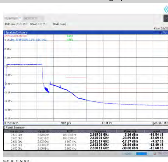
1-N38--30-10-H-6-CP-QPSK-Outer_Full-24@0-Ant1-PASS-see graph
