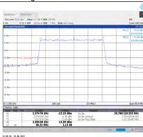
1-N38--30-40-M-1-DFT-QPSK-Outer_Full-100@0-An t1-35.78-38.320-<40-PASS
