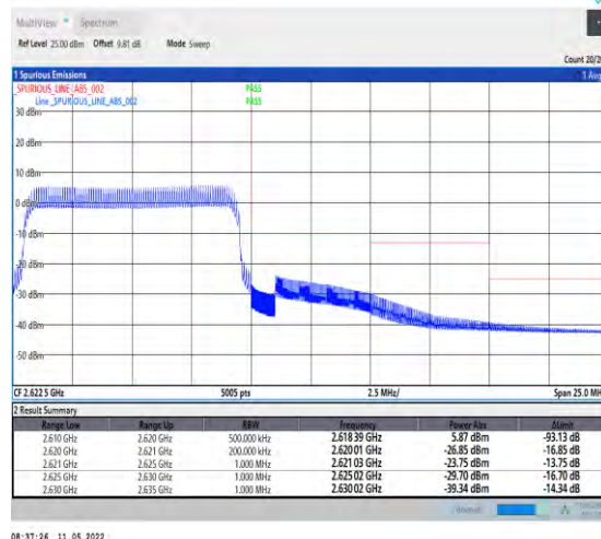
1-N38-PC2-30-10-H-6-CP-QPSK-Outer_Full-24@ 0-Ant1-PASS-see graph
