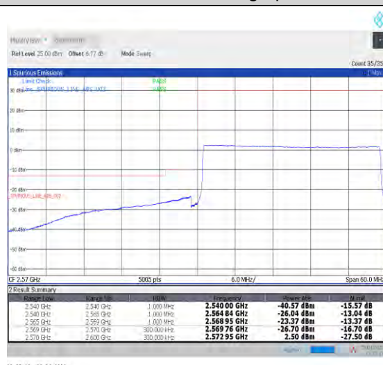
1-N38--30-30-L-6-CP-QPSK-Outer_Full-78@0-Ant1-PASS-see graph
