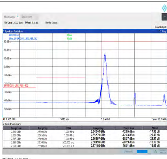
1-N38-PC2-30-20-L-4-CP-QPSK-Edge_1RB_Left-1@0 -Ant1-PASS-see graph
