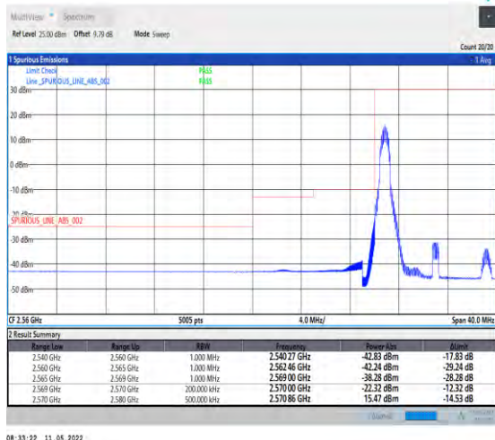
1-N38-PC2-30-10-L-4-CP-QPSK-Edge_1RB_Left-1@0 -Ant1-PASS-see graph
