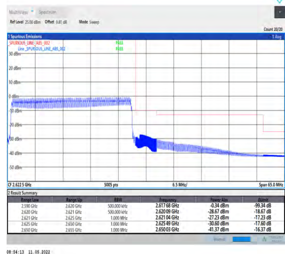
1-N38-PC2-30-30-H-6-CP-QPSK-Outer_Full-78@ 0-Ant1-PASS-see graph
