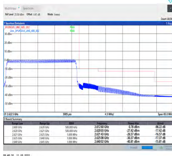
1-N38-PC2-30-20-H-6-CP-QPSK-Outer_Full-51@ 0-Ant1-PASS-see graph
