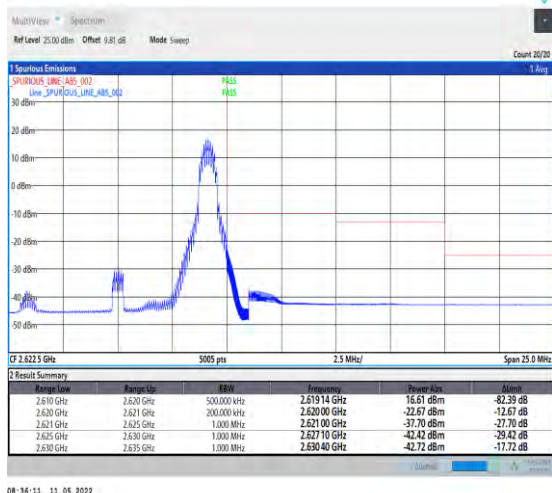
1-N38-PC2-30-10-H-5-CP-QPSK-Edge_1RB_Right-1@ 23-Ant1-PASS-see graph
