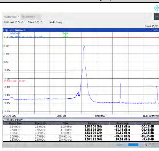
1-N38--30-30-L-4-CP-QPSK-Edge_1RB_Left-1@0-Ant1-PASS-see graph
