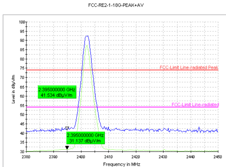
Fig.27. Radiated emission (Power): GFSK low channel
