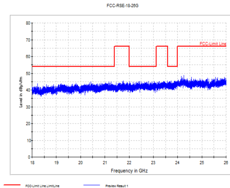
Fig.29. Radiated emission: GFSK, 18 GHz - 26 GHz
