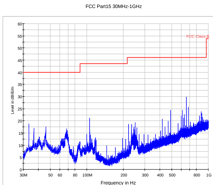
Fig.18. Radiated emission: GFSK, 2402MHz, 30 MHz - 1 GHz
