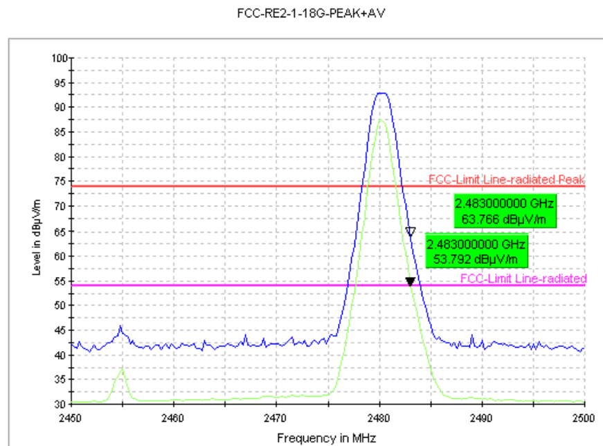
Fig.28. Radiated emission (Power): GFSK high channel
