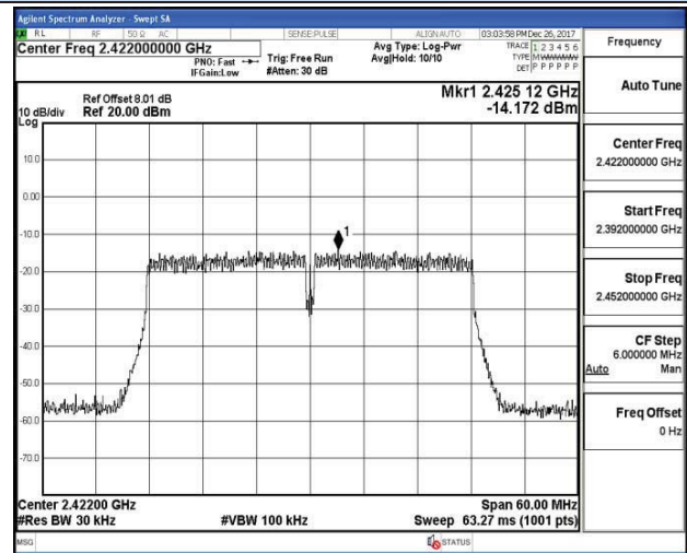
802.11n-HT40 Chain 1-Low channel
