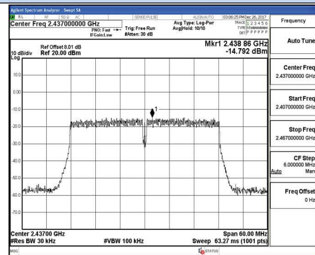
802.11n-HT40 Chain 1-Middle channel
