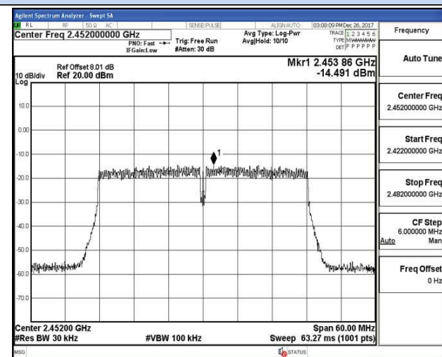
802.11n-HT40 Chain 1-High channel
