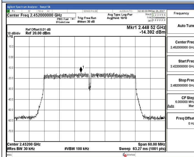
802.11n-HT40 Chain 0-High channel
