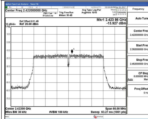
802.11n-HT40 Chain 0-Low channel
