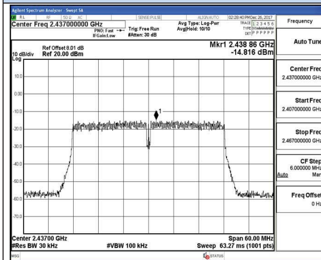
802.11n-HT40 Chain 0-Middle channel
