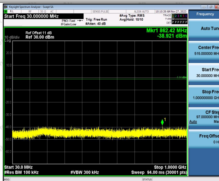
2.4G_Ant1_2440.8_30~1000
