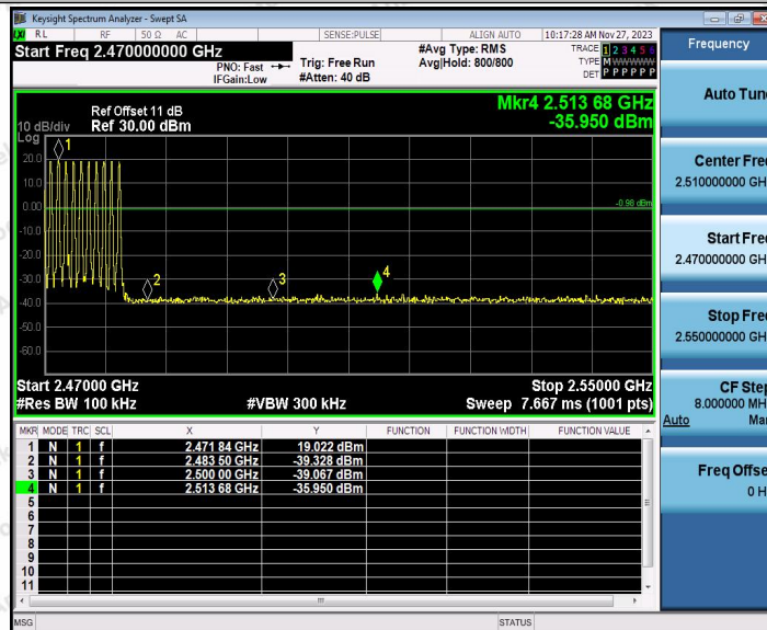
2.4G_Ant1_High_Hop_2479.8
