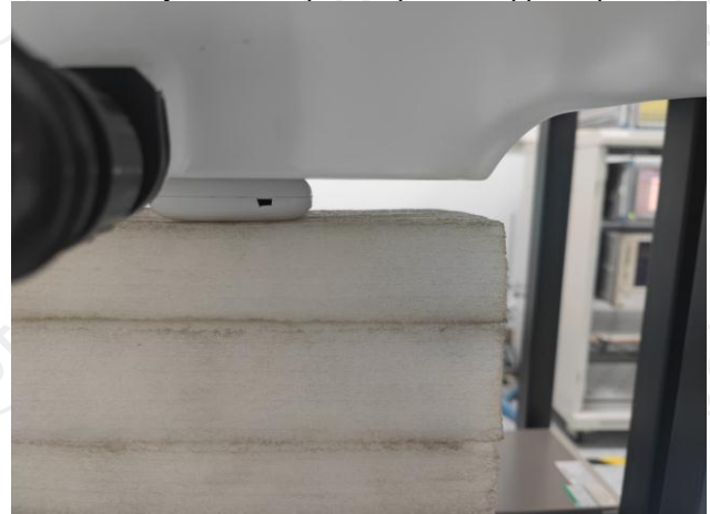
Body worn –vertical(External) (0mm)
