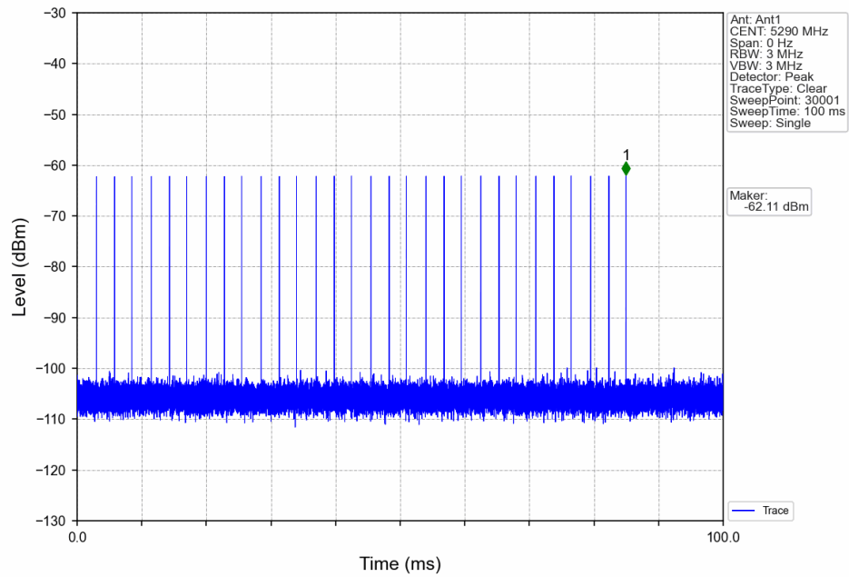
Signal Calibration_802.11 ac_2A_5290MHz_RadarType5_Trial0
