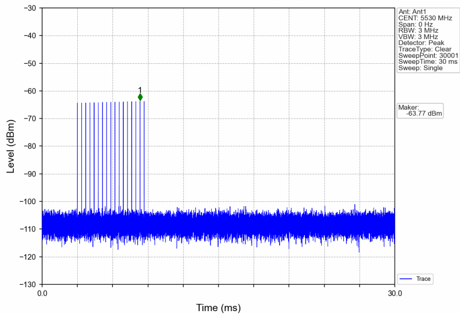
Signal Calibration_802.11 ac_2C_5530MHz_RadarType3_Trial0
