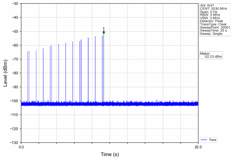
Signal Calibration_802.11 ac_2C_5530MHz_RadarType5_Trial0
