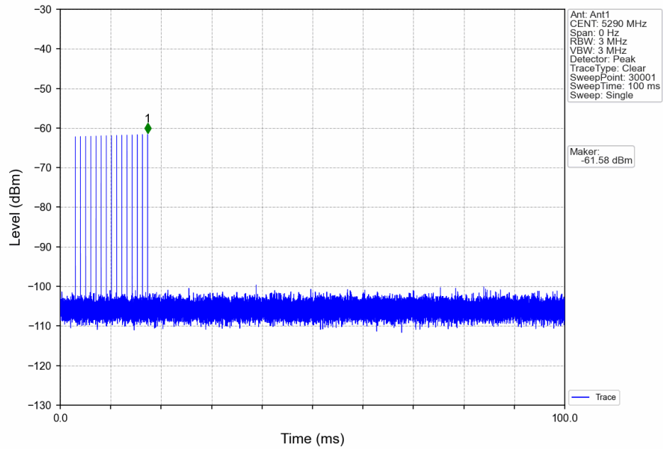
Signal Calibration_802.11 ac_2A_5290MHz_RadarType3_Trial0
