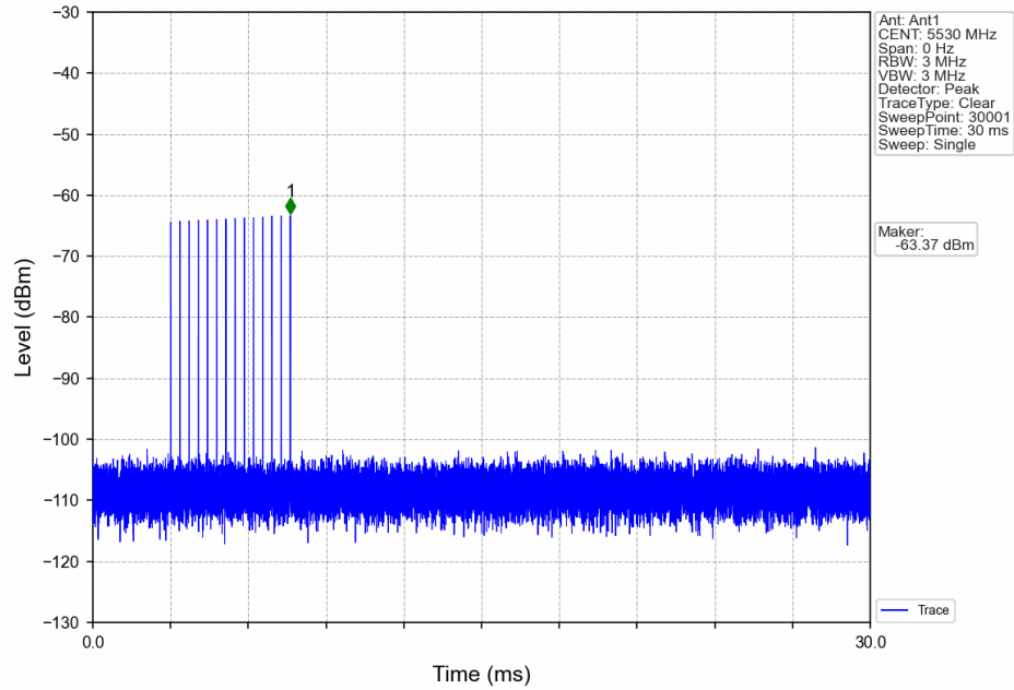
Signal Calibration_802.11 ac_2C_5530MHz_RadarType5_Trial0
