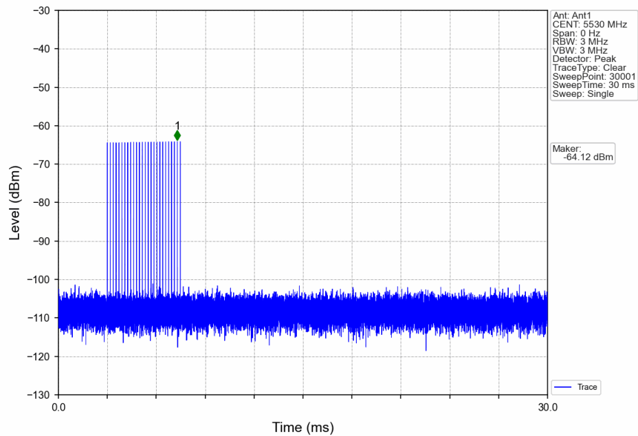
Signal Calibration_802.11 ac_2C_5530MHz_RadarType3_Trial0
