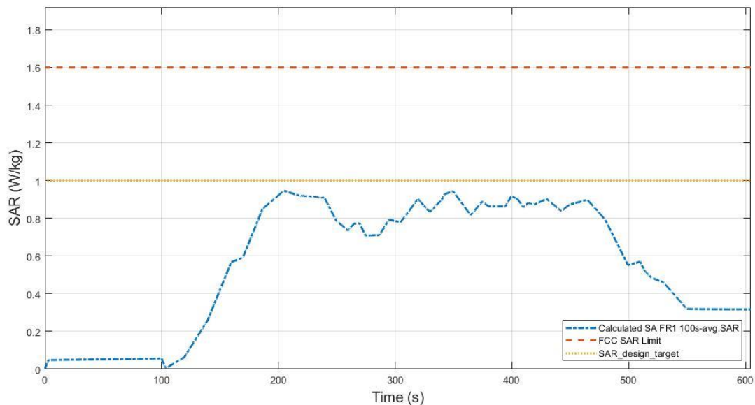
Figure 7.3-22 Total time-averaged SAR in TC04
