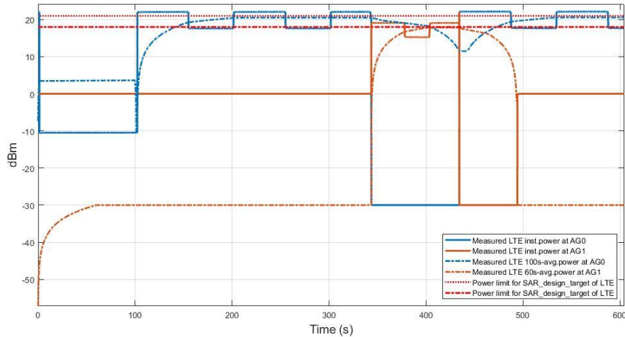
Figure 7.11-1 Conducted Transmitted power for LTE Band 7 and LTE band 48 in Test TC12
