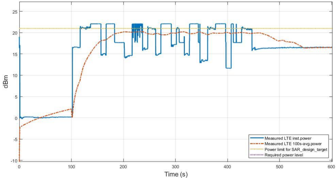
Figure 7.3-13 Conducted Tx power of LTE B7 in TC03
