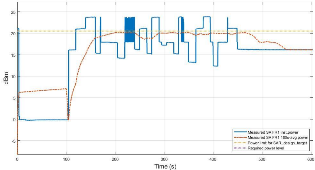
Figure 7.3-19 Conducted Tx power for SA FR1 n25 in TC04
