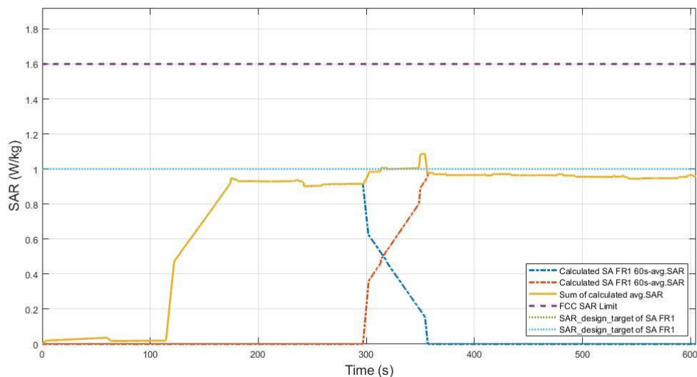
Figure 7.7-2 Total time-averaged SAR FR1 n77 in TC8
