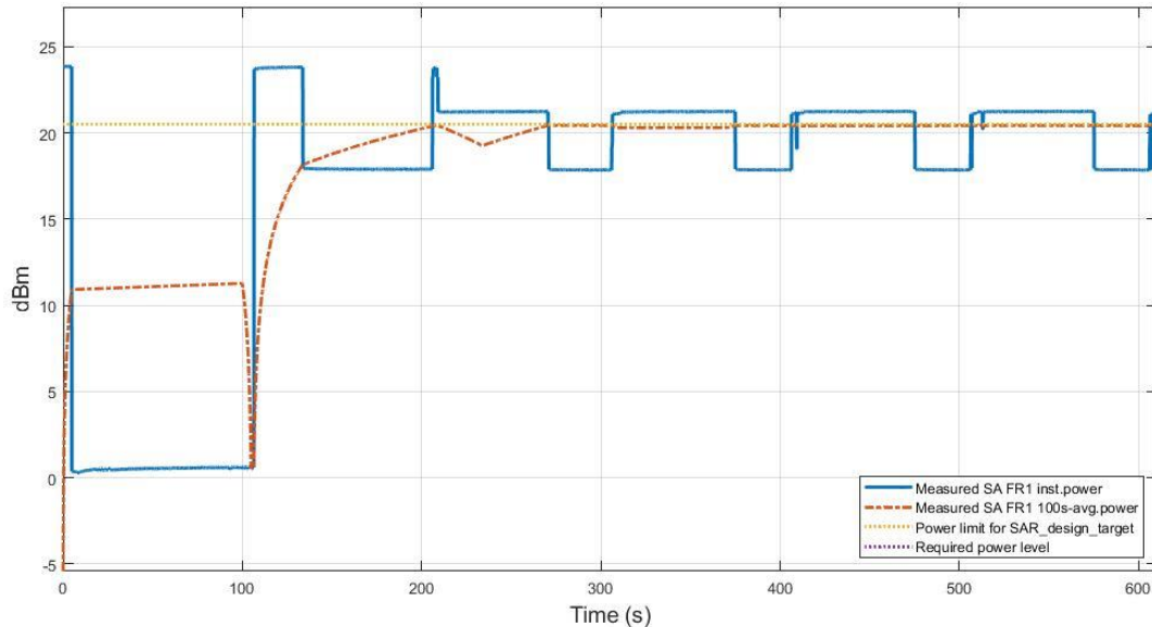
Figure 7.3-7 Time-average conducted power of SA FR1 n25 in TC02
