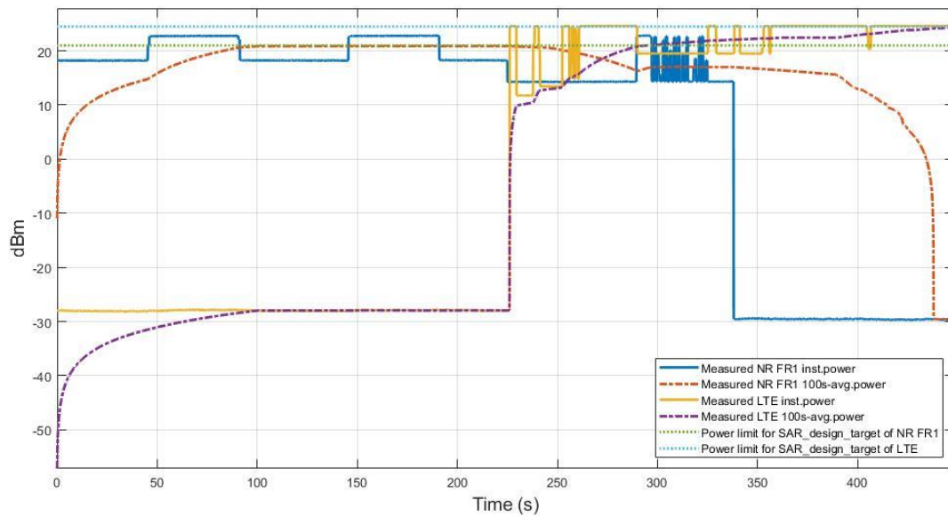
Figure 7.6-3 Time average SAR of LTE Band 12 and FR1 n41 EN-DC case
