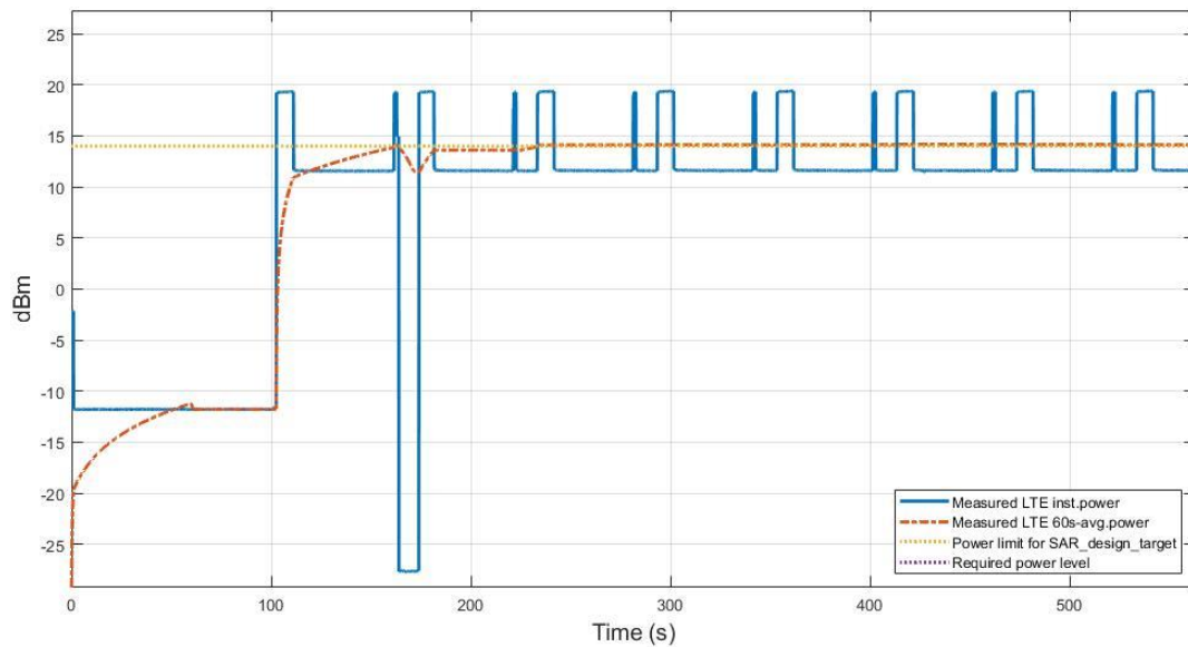
Figure 7.4-5 Conducted Tx power in Call_Disconnect_Re-establishment LTE Band 48 case TC05
