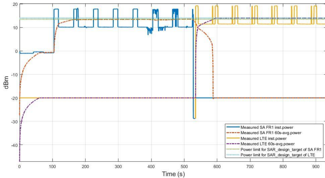
Figure 7.5-5 Conducted Tx power for SAR IRAT re-selection in test TC06 [n48 to LTE Band 48]
