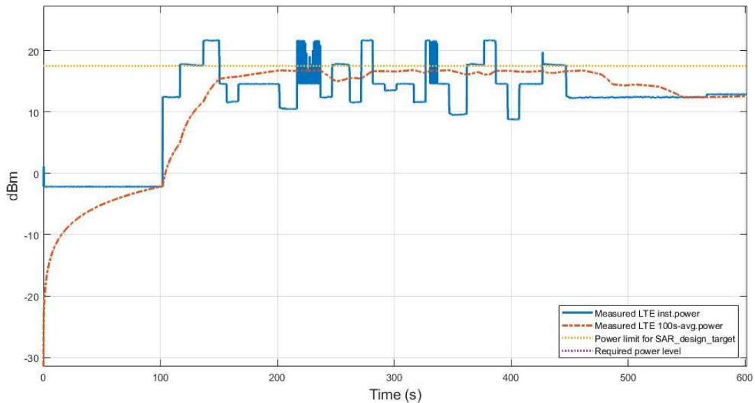
Figure 7.3-15 Conducted Tx power of LTE B41 in TC03
