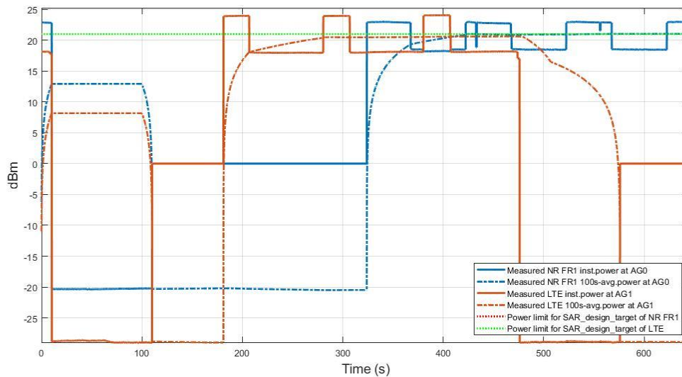
Figure 7.12-3 Conducted Transmitted power for LTE Band 66 and NR band n41 in Test TC13
