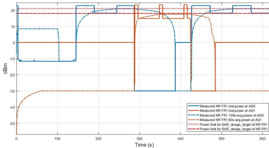
Figure 7.11-3 Conducted Transmitted power for NR Band 41 and NR band 77 in Test TC12
