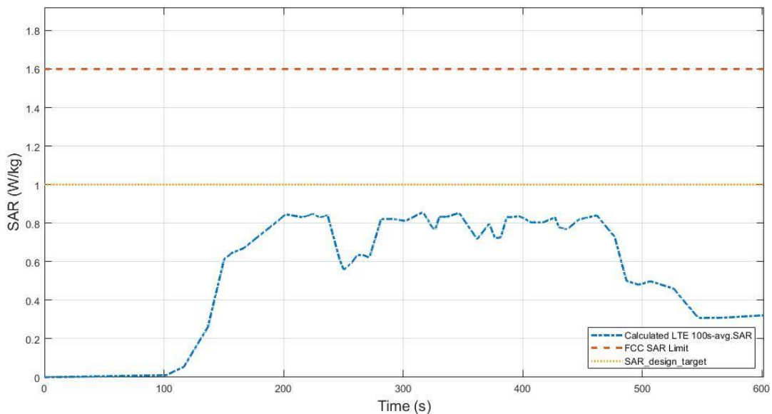
Figure 7.3-16 Total time-averaged SAR in TC03
