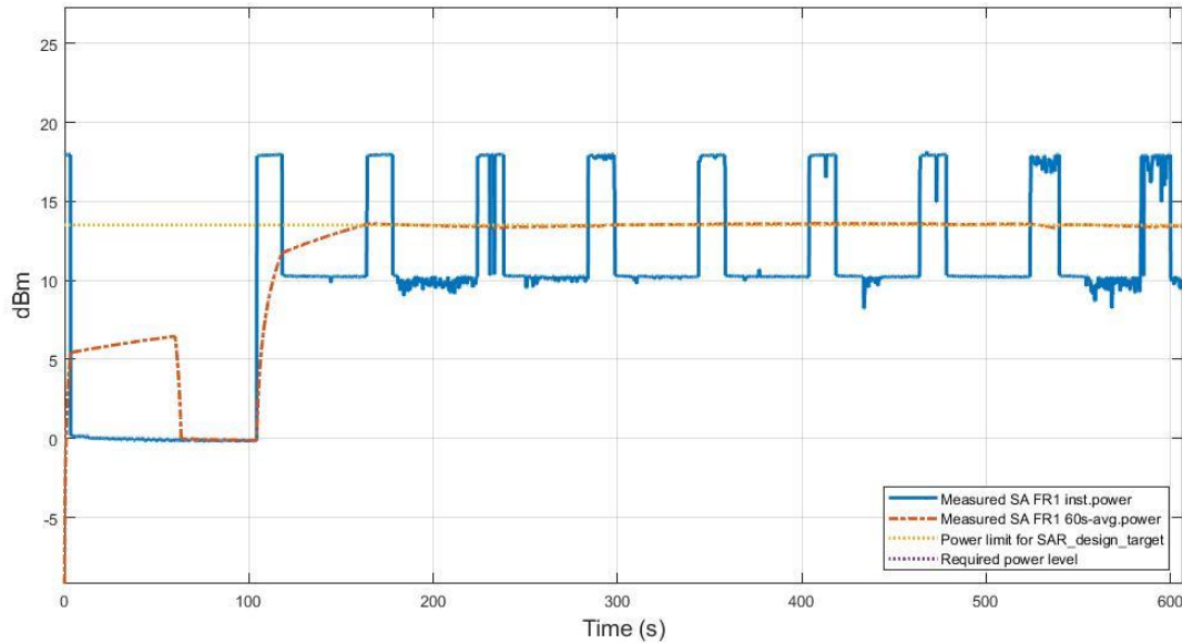
Figure 7.3-11 Time-average conducted power of SA FR1 n48 in TC02
