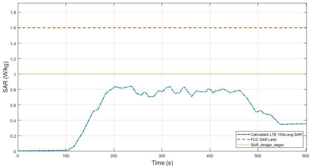
Figure 7.3-14 Total time-averaged SAR in TC03
