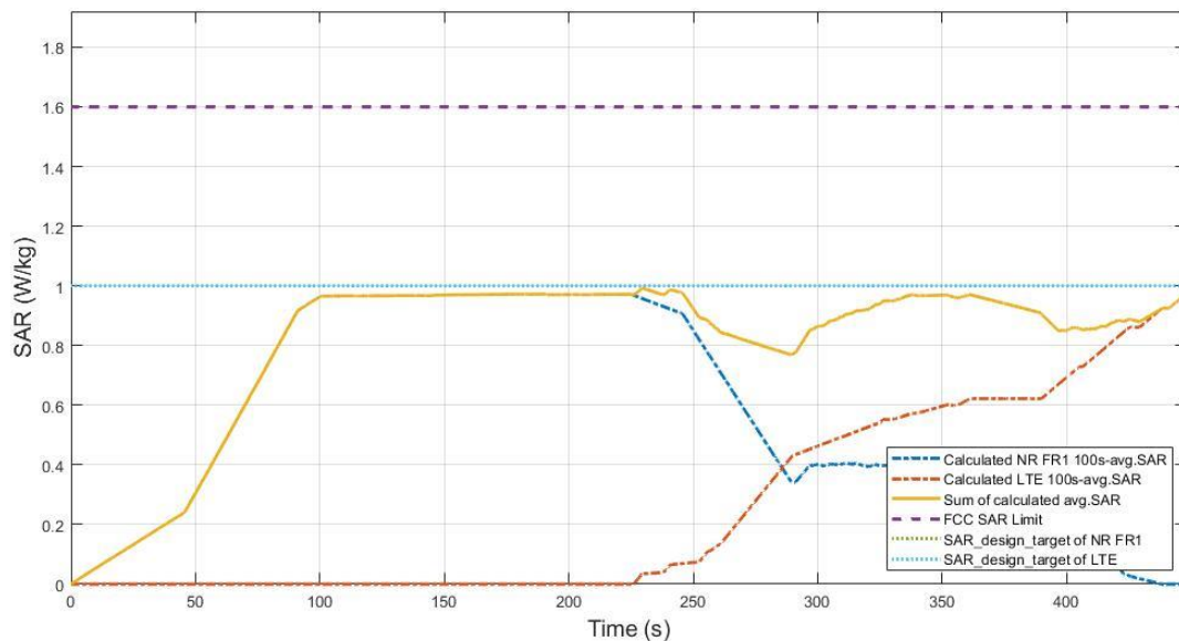
Figure 7.6-4 Total time-averaged SAR in TC07
