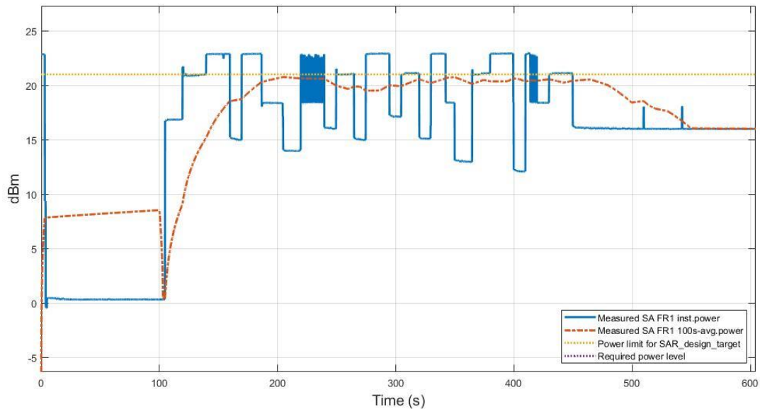
Figure 7.3-21 Conducted Tx power for SA FR1 n41 in TC04
