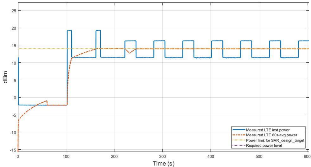
Figure 7.3-5 Time average conducted power of LTE B48 in TC01
