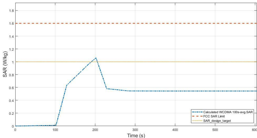
Figure 7.9-2 Total time-averaged SAR in TC10-1
