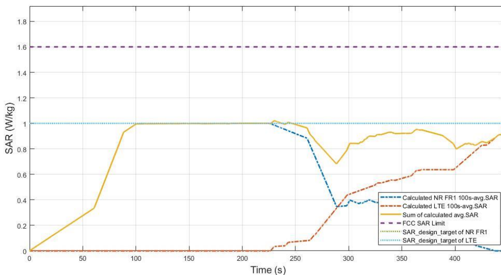
Figure 7.6-2 Total time-averaged SAR in TC07
