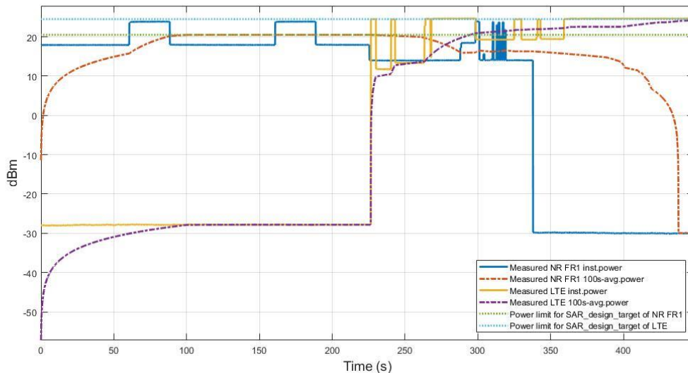
Figure 7.6-1 Time average SAR of LTE Band 12 and FR1 n25 EN-DC case
