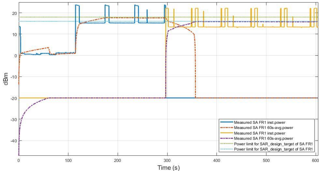
Figure 7.7-1 Conducted Tx power for SAR RSI Change FR1 n77 in test TC8
