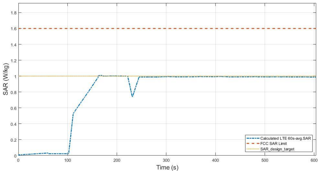
Figure 7.3-6 Total time-averaged SAR in TC01
