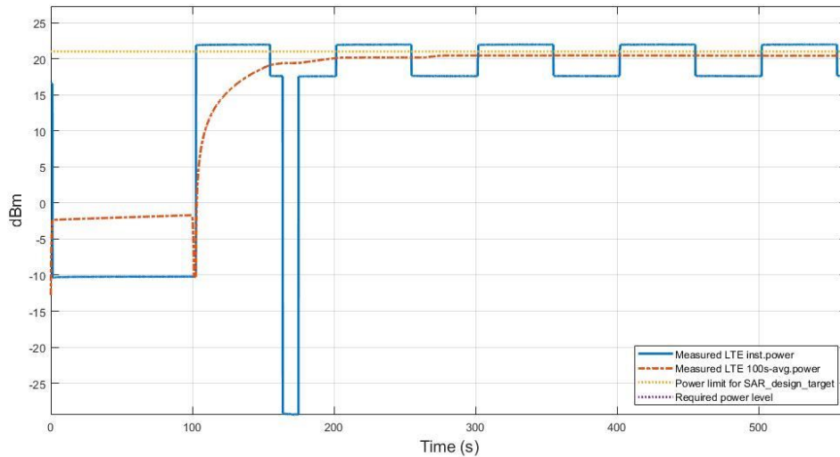
Figure 7.4-1 Conducted Tx power in Call_Disconnect_Reestablishment LTE Band 7 case TC05
