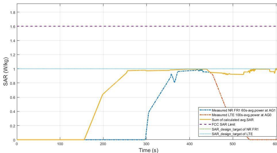
Figure 7.12-2 Total time-averaged SAR in TC13
