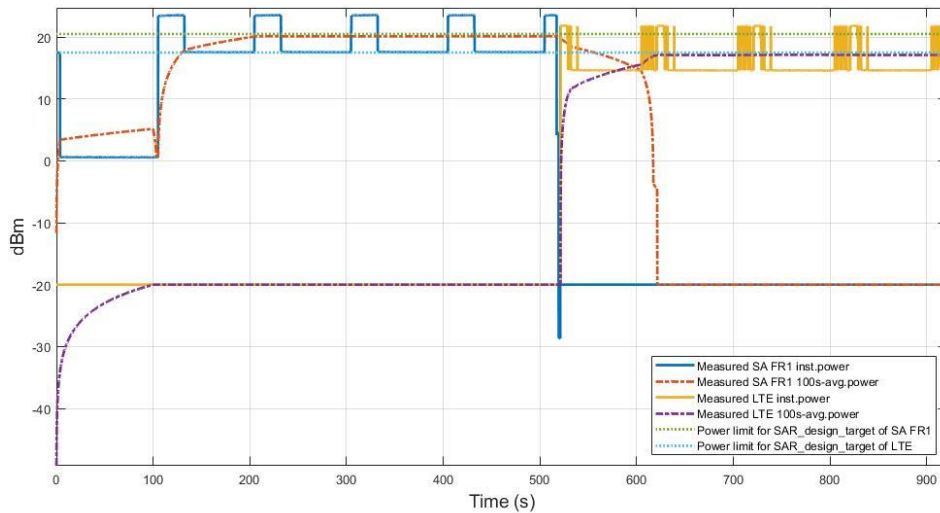
Figure 7.5-1 Conducted Tx power for SAR IRAT re-selection in test TC06 [n25 to LTE Band 41]
