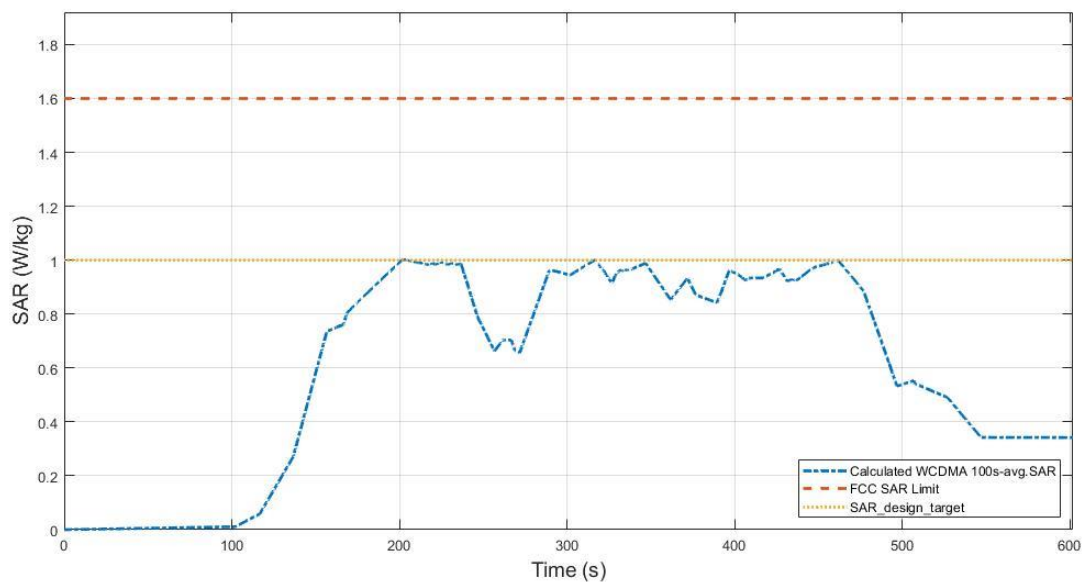
Figure 7.9-2 Total time-averaged SAR in TC10-2
