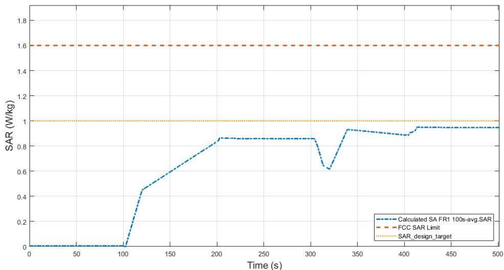
Figure 7.8-2 Total time-averaged SAR in TC9
