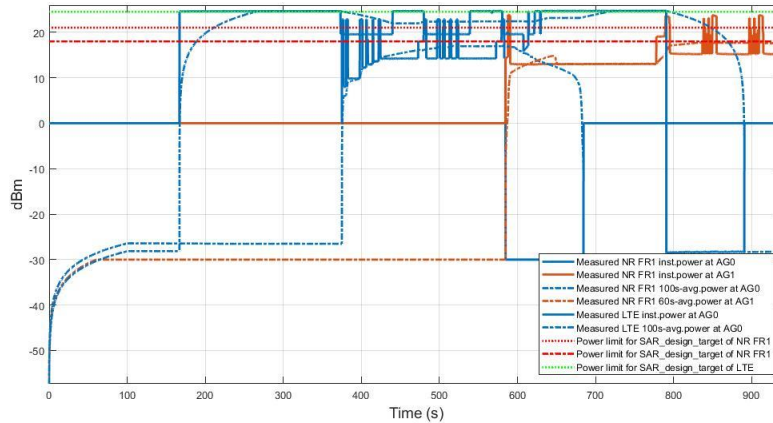
Figure 7.13-1 Conducted Transmitted power for LTE Band 12 and NR band n41, n77 in Test TC14
