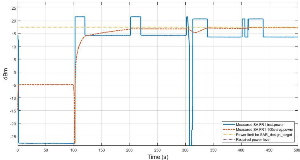
Figure 7.8-1 Conducted Transmitted Power of test TC9 [LTE Band 41]
