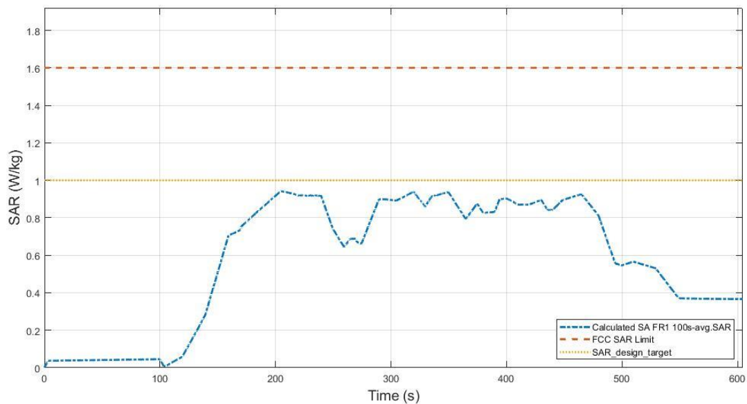
Figure 7.3-20 Total time-averaged SAR in TC04
