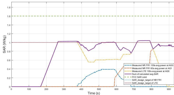
Figure 7.13-2 Total time-averaged SAR in TC14
