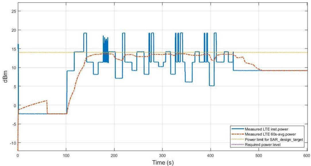
Figure 7.3-17 Conducted Tx power of LTE B48 in TC03
