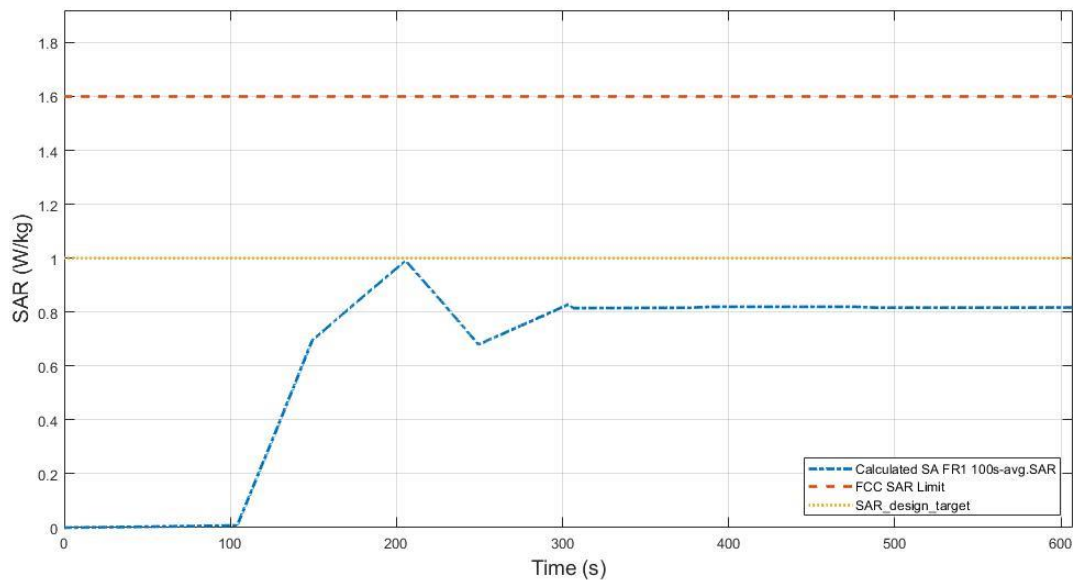
Figure 7.3-10 Total time-averaged SAR in TC02
