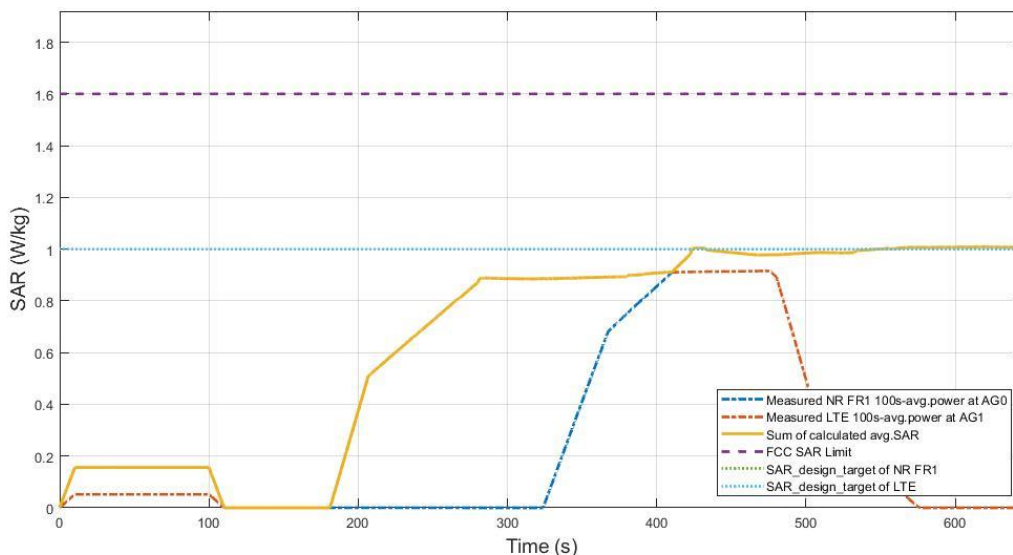
Figure 7.12-4 Total time-averaged SAR in TC13
