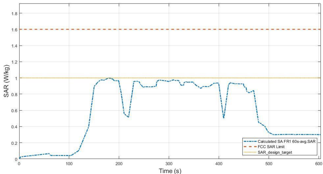
Figure 7.3-24 Total time-averaged SAR in TC04
