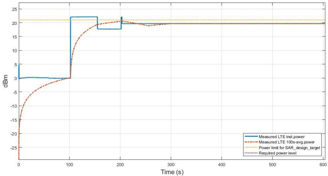
Figure 7.3-1 Time average conducted power of LTE B7 in TC01
