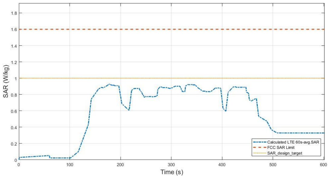
Figure 7.3-18 Total time-averaged SAR in TC03
