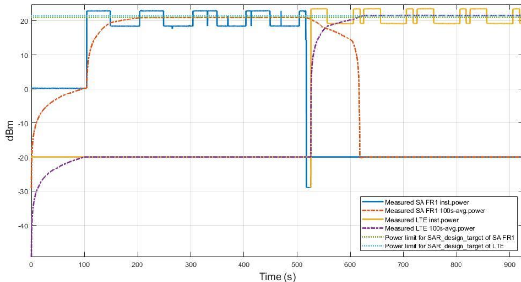
Figure 7.5-3 Conducted Tx power for SAR IRAT re-selection in test TC06 [n41 to LTE Band 66]
