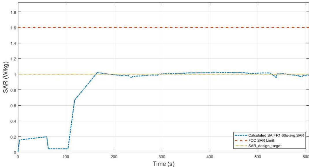
Figure 7.3-12 Total time-averaged SAR in TC02
