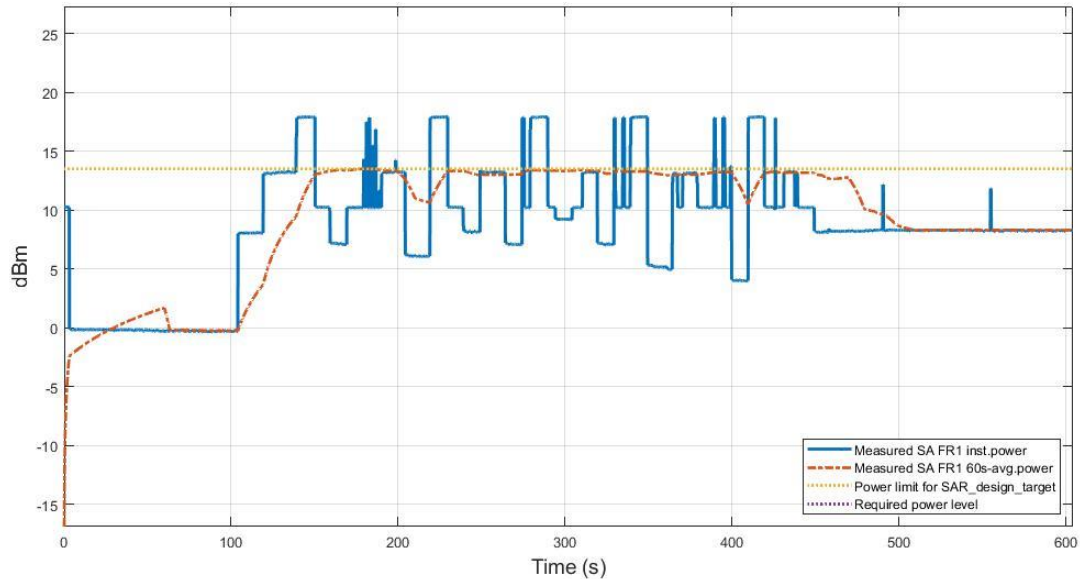
Figure 7.3-23 Conducted Tx power for SA FR1 n48 in TC04
