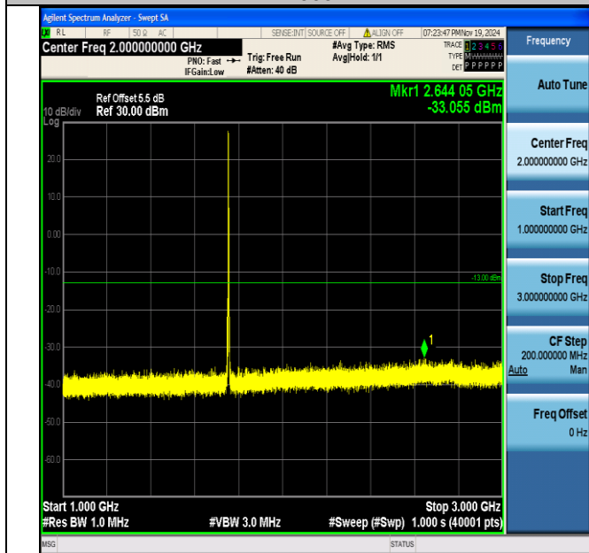
Band4_3MHz_16QAM_20385_1RB#0_1000~3000_1000~3000
