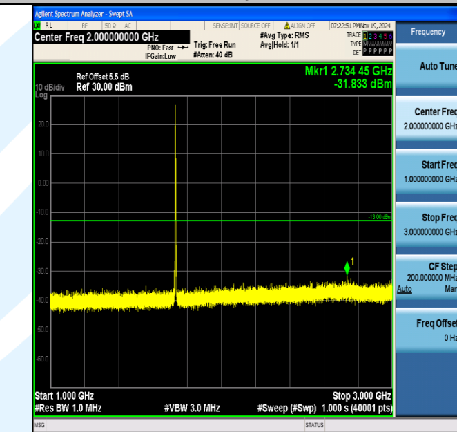
Band4_3MHz_16QAM_20175_1RB#0_1000~3000_1000~3000
