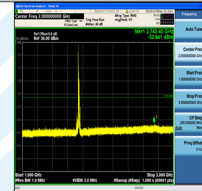
Band4_15MHz_QPSK_20325_1RB#0_1000~3000_1000~3000
