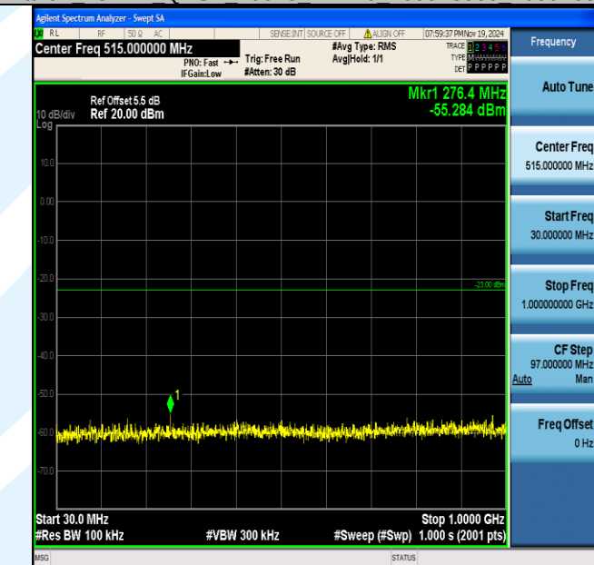
Band4_15MHz_QPSK_20175_1RB#0_30~1000_30~1000
