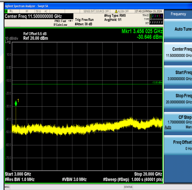
Band4_10MHz_QPSK_20175_1RB#0_3000~20000_3000~20000
