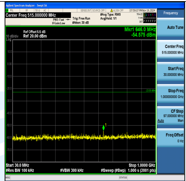
Band4_15MHz_16QAM_20025_1RB#0_30~1000_30~1000
