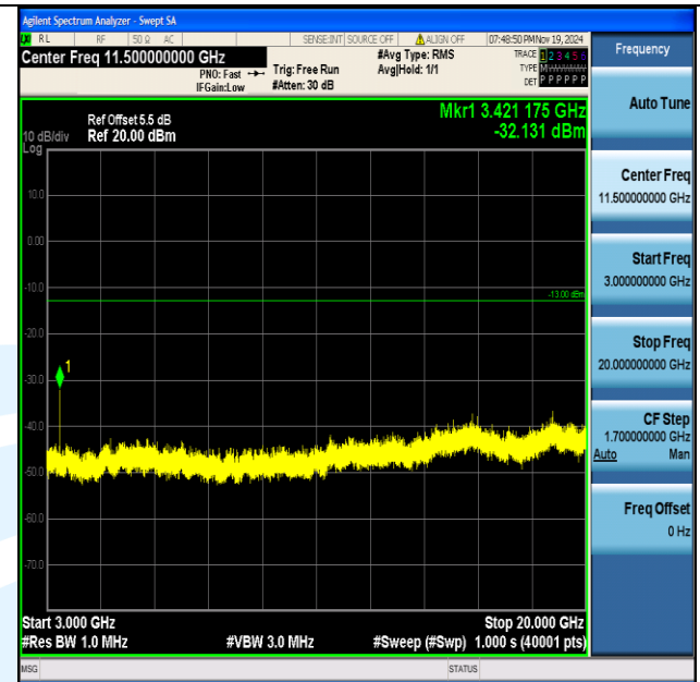
Band4_10MHz_16QAM_20000_1RB#0_3000~20000_3000~2000
