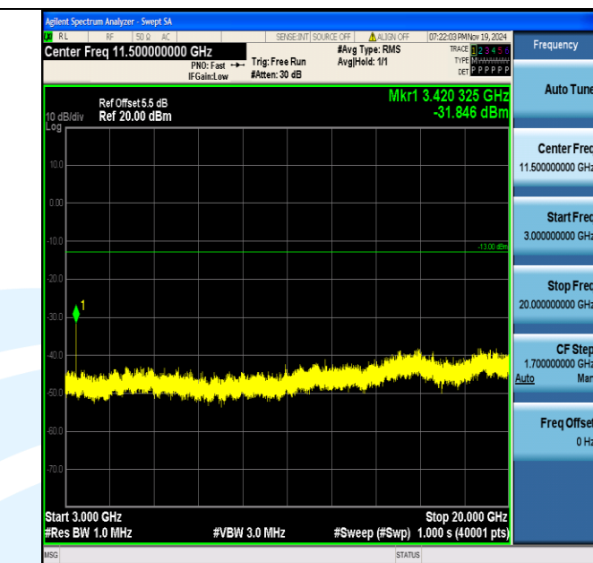
Band4_3MHz_16QAM_19965_1RB#0_3000~20000_3000~20000
