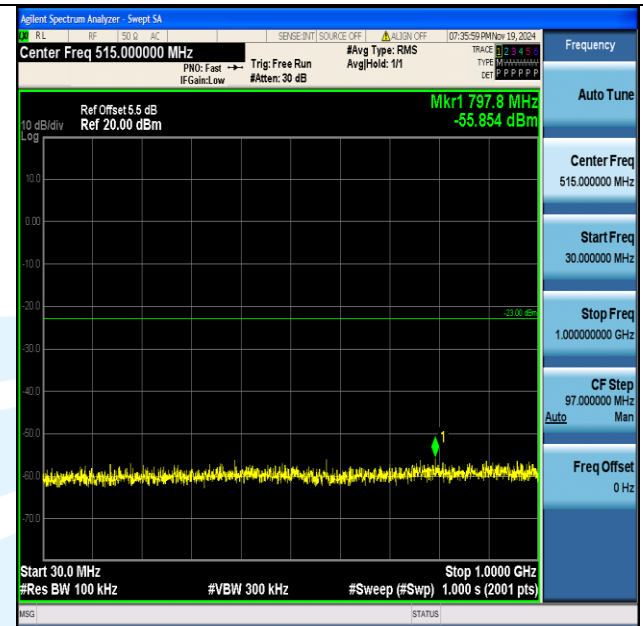
Band4_5MHz_16QAM_19975_1RB#0_30~1000_30~1000
