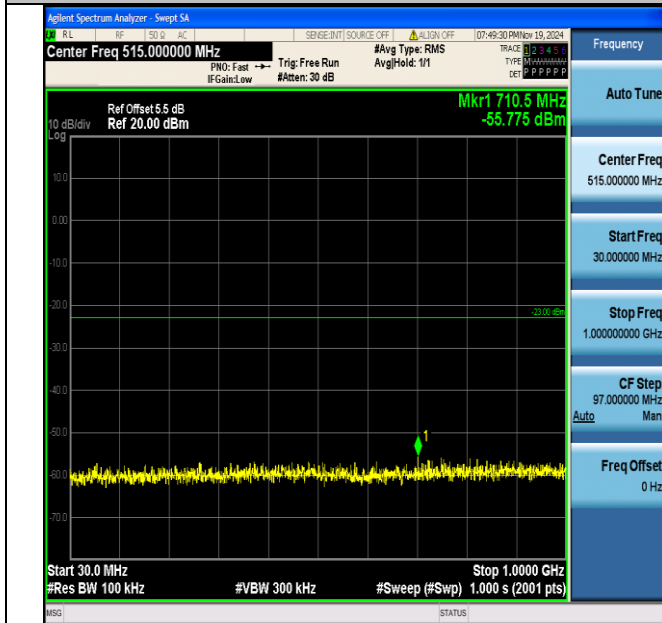
Band4_10MHz_16QAM_20175_1RB#0_30~1000_30~1000
