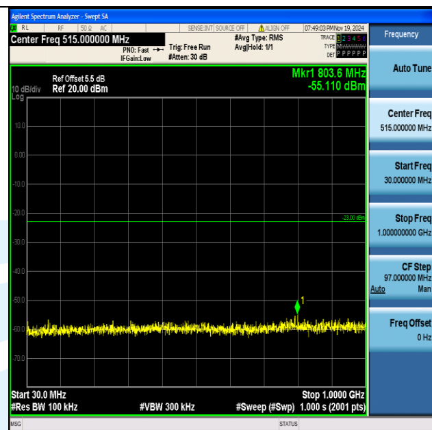
Band4_10MHz_QPSK_20175_1RB#0_30~1000_30~1000
