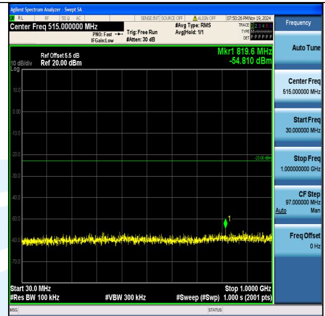
Band4_10MHz_16QAM_20350_1RB#0_30~1000_30~1000
