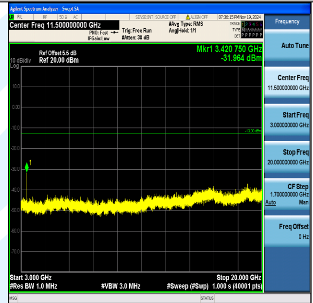
Band4_5MHz_16QAM_19975_1RB#0_3000~20000_3000~20000
