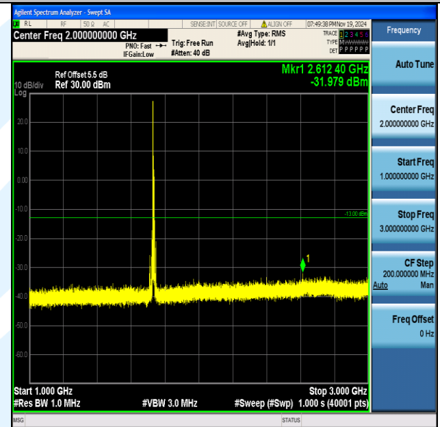
Band4_10MHz_16QAM_20175_1RB#0_1000~3000_1000~3000
