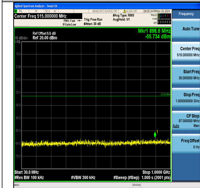
Band4_15MHz_QPSK_20325_1RB#0_30~1000_30~1000
