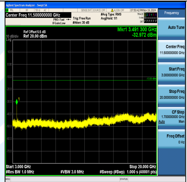
Band4_10MHz_16QAM_20350_1RB#0_3000~20000_3000~20000
