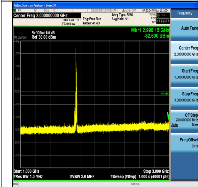
Band4_10MHz_16QAM_20350_1RB#0_1000~3000_1000~3000
