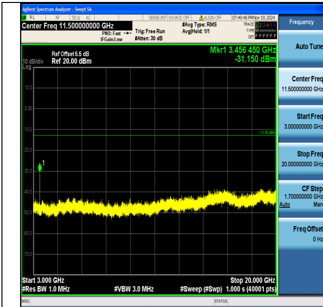
Band4_10MHz_16QAM_20175_1RB#0_3000~20000_3000~20000
