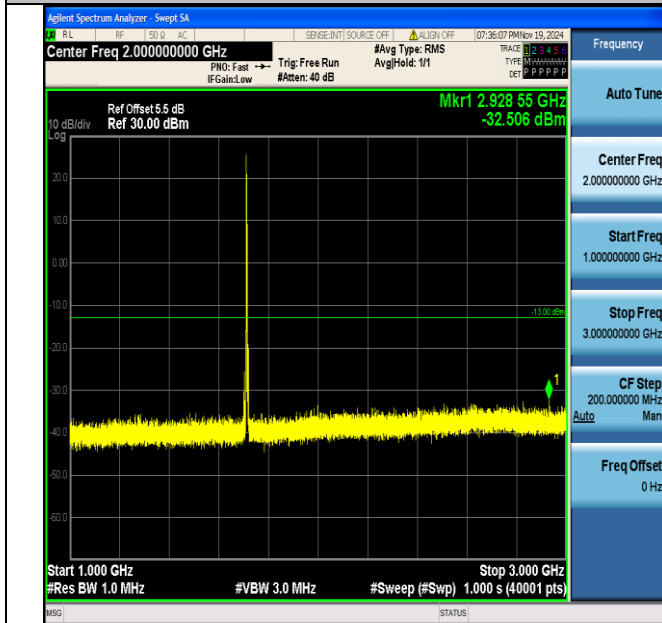
Band4_5MHz_16QAM_19975_1RB#0_1000~3000_1000~3000
