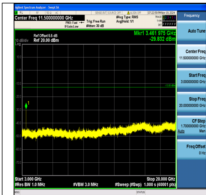
Band4_3MHz_16QAM_20175_1RB#0_3000~20000_3000~20000
