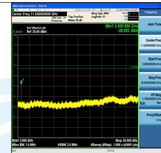
Band4_5MHz_16QAM_20375_1RB#0_3000~20000_3000~20000
