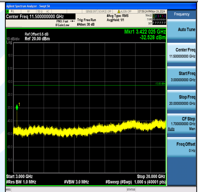
Band4_15MHz_16QAM_20025_1RB#0_3000~20000_3000~20000
