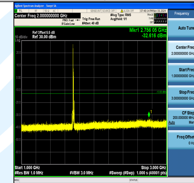
Band4_10MHz_QPSK_20000_1RB#0_1000~3000_1000~3000
