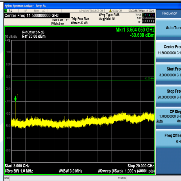
Band4_3MHz_16QAM_20385_1RB#0_3000~20000_3000~20000
