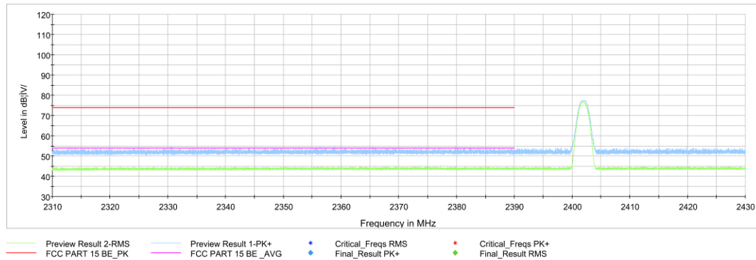
Fig.18. Frequency Band Edges: GFSK, 2402 MHz, Hopping Off, 2.31 GHz – 2.43GHz
