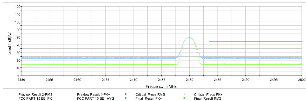
Fig.19. Frequency Band Edges: GFSK, 2480 MHz, Hopping Off, 2.45 GHz - 2.50GHz
