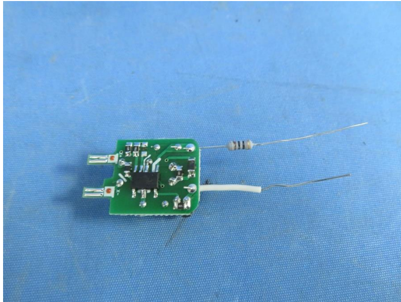
Photo 6 - Internal view
