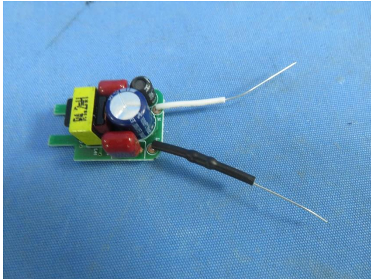
Photo 4 - Internal view
