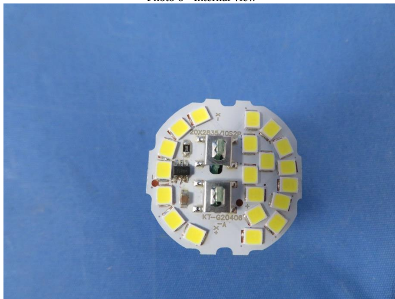
Photo 6 - Internal view
