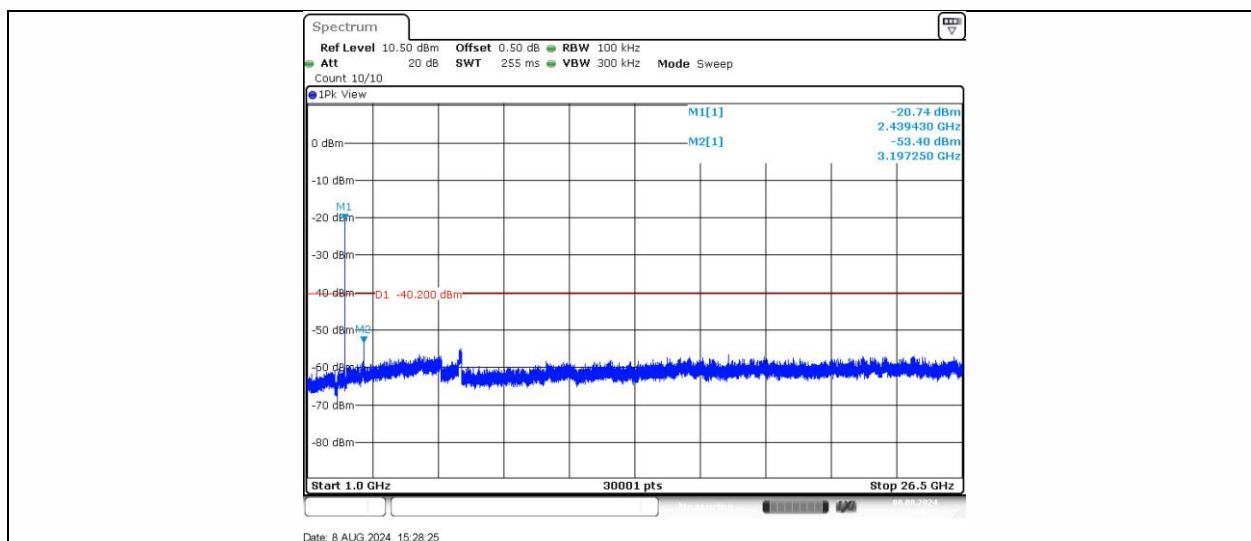
BLE_1M_Ant1_2440_1000~26500
