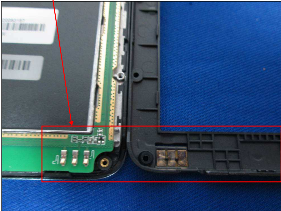
WWAN RX Diversity Antenna
