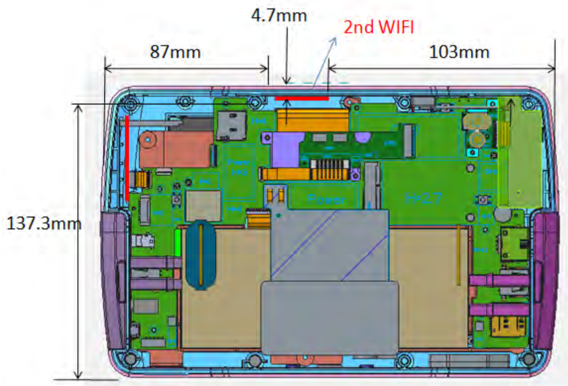
Fig.16 Antenna separation distance of EUT (WLAN Aux antenna)
