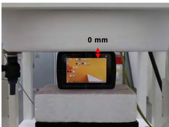
Fig.8 EUT Bottom side to flat phantom
