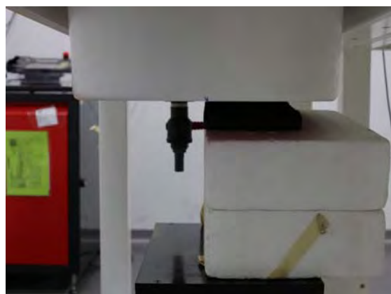
Fig.5 EUT Back side (Curve) to flat phantom (WWAN)
