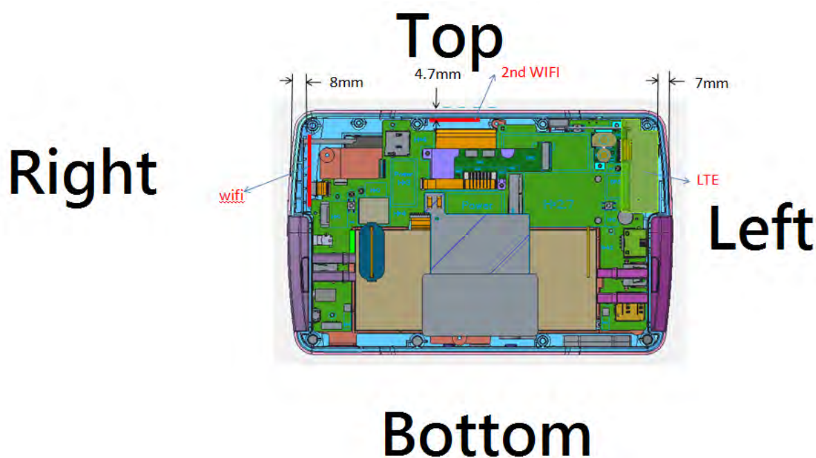
Fig.13 Antenna position of EUT (Back view)
