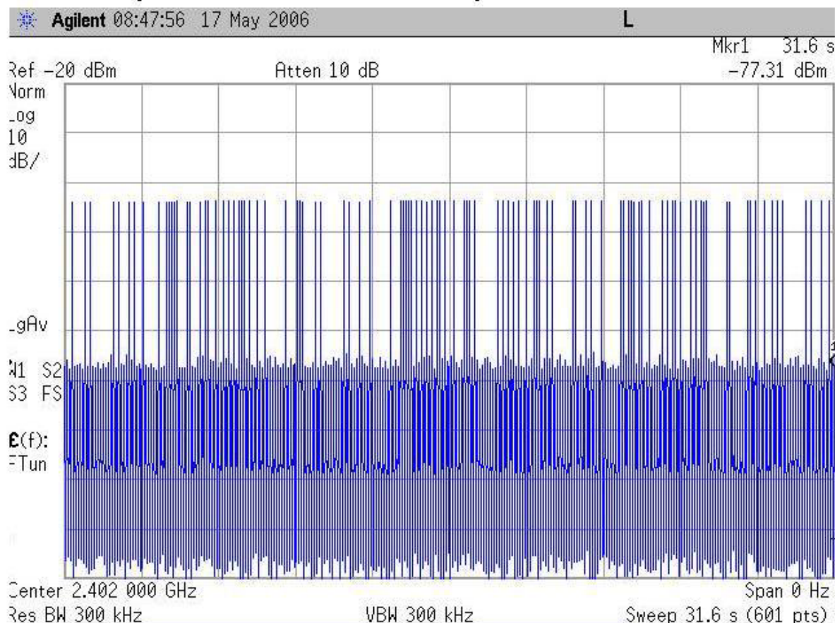
Figure 4-7: Time of Occupancy, 31.6 sec, DH5 Mode
