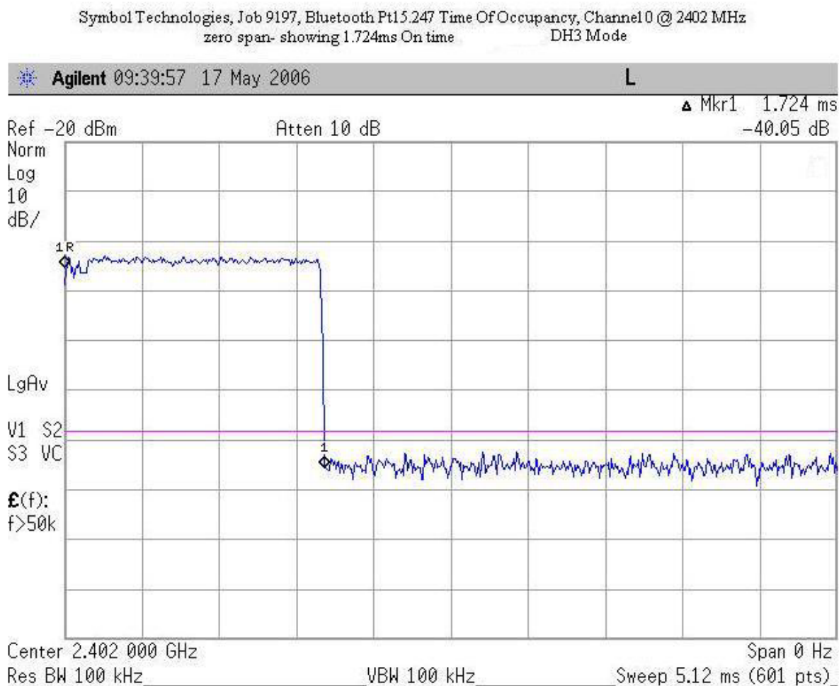
Figure 4-2. Duty Cycle Plot, Pulse Width, DH3 Mode
