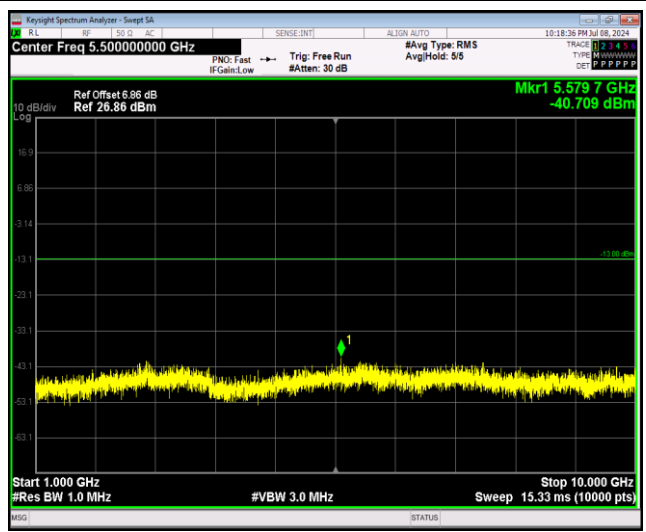
Band12-10MHz-64QAM-23095-1RB#0-Range2:1000~10000MHz
