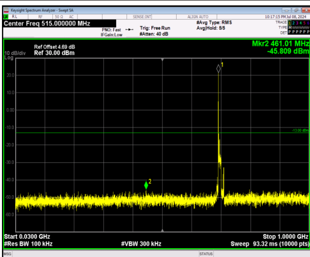
Band12-10MHz-16QAM-23095-1RB#0-Range1:30~1000MHz
