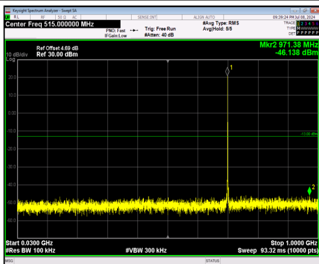
Band12-1.4MHz-64QAM-23173-1RB#0-Range1:30 ~1000MHz
