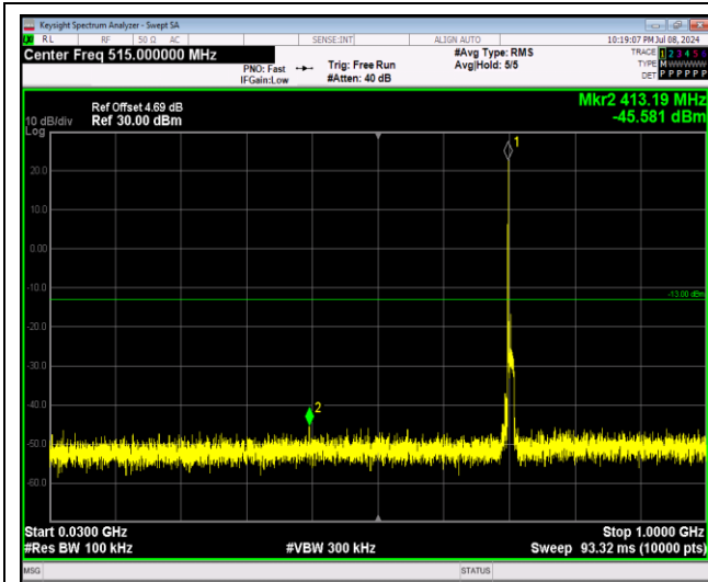
Band12-10MHz-64QAM-23060-1RB#0-Range1:30~1000MHz
