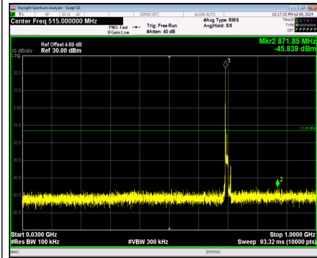
Band12-10MHz-64QAM-23095-1RB#0-Range1:30~1000MHz
