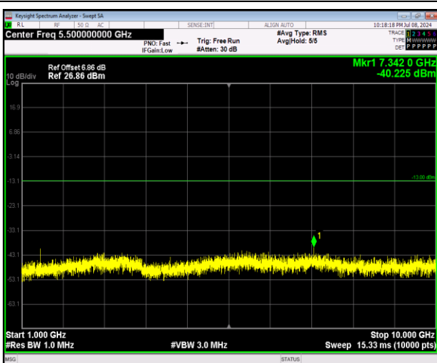
Band12-10MHz-16QAM-23130-1RB#0-Range2:1000~10000MHz
