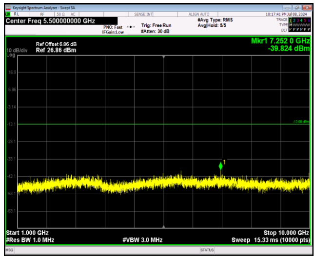
Band12-10MHz-64QAM-23095-1RB#0-Range2:1000~10000MHz
