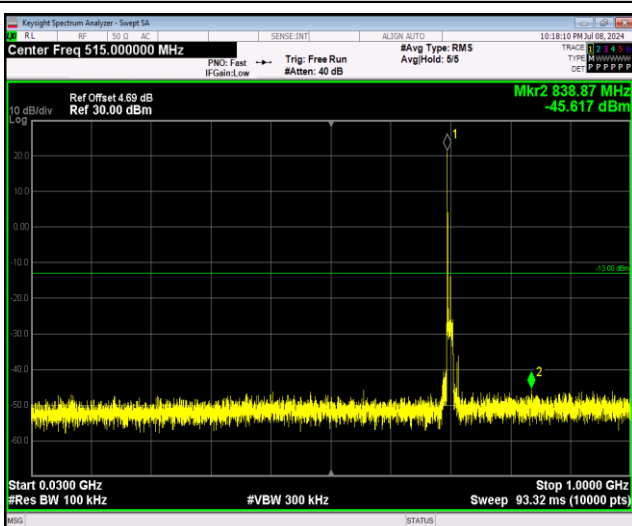
Band12-10MHz-16QAM-23130-1RB#0-Range1:30~1000MHz
