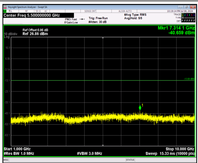
Band12-10MHz-64QAM-23060-1RB#0-Range2:1000~10000MHz
