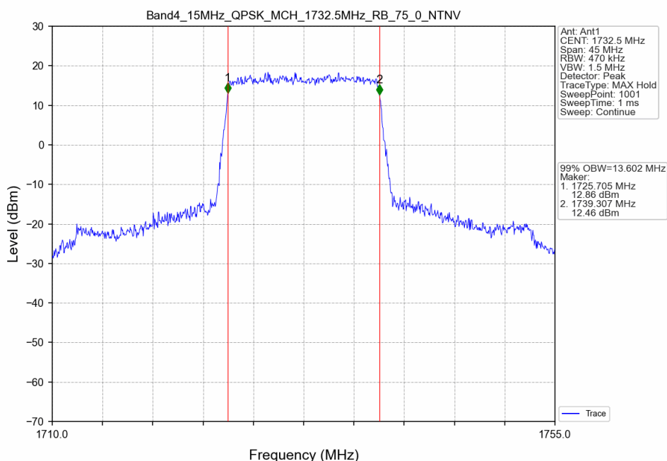
Band4_15MHz_QPSK_MCH_1732.5MHz_RB_75_0_NTNV
