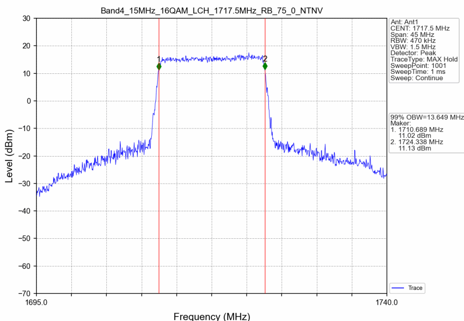
Band4_15MHz_16QAM_LCH_1717.5MHz_RB_75_0_NTNV
