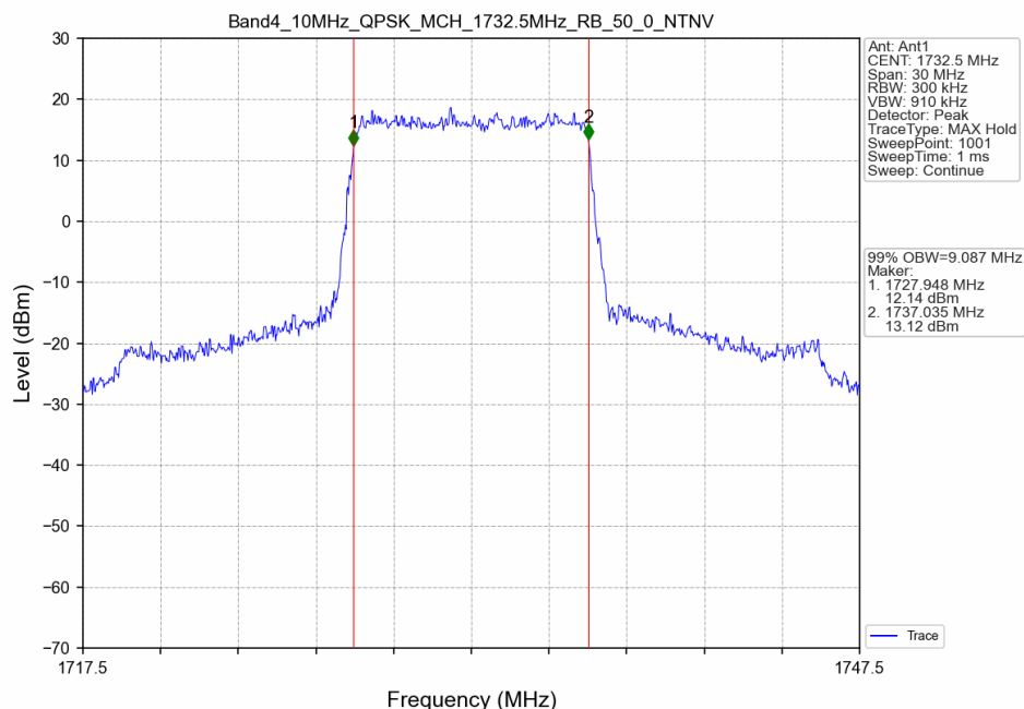
Band4_10MHz_QPSK_MCH_1732.5MHz_RB_50_0_NTNV
