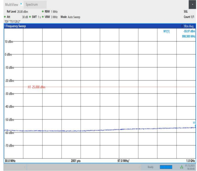
7-7-20MHz-10MHz-16QAM-16QAM-21051-21195-1RB#0-1RB #49-30~1000MHz-PASS
