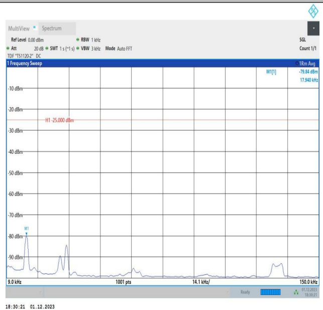
7-7-20MHz-10MHz-16QAM-16QAM-21051-21195-1RB#0-1RB #49-0.009~0.15MHz-PASS
