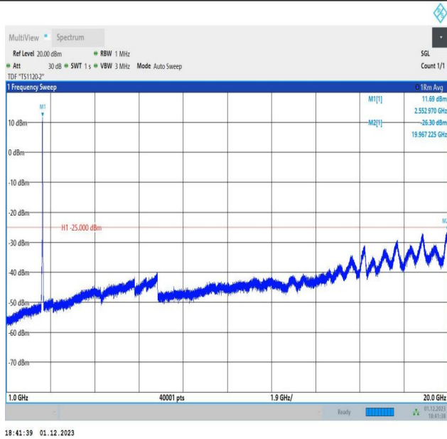
7-7-20MHz-10MHz-64QAM-64QAM-21251-21395-100RB#0-5 ORB#0-1000~20000MHz-PASS
