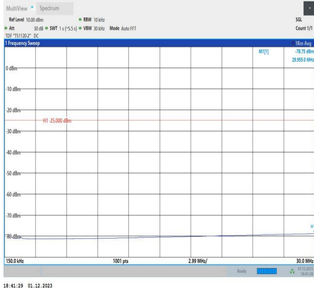
7-7-20MHz-10MHz-64QAM-64QAM-21251-21395-100RB#0-5 ORB#0-0.15~30MHz-PASS
