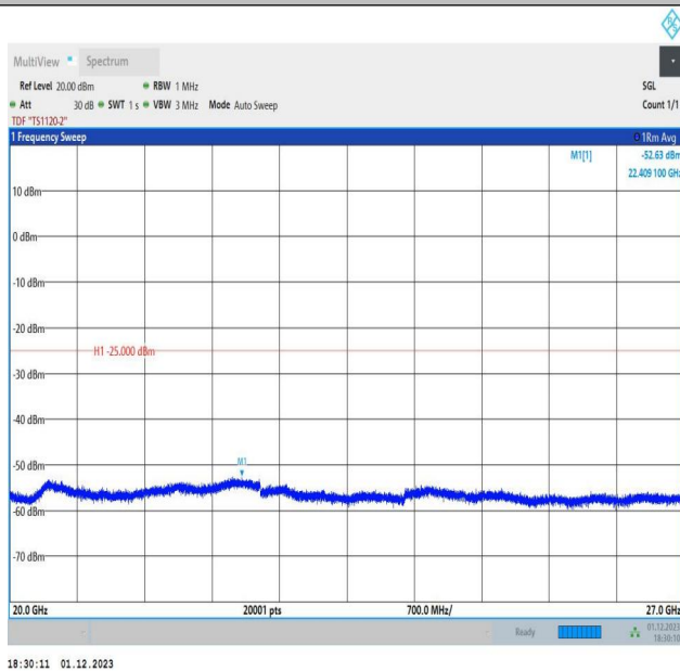
7-7-20MHz-10MHz-QPSK-QPSK-21051-21195-1RB#0-1RB#4 9-20000~27000MHz-PASS
