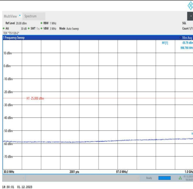
7-7-20MHz-10MHz-QPSK-QPSK-21051-21195-1RB#0-1RB#4 9-30~1000MHz-PASS
