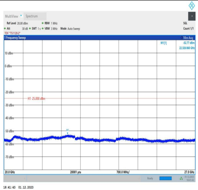
7-7-20MHz-10MHz-64QAM-64QAM-21251-21395-100RB#0-5 ORB#0-20000~27000MHz-PASS
