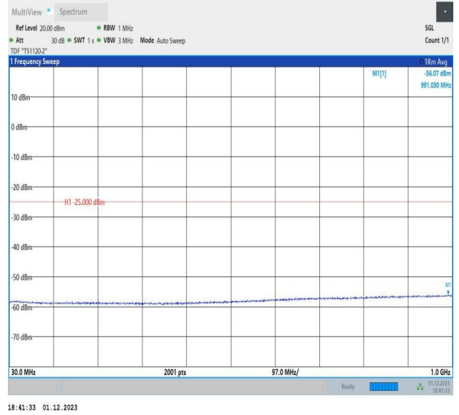
7-7-20MHz-10MHz-64QAM-64QAM-21251-21395-100RB#0-5 ORB#0-30~1000MHz-PASS
