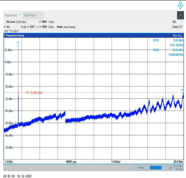
7-7-20MHz-10MHz-QPSK-QPSK-21051-21195-1RB#0-1RB#4 9-1000~20000MHz-PASS
