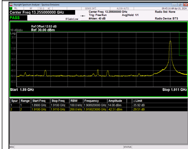
Band2_20MHz_64QAM_19100_1RB#99
