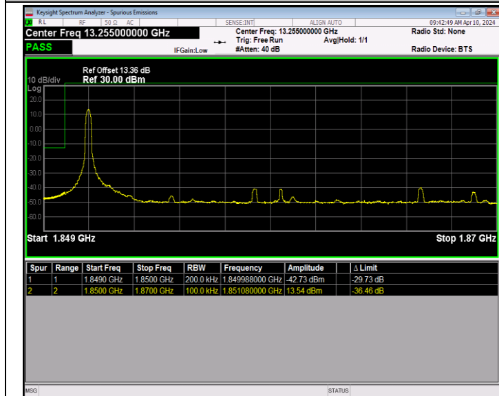
Band2_20MHz_64QAM_18700_1RB#0
