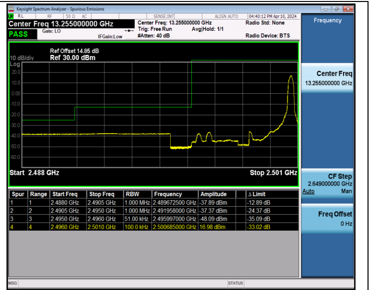
Band41_5MHz_QPSK_39675_1RB#24
