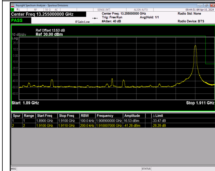
Band2_20MHz_QPSK_19100_1RB#99
