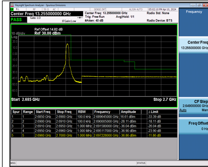
Band41_5MHz_QPSK_41565_1RB#24
