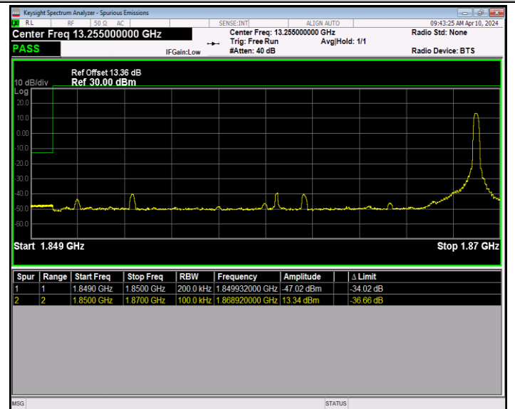
Band2_20MHz_64QAM_18700_1RB#99
