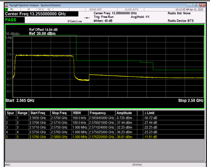
Band7_5MHz_16QAM_21425_25RB#0
