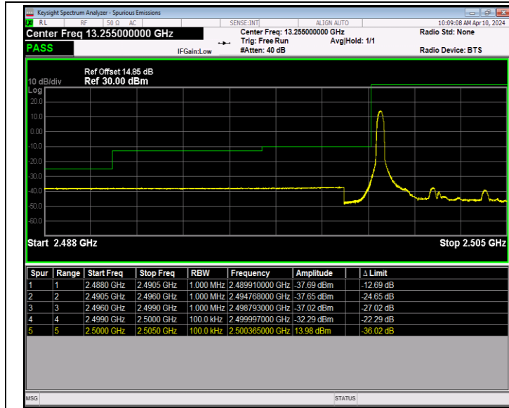
Band7_5MHz_64QAM_20775_1RB#0
