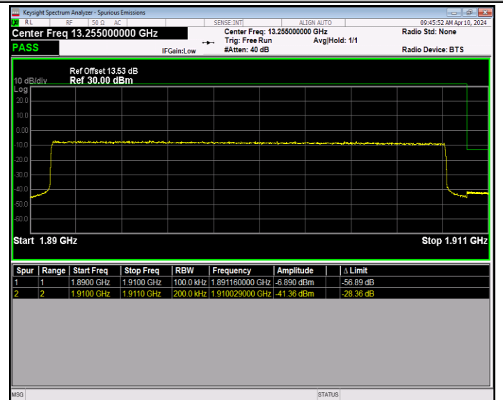
Band2_20MHz_64QAM_19100_100RB#0
