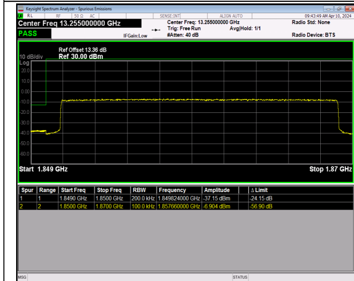
Band2_20MHz_16QAM_18700_100RB#0
