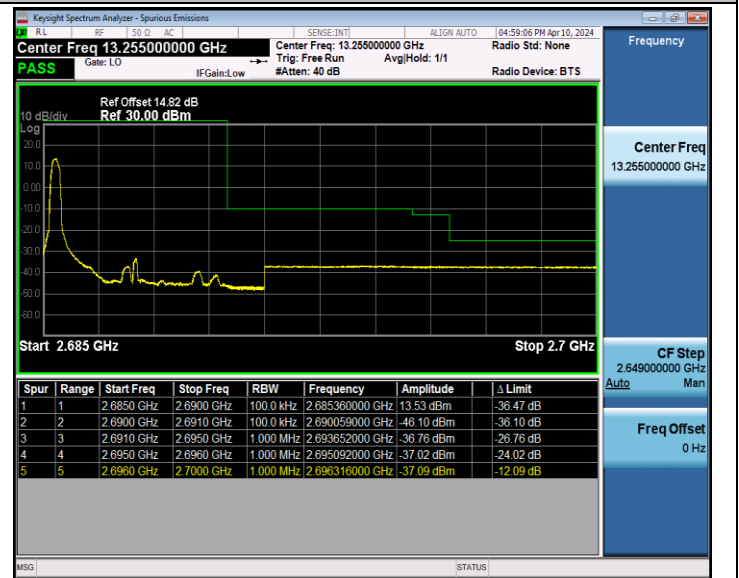
Band41_5MHz_64QAM_41565_1RB#0
