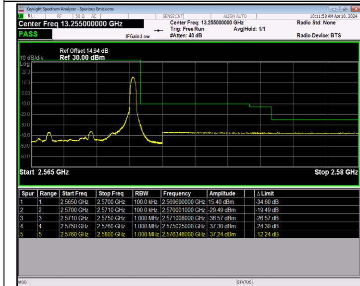
Band7_5MHz_16QAM_21425_1RB#24
