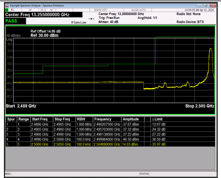
Band7_5MHz_64QAM_20775_1RB#24
