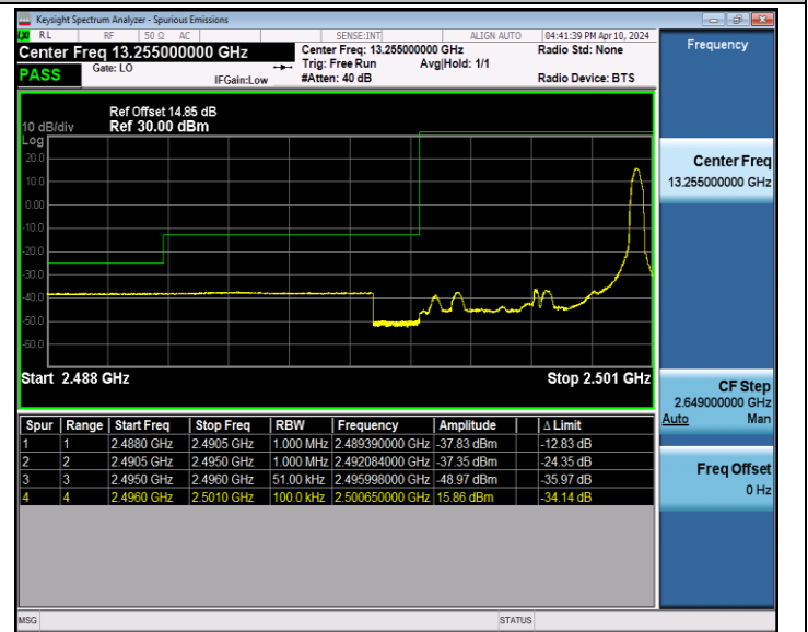
Band41_5MHz_16QAM_39675_1RB#24
