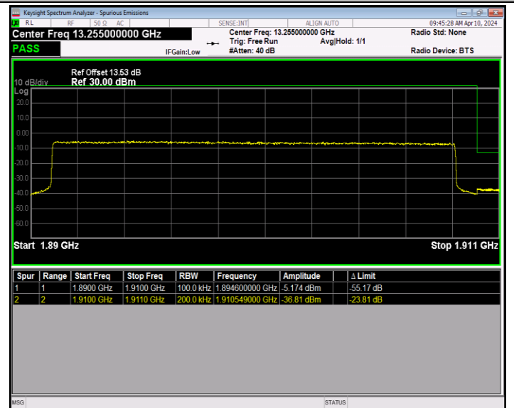
Band2_20MHz_QPSK_19100_100RB#0
