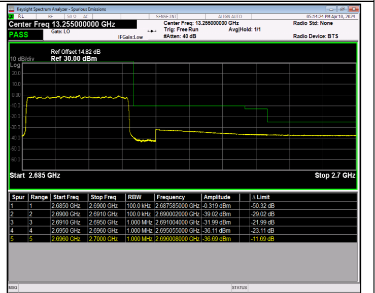
Band41_5MHz_16QAM_41565_25RB#0
