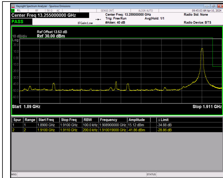
Band2_20MHz_16QAM_19100_1RB#99
