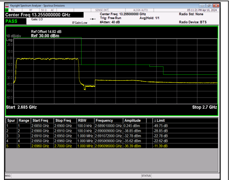
Band41_5MHz_QPSK_41565_25RB#0
