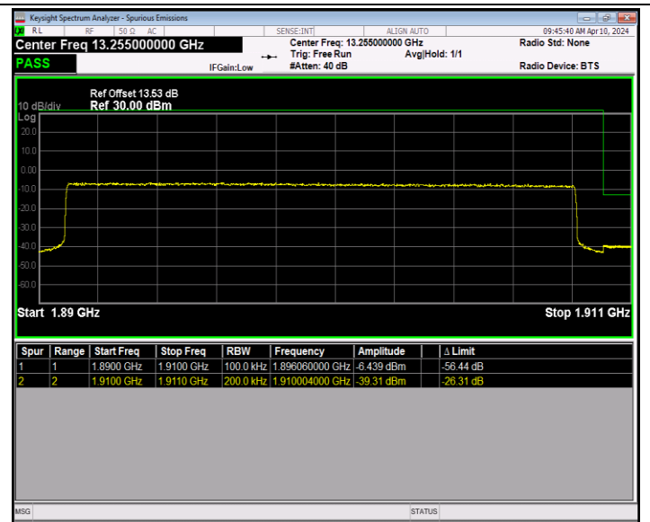
Band2_20MHz_16QAM_19100_100RB#0
