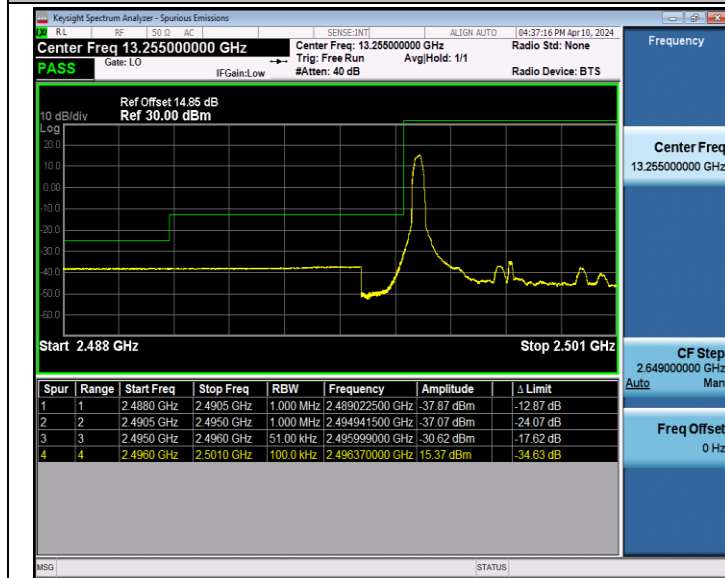
Band41_5MHz_16QAM_39675_1RB#0
