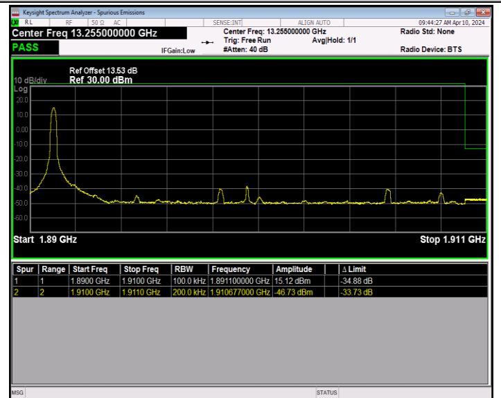
Band2_20MHz_16QAM_19100_1RB#0
