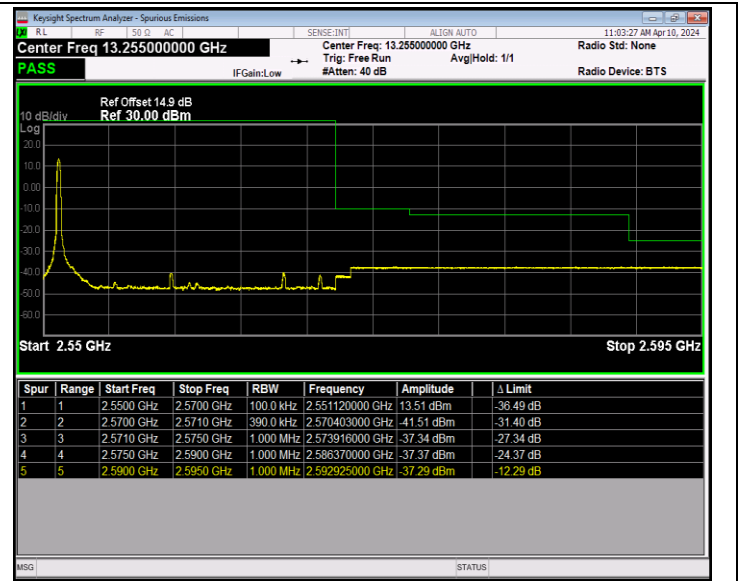
Band7_20MHz_64QAM_21350_1RB#0
