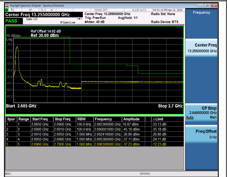
Band41_5MHz_QPSK_41565_1RB#0
