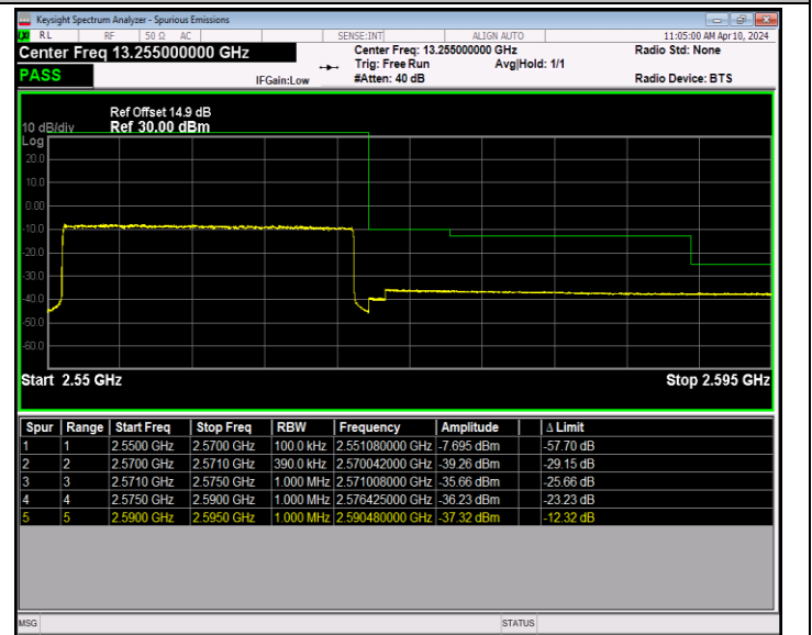
Band7_20MHz_64QAM_21350_100RB#0
