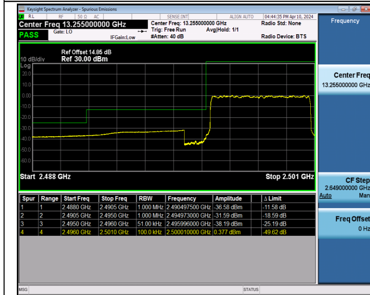
Band41_5MHz_QPSK_39675_25RB#0
