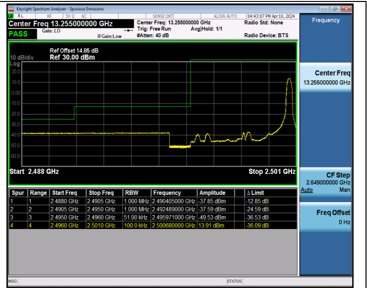
Band41_5MHz_64QAM_39675_1RB#24
