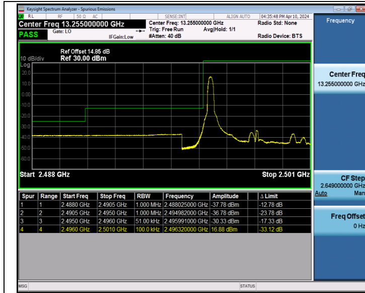
Band41_5MHz_QPSK_39675_1RB#0
