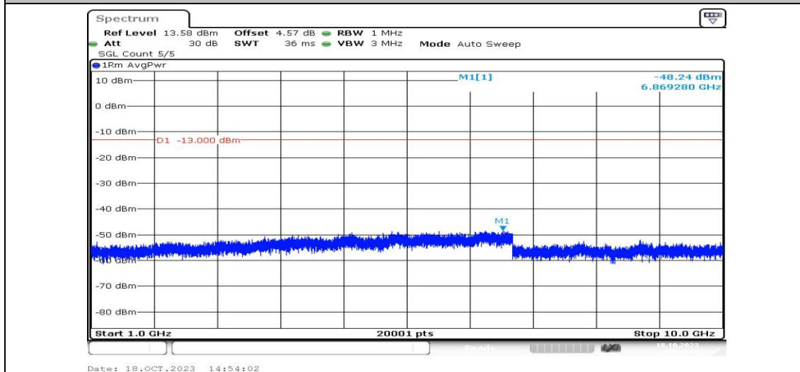
Band12-3MHz-16QAM-23095-1RB#0-Range4:1000~10000MHz-PASS
