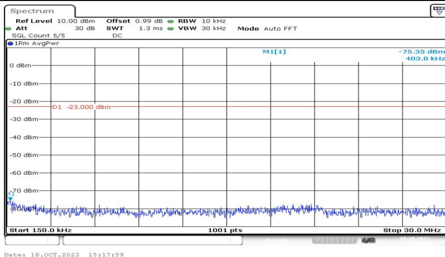
Band12-5MHz-QPSK-23095-1RB#0-Range2:0.15~30MHz-PASS
