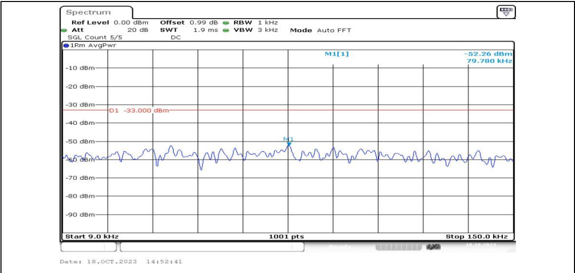
Band12-3MHz-QPSK-23095-1RB#0-Range1:0.009~0.15MHz-PASS
