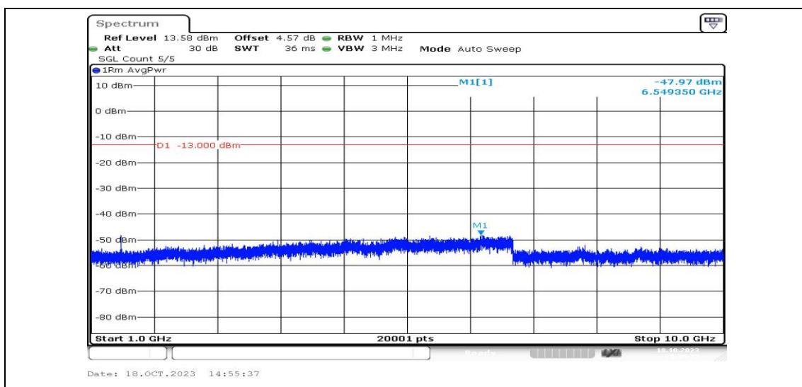
Band12-3MHz-16QAM-23165-1RB#0-Range4:1000~10000MHz-PASS
