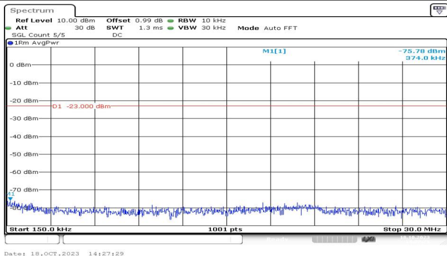
Band12-1.4MHz-16QAM-23017-1RB#0-Range2:0.15~30MHz-PASS
