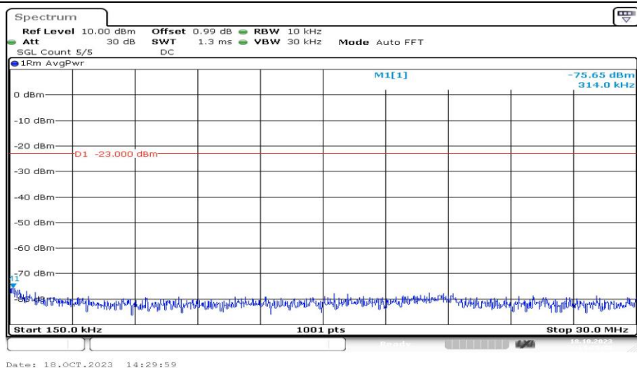
Band12-1.4MHz-QPSK-23173-1RB#0-Range2:0.15~30MHz-PASS
