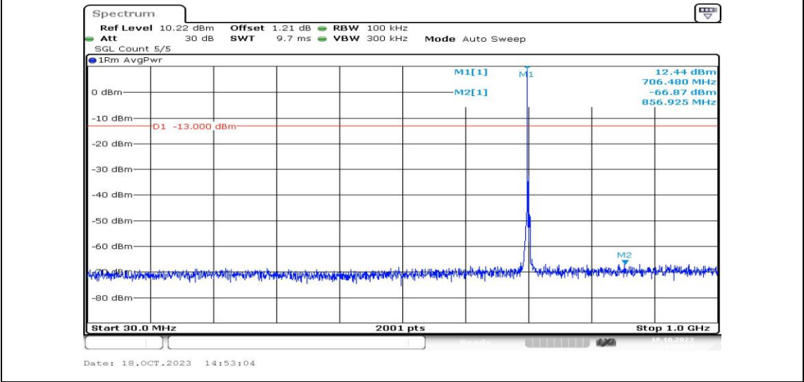
Band12-3MHz-QPSK-23095-1RB#0-Range3:30~1000MHz-PASS
