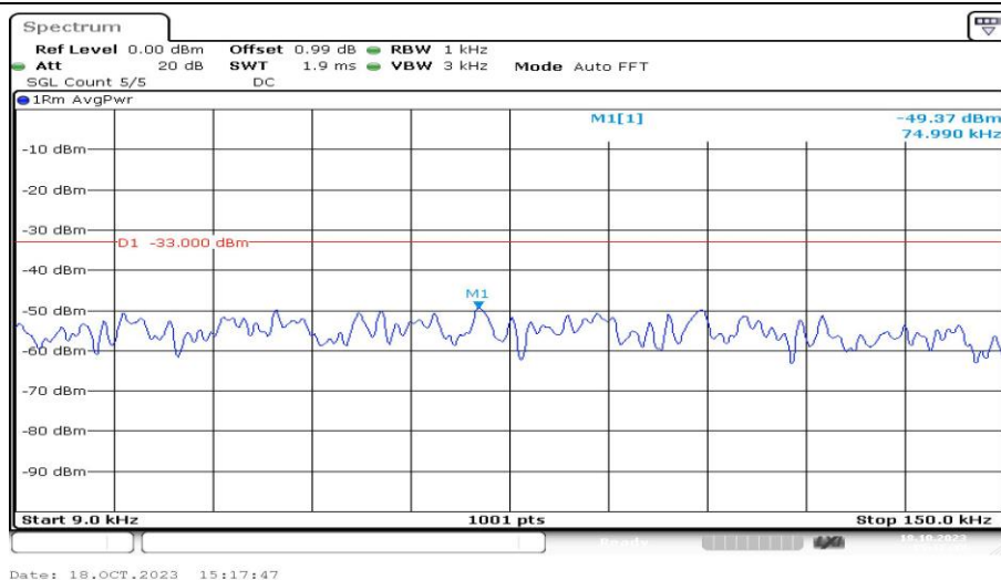
Band12-5MHz-QPSK-23095-1RB#0-Range1:0.009~0.15MHz-PASS
