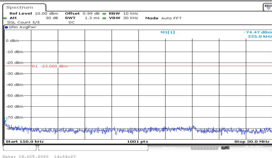
Band12-3MHz-QPSK-23165-1RB#0-Range2:0.15~30MHz-PASS
