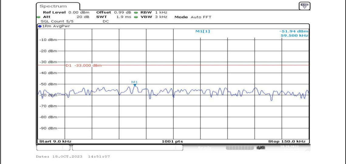
Band12-3MHz-QPSK-23025-1RB#0-Range1:0.009~0.15MHz-PASS
