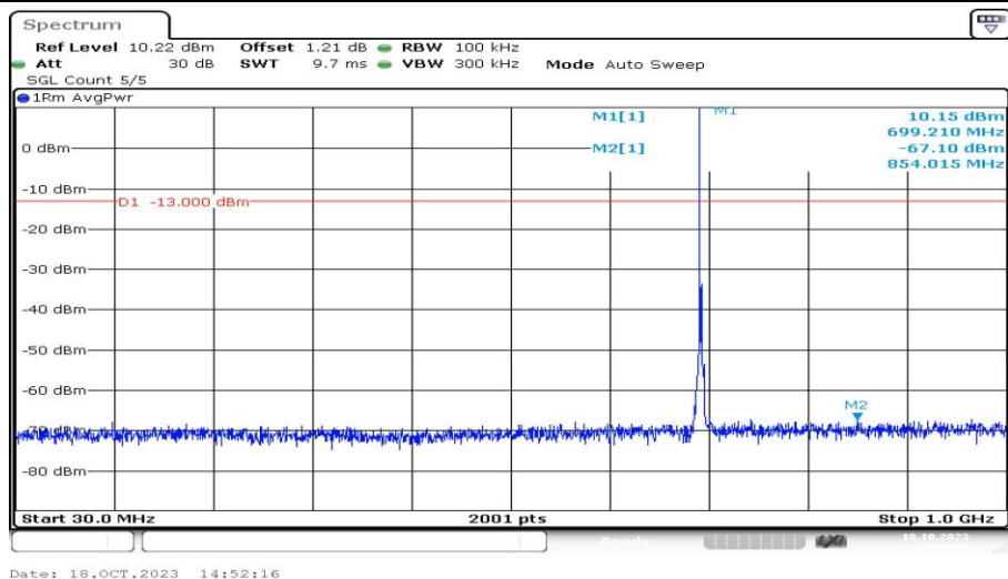
Band12-3MHz-16QAM-23025-1RB#0-Range3:30~1000MHz-PASS
