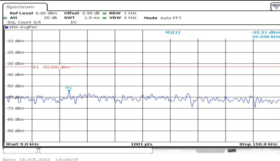
Band12-1.4MHz-16QAM-23095-1RB#0-Range1:0.009~0.15MHz-PASS
