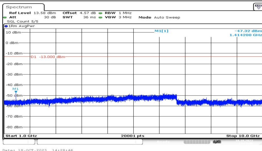
Band12-1.4MHz-QPSK-23095-1RB#0-Range4:1000~10000MHz-PASS
