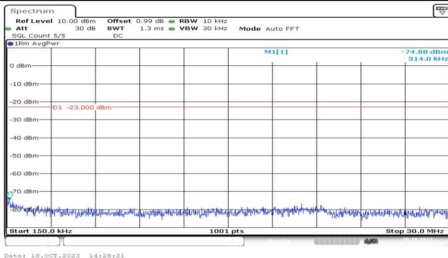
Band12-1.4MHz-QPSK-23095-1RB#0-Range2:0.15~30MHz-PASS
