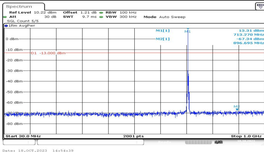
Band12-3MHz-QPSK-23165-1RB#0-Range3:30~1000MHz-PASS
