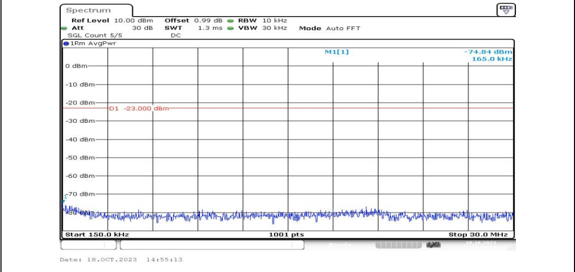
Band12-3MHz-16QAM-23165-1RB#0-Range2:0.15~30MHz-PASS
