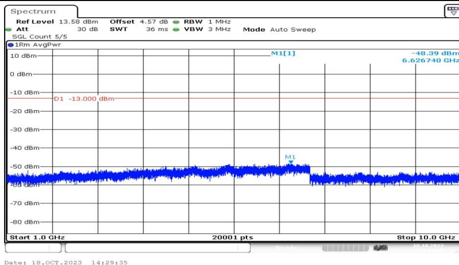
Band12-1.4MHz-16QAM-23095-1RB#0-Range4:1000~10000MHz-PASS
