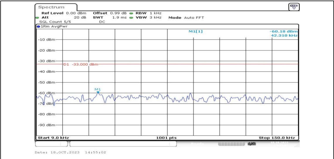
Band12-3MHz-16QAM-23165-1RB#0-Range1:0.009~0.15MHz-PASS
