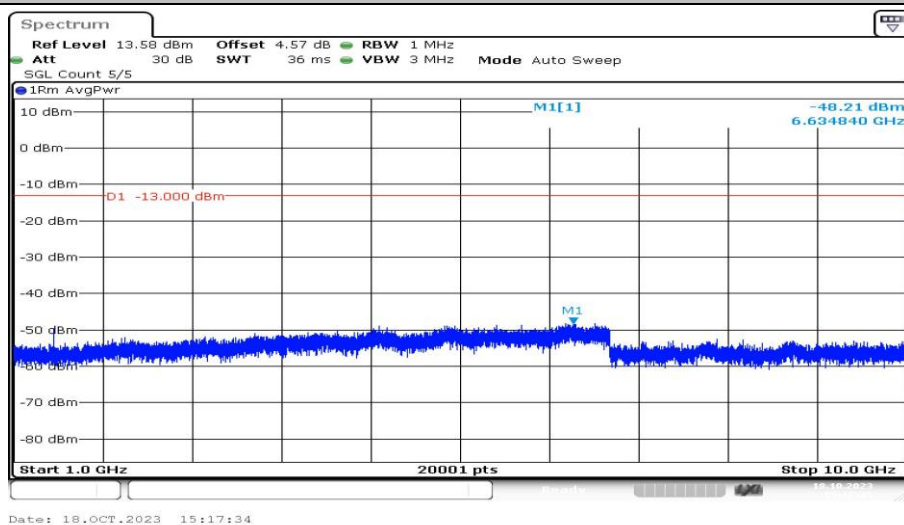
Band12-5MHz-16QAM-23035-1RB#0-Range4:1000~10000MHz-PASS
