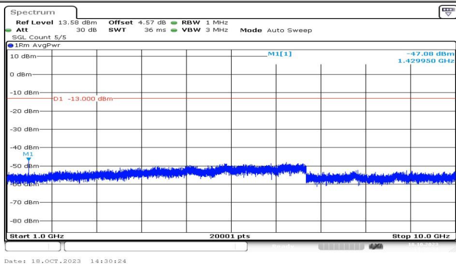
Band12-1.4MHz-QPSK-23173-1RB#0-Range4:1000~10000MHz-PASS
