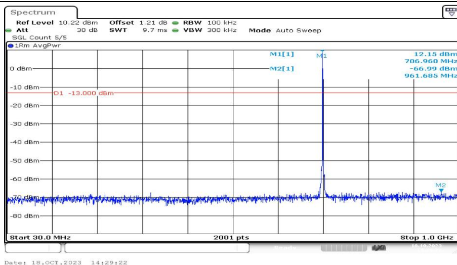
Band12-1.4MHz-16QAM-23095-1RB#0-Range3:30~1000MHz-PASS
