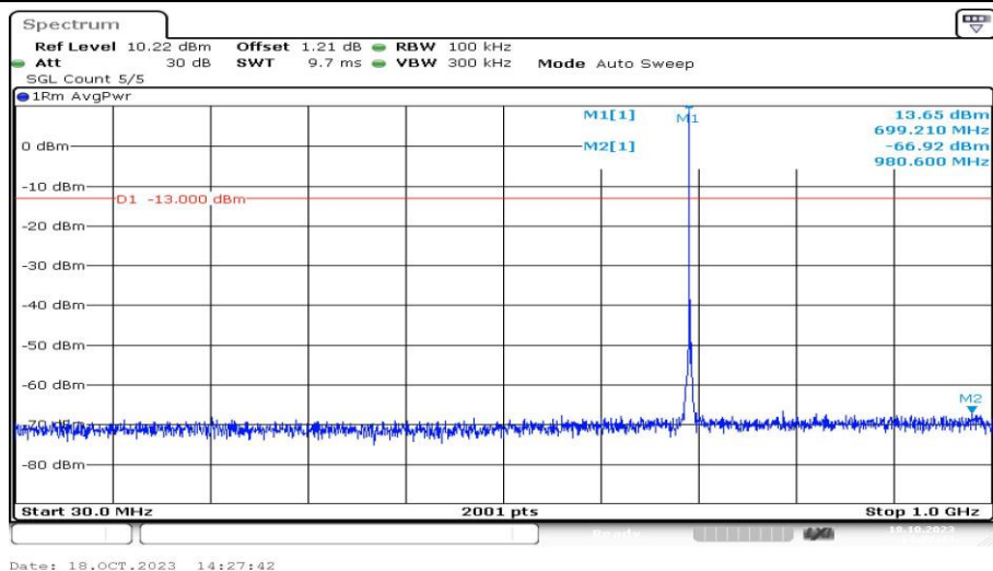
Band12-1.4MHz-16QAM-23017-1RB#0-Range3:30~1000MHz-PASS
