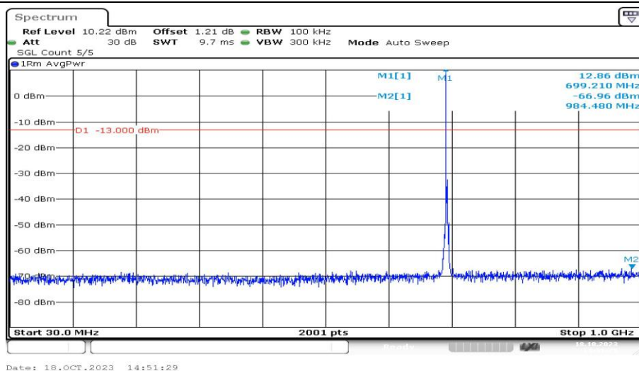
Band12-3MHz-QPSK-23025-1RB#0-Range3:30~1000MHz-PASS
