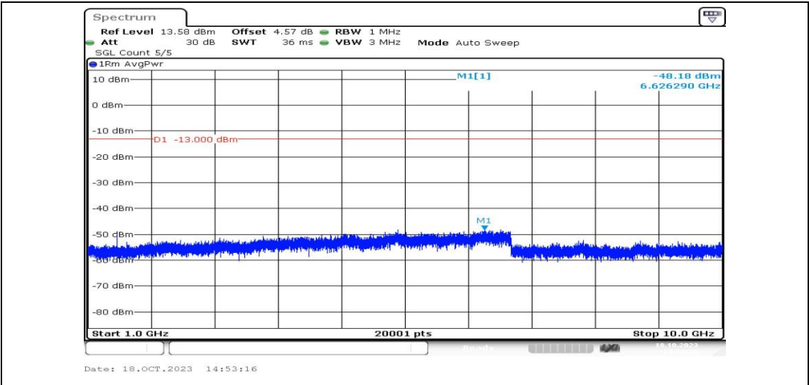
Band12-3MHz-QPSK-23095-1RB#0-Range4:1000~10000MHz-PASS
