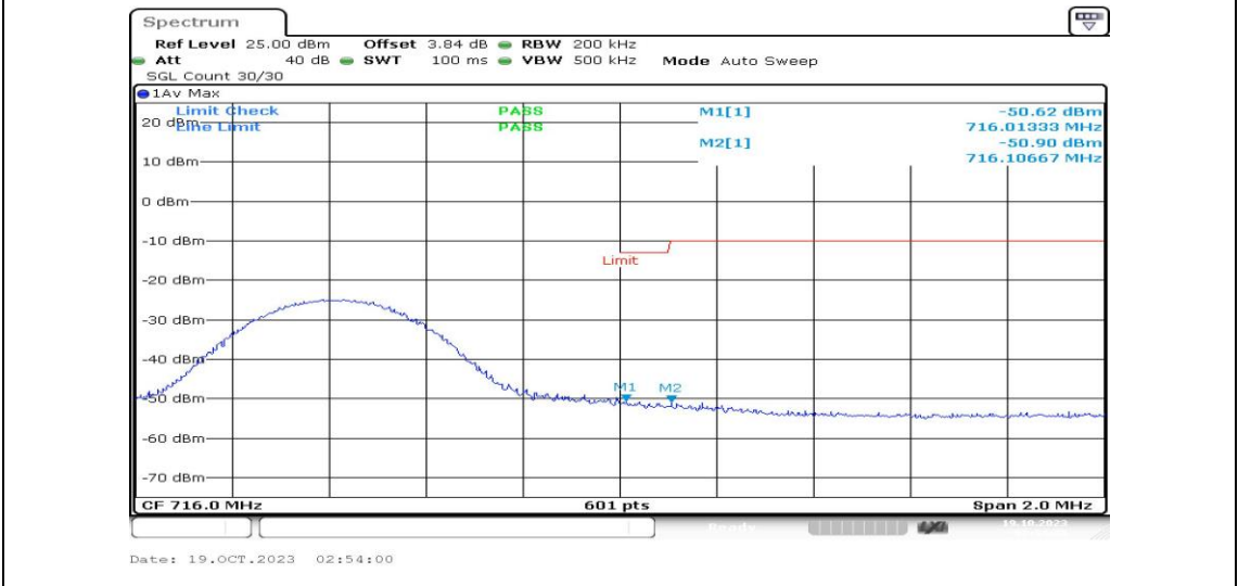
Band12-10MHz-QPSK-23130-1RB#0-PASS
