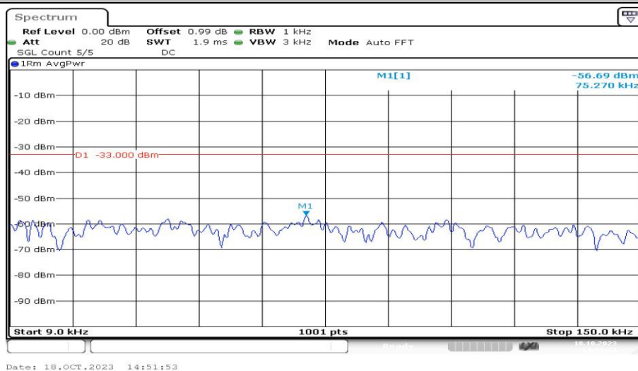
Band12-3MHz-16QAM-23025-1RB#0-Range1:0.009~0.15MHz-PASS
