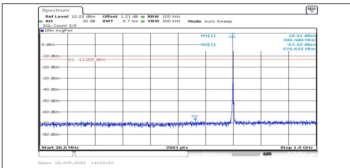
Band12-3MHz-16QAM-23095-1RB#0-Range3:30~1000MHz-PASS
