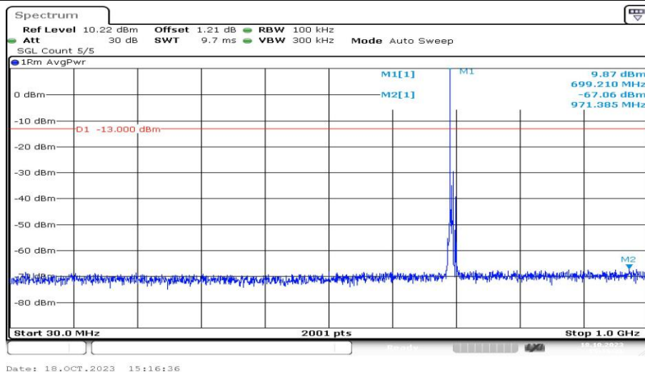
Band12-5MHz-QPSK-23035-1RB#0-Range3:30~1000MHz-PASS
