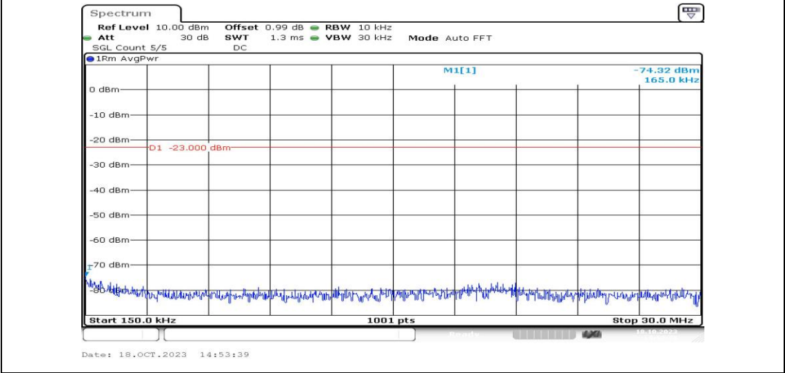
Band12-3MHz-16QAM-23095-1RB#0-Range2:0.15~30MHz-PASS
