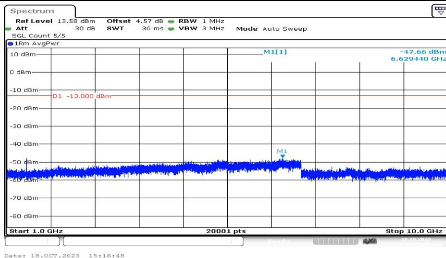
Band12-5MHz-QPSK-23035-1RB#0-Range4:1000~10000MHz-PASS
