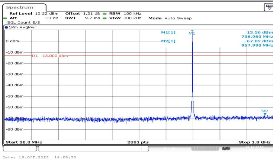
Band12-1.4MHz-QPSK-23095-1RB#0-Range3:30~1000MHz-PASS
