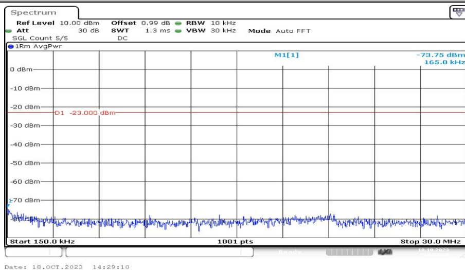
Band12-1.4MHz-16QAM-23095-1RB#0-Range2:0.15~30MHz-PASS
