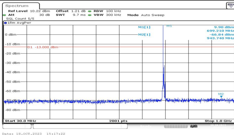
Band12-5MHz-16QAM-23035-1RB#0-Range3:30~1000MHz-PASS
