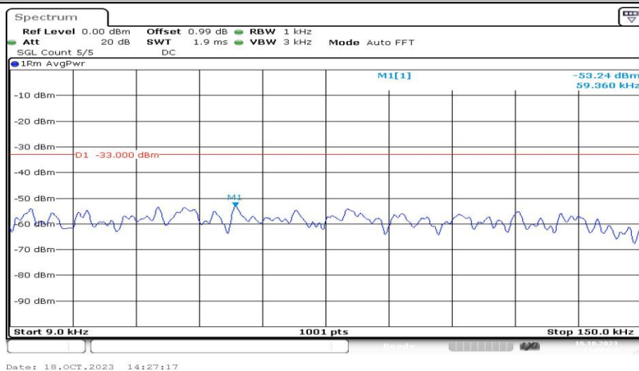
Band12-1.4MHz-16QAM-23017-1RB#0-Range1:0.009~0.15MHz-PASS
