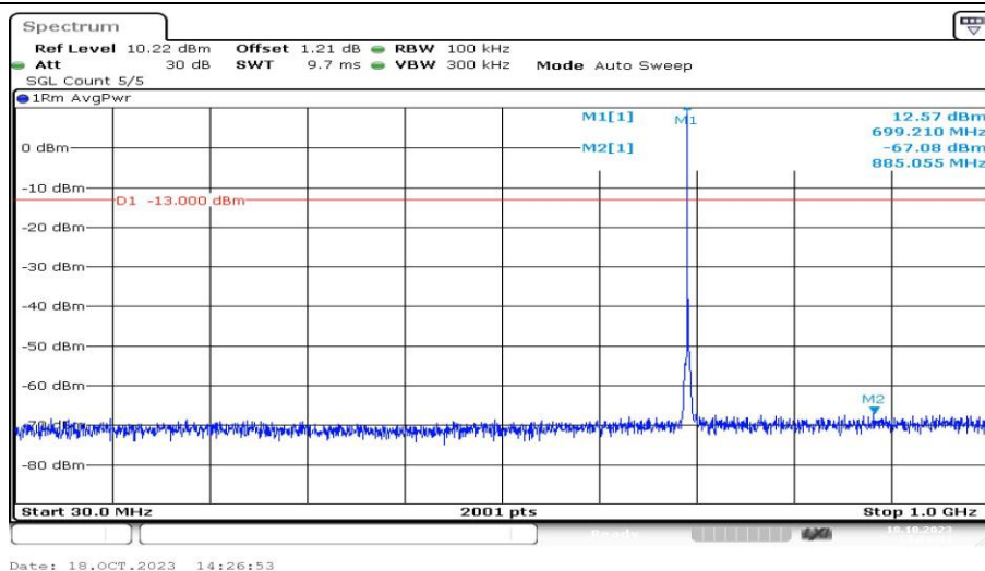
Band12-1.4MHz-QPSK-23017-1RB#0-Range3:30~1000MHz-PASS
