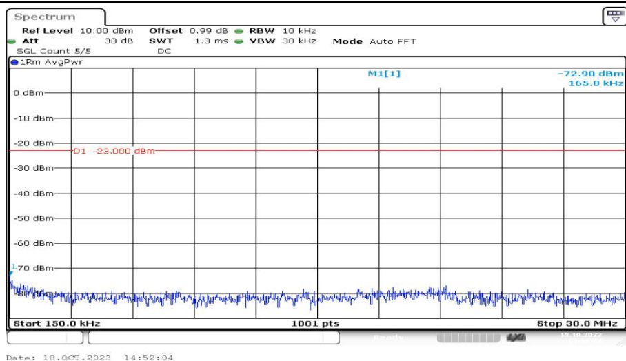
Band12-3MHz-16QAM-23025-1RB#0-Range2:0.15~30MHz-PASS
