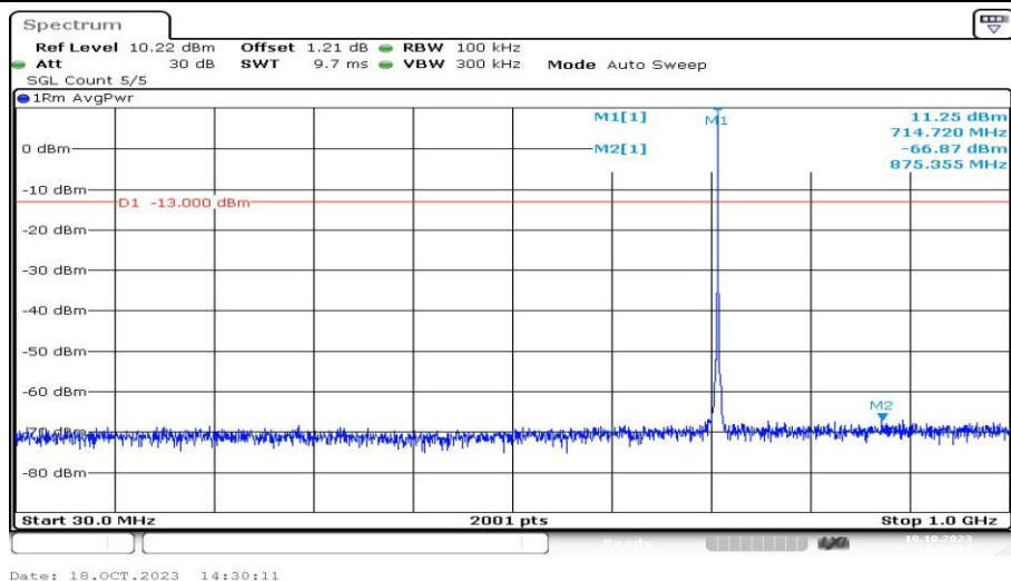
Band12-1.4MHz-QPSK-23173-1RB#0-Range3:30~1000MHz-PASS
