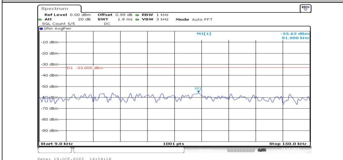
Band12-3MHz-QPSK-23165-1RB#0-Range1:0.009~0.15MHz-PASS
