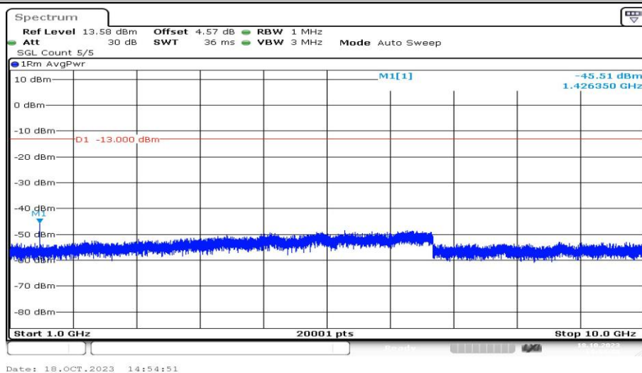
Band12-3MHz-QPSK-23165-1RB#0-Range4:1000~10000MHz-PASS
