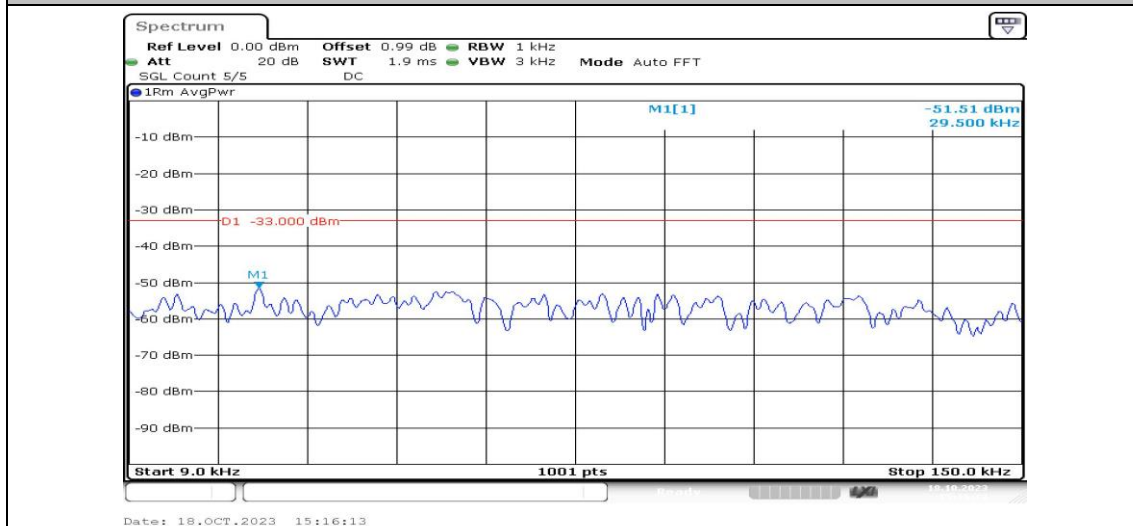
Band12-5MHz-QPSK-23035-1RB#0-Range1:0.009~0.15MHz-PASS
