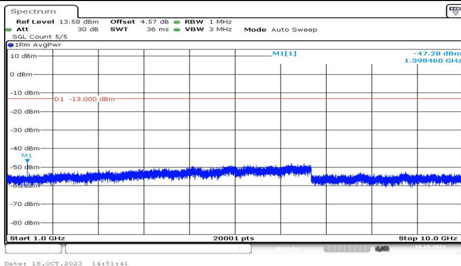
Band12-3MHz-QPSK-23025-1RB#0-Range4:1000~10000MHz-PASS
