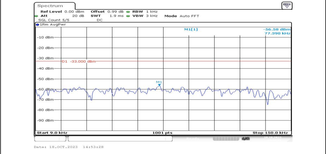
Band12-3MHz-16QAM-23095-1RB#0-Range1:0.009~0.15MHz-PASS
