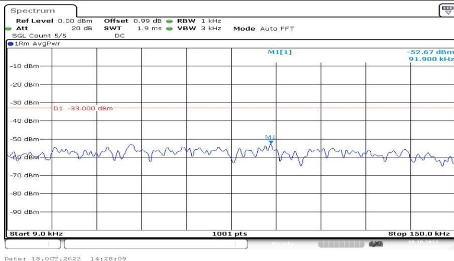
Band12-1.4MHz-QPSK-23095-1RB#0-Range1:0.009~0.15MHz-PASS
