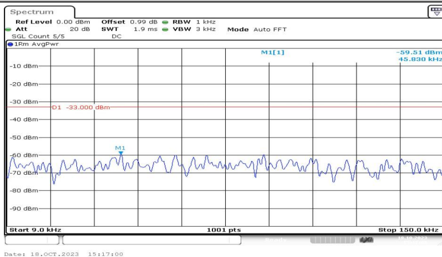
Band12-5MHz-16QAM-23035-1RB#0-Range1:0.009~0.15MHz-PASS
