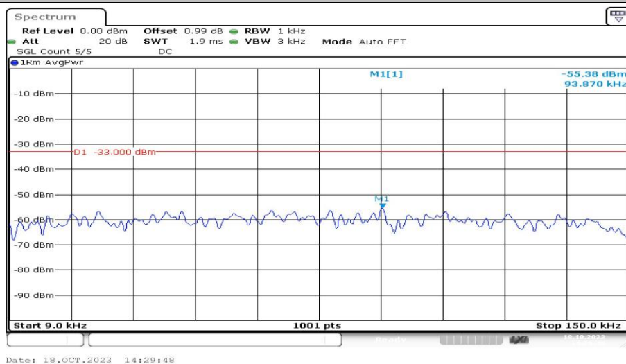
Band12-1.4MHz-QPSK-23173-1RB#0-Range1:0.009~0.15MHz-PASS
