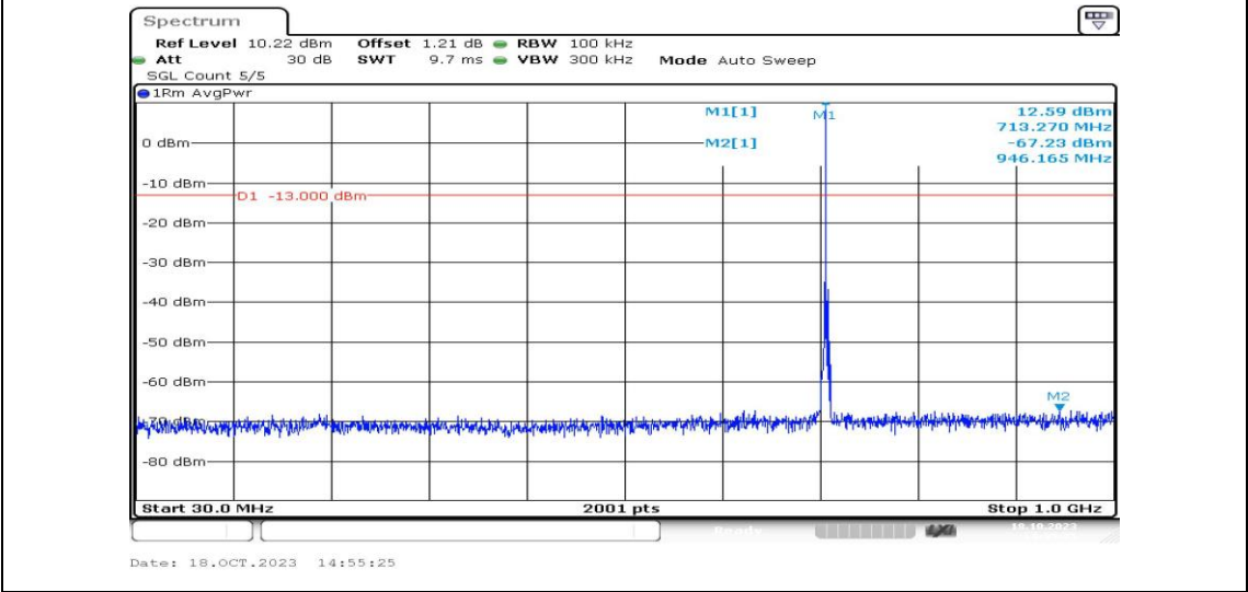
Band12-3MHz-16QAM-23165-1RB#0-Range3:30~1000MHz-PASS
