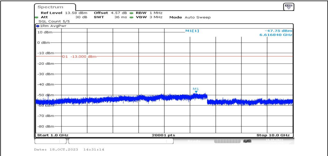
Band12-1.4MHz-16QAM-23173-1RB#0-Range4:1000~10000MHz-PASS
