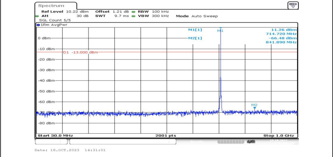
Band12-1.4MHz-16QAM-23173-1RB#0-Range3:30~1000MHz-PASS
