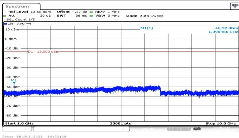
Band12-3MHz-16QAM-23025-1RB#0-Range4:1000~10000MHz-PASS
