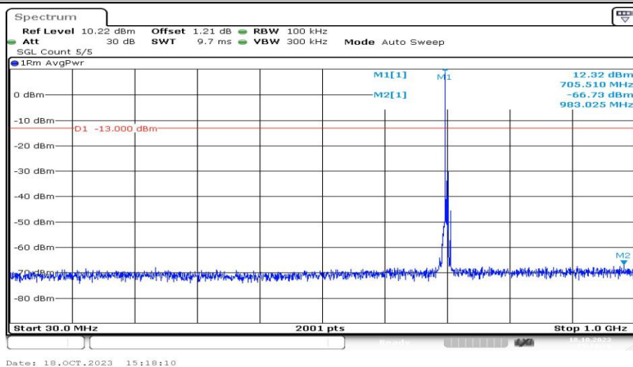
Band12-5MHz-QPSK-23095-1RB#0-Range3:30~1000MHz-PASS
