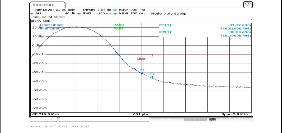
Band12-10MHz-QPSK-23130-1RB#49-PASS
