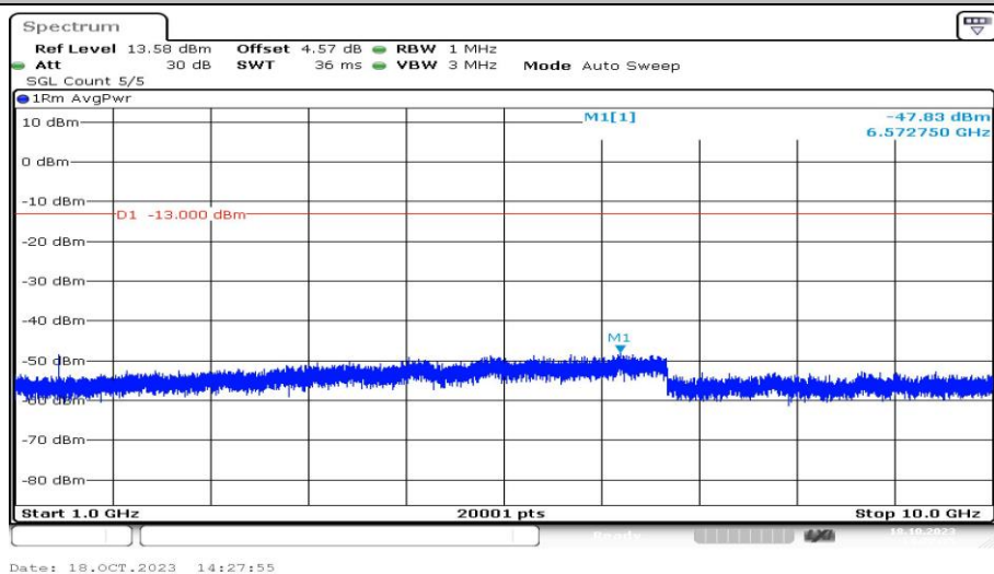
Band12-1.4MHz-16QAM-23017-1RB#0-Range4:1000~10000MHz-PASS
