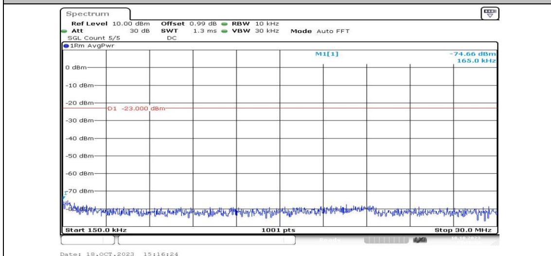
Band12-5MHz-QPSK-23035-1RB#0-Range2:0.15~30MHz-PASS
