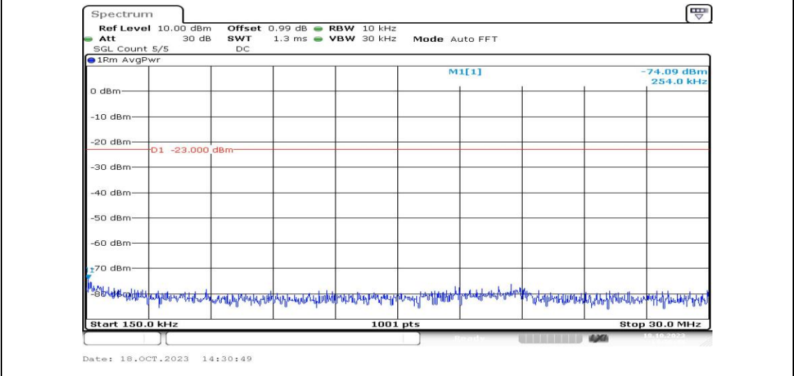
Band12-1.4MHz-16QAM-23173-1RB#0-Range2:0.15~30MHz-PASS
