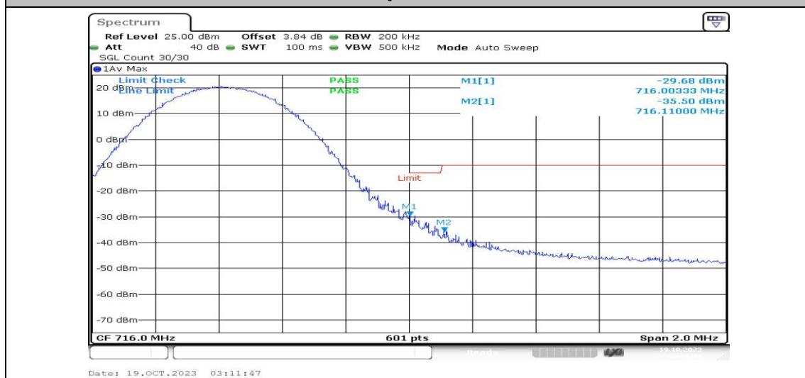
Band12-10MHz-16QAM-23130-1RB#49-PASS
