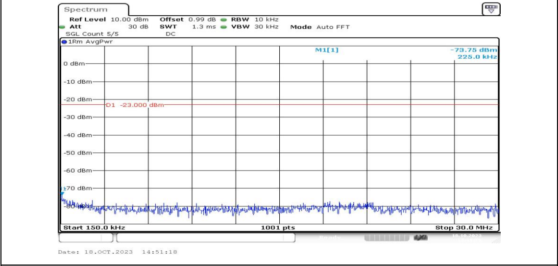
Band12-3MHz-QPSK-23025-1RB#0-Range2:0.15~30MHz-PASS
