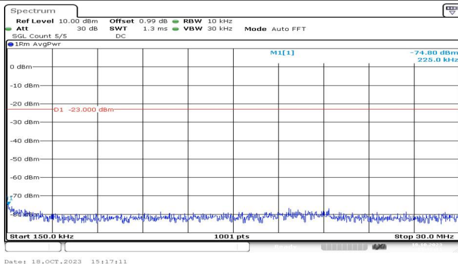
Band12-5MHz-16QAM-23035-1RB#0-Range2:0.15~30MHz-PASS
