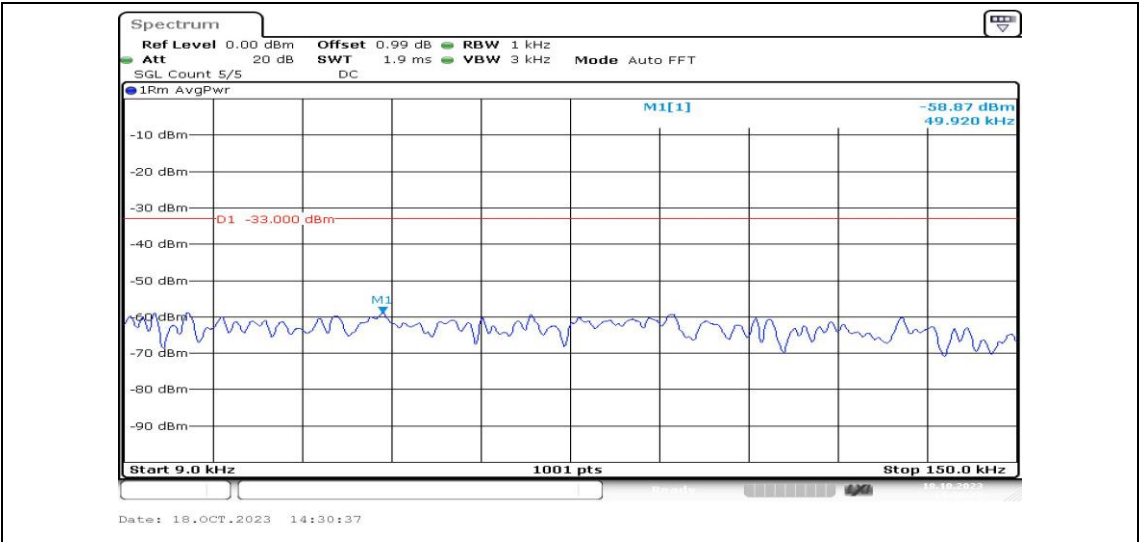
Band12-1.4MHz-16QAM-23173-1RB#0-Range1:0.009~0.15MHz-PASS
