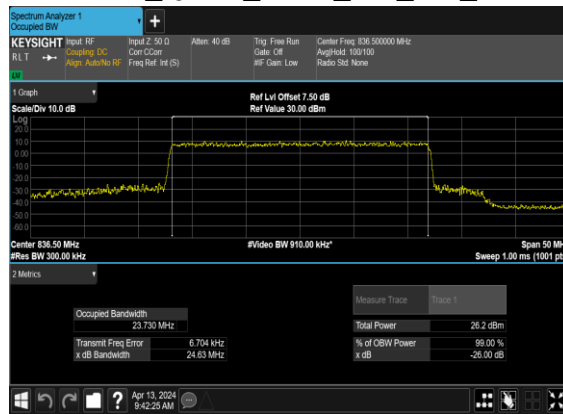
N5(25M)_CP-OFDM_QPSK_Outer_Full_Mid_CH
