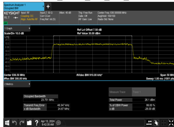
N5(25M)_CP-OFDM_16 QAM_Outer_Full_Mid_CH
