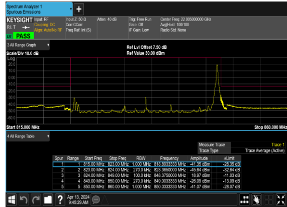
N5(25M)_DFT-s-OFDM_QPSK_Edge_1RB_Right_Mid_CH
