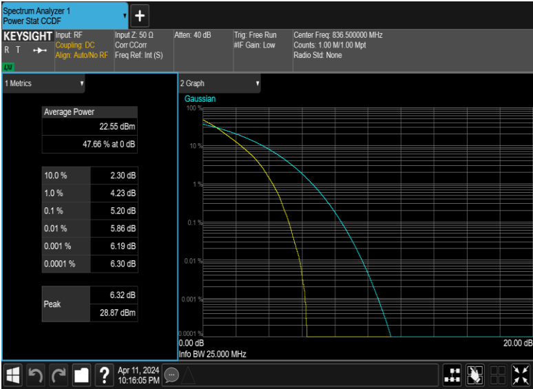
N26(20M)_DFT-s-OFDM_QPSK_Outer_Full_Mid_CH
