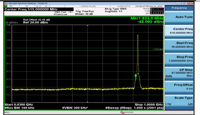
Band5_5MHz_16QAM_20525_25RB#0_30~1000_30~100 0
