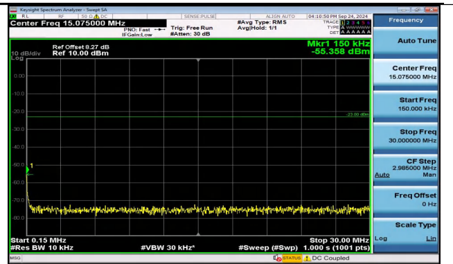
Band5_5MHz_QPSK_20625_25RB#0_0.15~30_0.15~30
