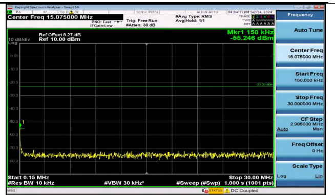
Band5_5MHz_QPSK_20525_1RB#24_0.15~30_0.15~30
