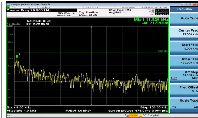
Band5_5MHz_QPSK_20625_25RB#0_0.009~0.15_0.009 ~0.15
