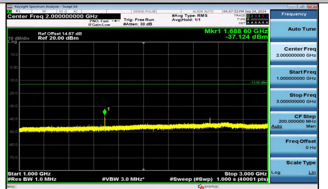
Band5_5MHz_QPSK_20625_1RB#0_1000~3000_1000~3000 00
