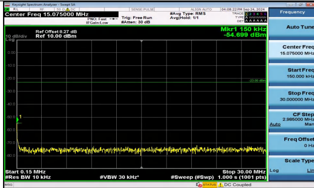
Band5_5MHz_16QAM_20625_1RB#0_0.15~30_0.15~30
