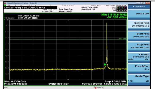
Band5_5MHz_16QAM_20525_1RB#0_30~1000_30~1000
