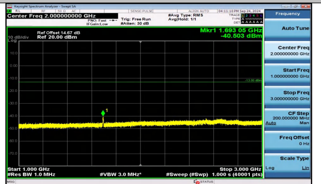
Band5_5MHz_QPSK_20625_25RB#0_1000~3000_1000~3000
