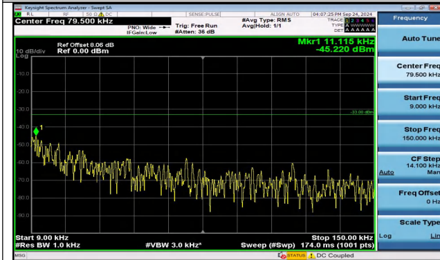
Band5_5MHz_QPSK_20625_1RB#0_0.009~0.15_0.009~0.15 0.15
