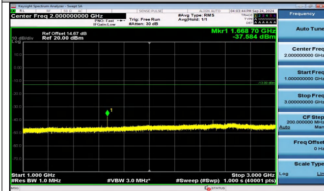
Band5_5MHz_16QAM_20525_1RB#0_1000~3000_1000~3000
