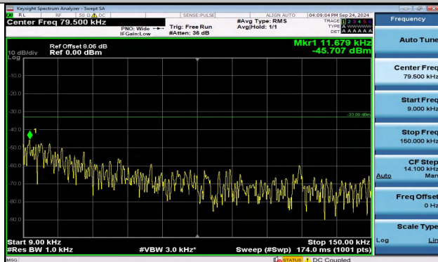
Band5_5MHz_QPSK_20625_1RB#24_0.009~0.15_0.009~0.15
