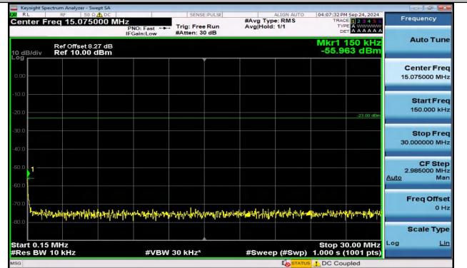
Band5_5MHz_QPSK_20625_1RB#0_0.15~30_0.15~30
