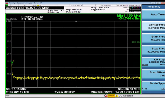
Band5_5MHz_16QAM_20525_25RB#0_0.15~30_0.15~3 0
