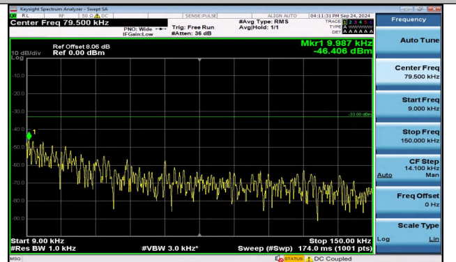
Band5_5MHz_16QAM_20625_25RB#0_0.009~0.15_0.009
