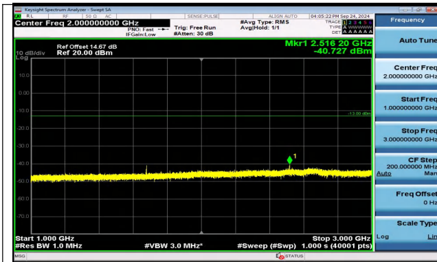
Band5_5MHz_16QAM_20525_1RB#24_1000~3000_1000 ~3000
