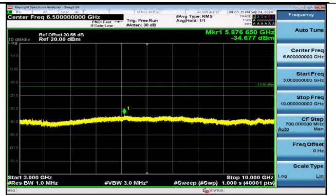
Band5_5MHz_16QAM_20525_1RB#24_3000~10000_3000 ~10000
