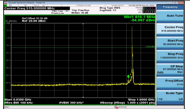
Band5_5MHz_16QAM_20625_1RB#0_30~1000_30~1000
