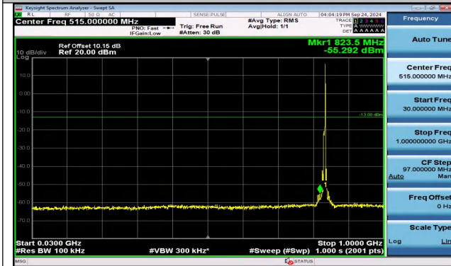
Band5_5MHz_QPSK_20525_1RB#24_30~1000_30~1000
