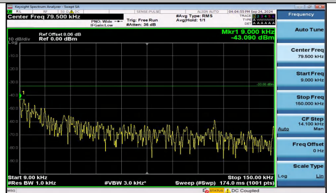
Band5_5MHz_16QAM_20525_1RB#24_0.009~0.15_0.009~0.15
