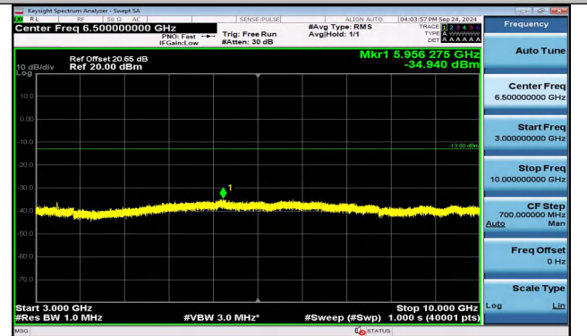
Band5_5MHz_16QAM_20525_1RB#0_3000~10000_3000~10000
