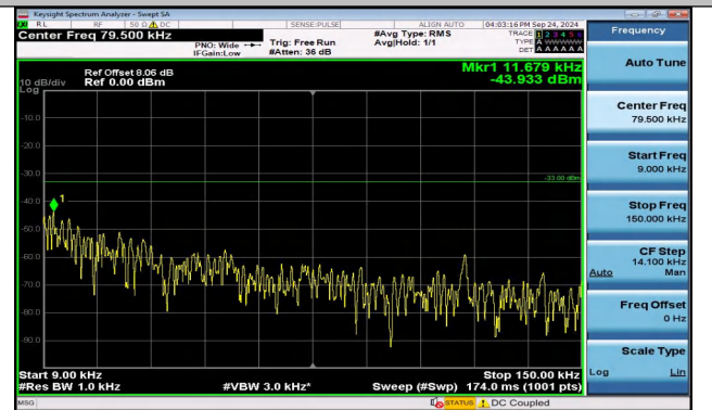
Band5_5MHz_16QAM_20525_1RB#0_0.009~0.15_0.009~0.15
