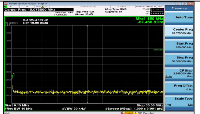
Band5_5MHz_QPSK_20625_1RB#24_0.15~30_0.15~30
