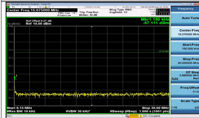
Band5_5MHz_16QAM_20525_1RB#0_0.15~30_0.15~30
