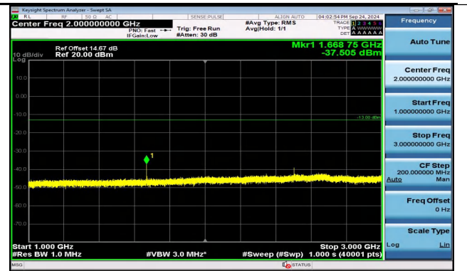
Band5_5MHz_QPSK_20525_1RB#0_1000~3000_1000~3000
