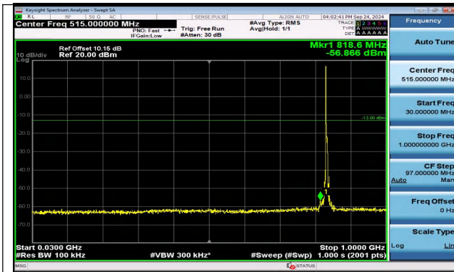
Band5_5MHz_QPSK_20525_1RB#0_30~1000_30~1000
