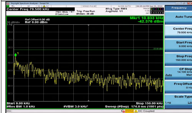
Band5_5MHz_QPSK_20525_25RB#0_0.009~0.15_0.009 ~0.15
