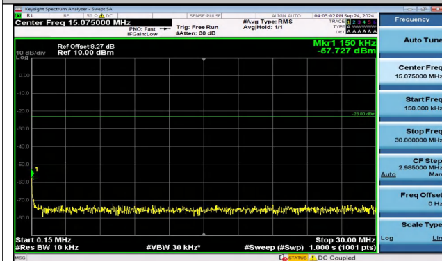
Band5_5MHz_16QAM_20525_1RB#24_0.15~30_0.15~30
