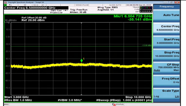
Band5_5MHz_16QAM_20625_1RB#0_3000~10000_3000~10000
