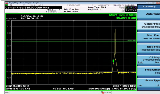
Band5_5MHz_QPSK_20525_25RB#0_30~1000_30~1000
