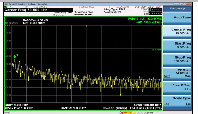
Band5_5MHz_16QAM_20525_25RB#0_0.009~0.15_0.009 ~0.15
