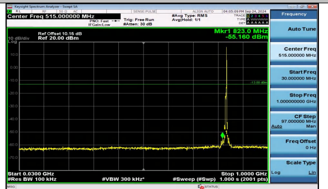
Band5_5MHz_16QAM_20525_1RB#24_30~1000_30~1000
