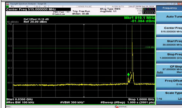
Band5_5MHz_QPSK_20625_1RB#0_30~1000_30~1000
