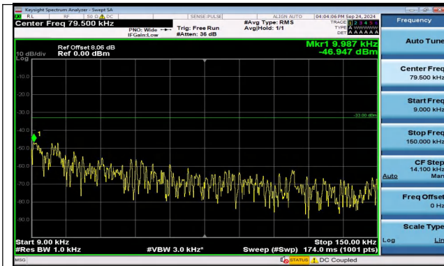
Band5_5MHz_QPSK_20525_1RB#24_0.009~0.15_0.009~0.15
