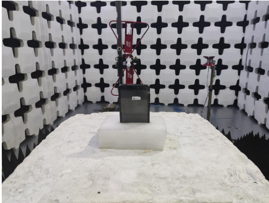
7. Radiated Emissions (Part 15C Wi-Fi/Bluetooth, 1GHz -18GHz)
