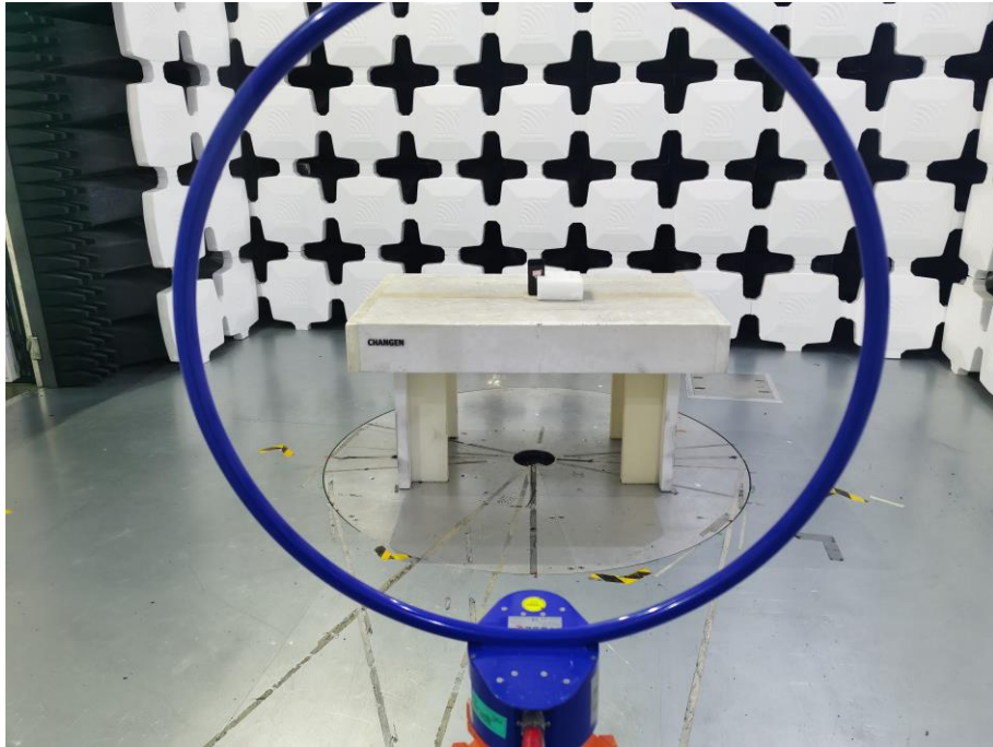
5. Radiated Emissions (Part 15C Wi-Fi/Bluetooth, 9kHz-30MHz)
