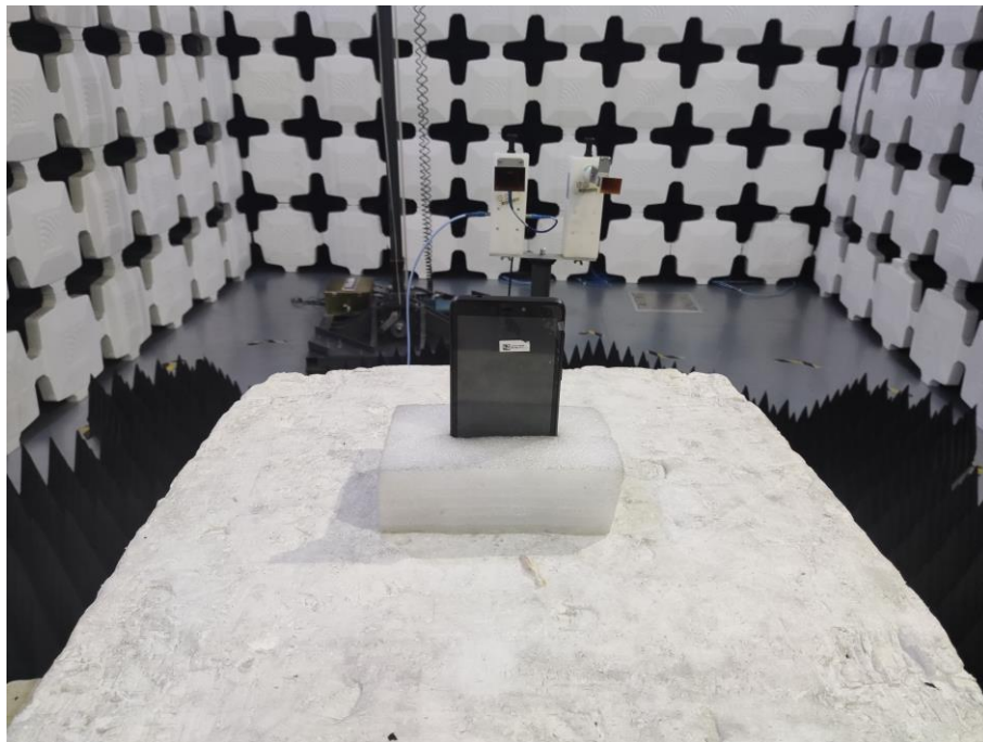
8. Radiated Emissions (Part 15C Wi-Fi/Bluetooth, 18GHz -26.5GHz)
