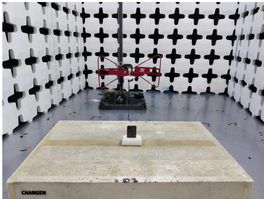
6. Radiated Emissions (Part 15C Wi-Fi/Bluetooth, 30MHz-1GHz)
