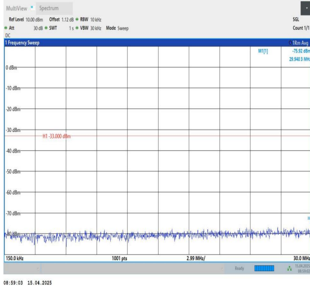
Band25-20MHz-QPSK-26590-1RB#99-0.15~30-PASS
