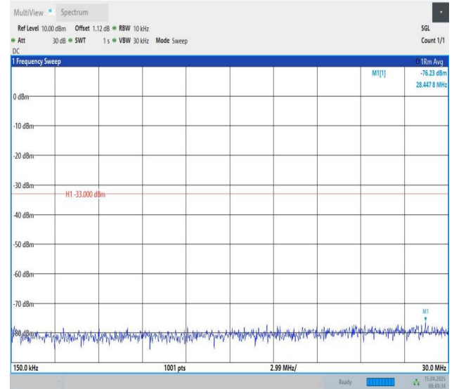
Band25-10MHz-QPSK-26640-1RB#0-0.15~30-PASS
