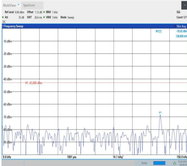
Band25-10MHz-QPSK-26640-1RB#0-0.009~0.15-PASS
