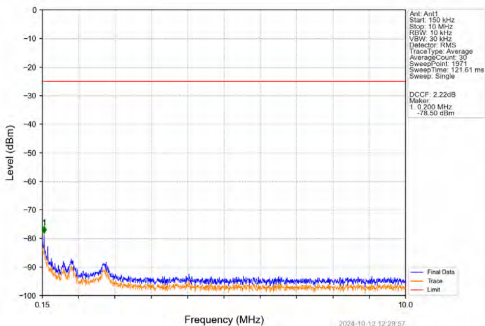
Band41_15MHz_16QAM_MCH_2593MHz_RB_1_0_NTNV
