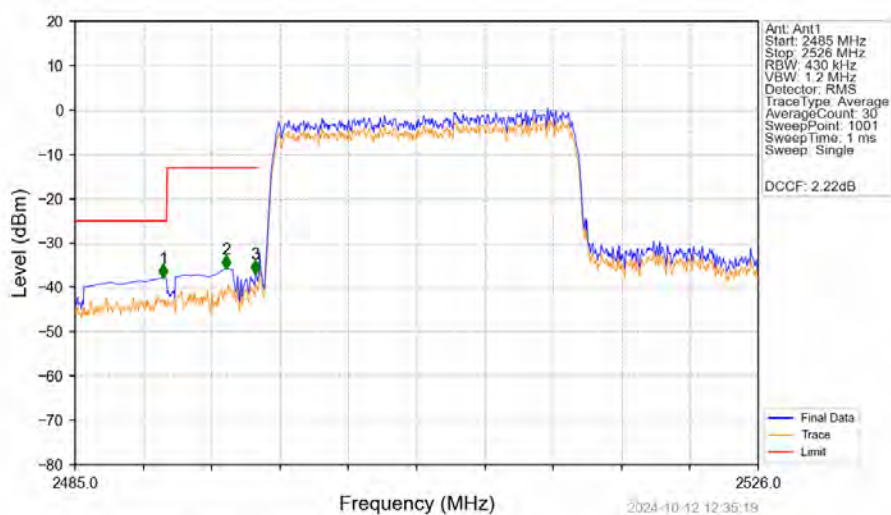
Band41_20MHz_16QAM_LCH_2506MHz_RB_100_0_NTNV
