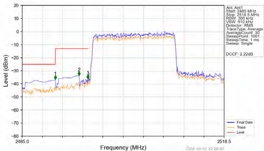
Band41_15MHz_16QAM_LCH_2503.5MHz_RB_75_0_NTNV
