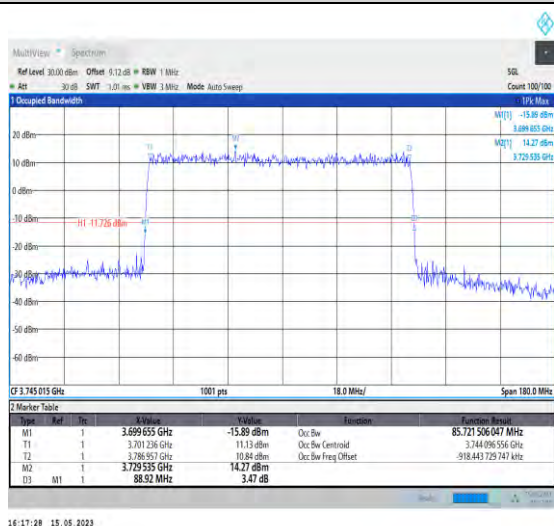
1-N77-3700-3980-PC1-30-90-L-4-DFT-64QAM-Out er_Full-240@0-Ant0-85.722-88.920-≤90-PASS
