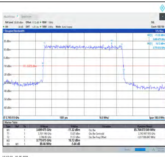
1-N77-3700-3980-PC1-30-90-L-2-DFT-PI2BPSK-Out er_Full-240@0-Ant0-85.704-89.460-≤90-PASS
