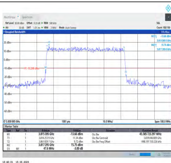
1-N77-3700-3980-PC1-30-50-M-1-DFT-QPSK-Outer Full-128@0-Ant0-45.586-47.600-≤50-PASS
