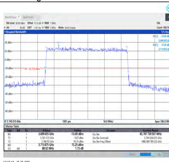
1-N77-3700-3980-PC1-30-90-L-3-DFT-16QAM-Out er_Full-240@0-Ant0-85.788-88.920-≤90-PASS
