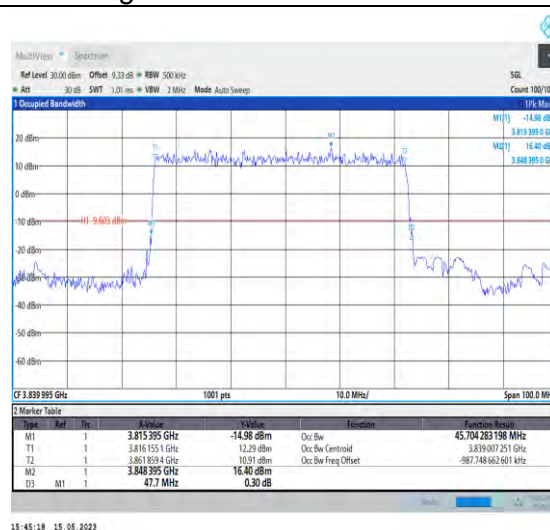
1-N77-3700-3980-PC1-30-50-M-2-DFT-PI2BPSK-O uter Full-128@0-Ant0-45.704-47.700-≤50-PASS
