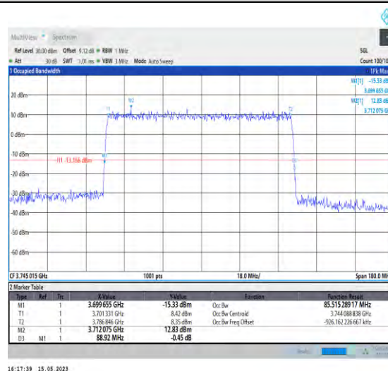
1-N77-3700-3980-PC1-30-90-L-5-DFT-256QAM-Out er_Full-240@0-Ant0-85.515-88.920-≤90-PASS
