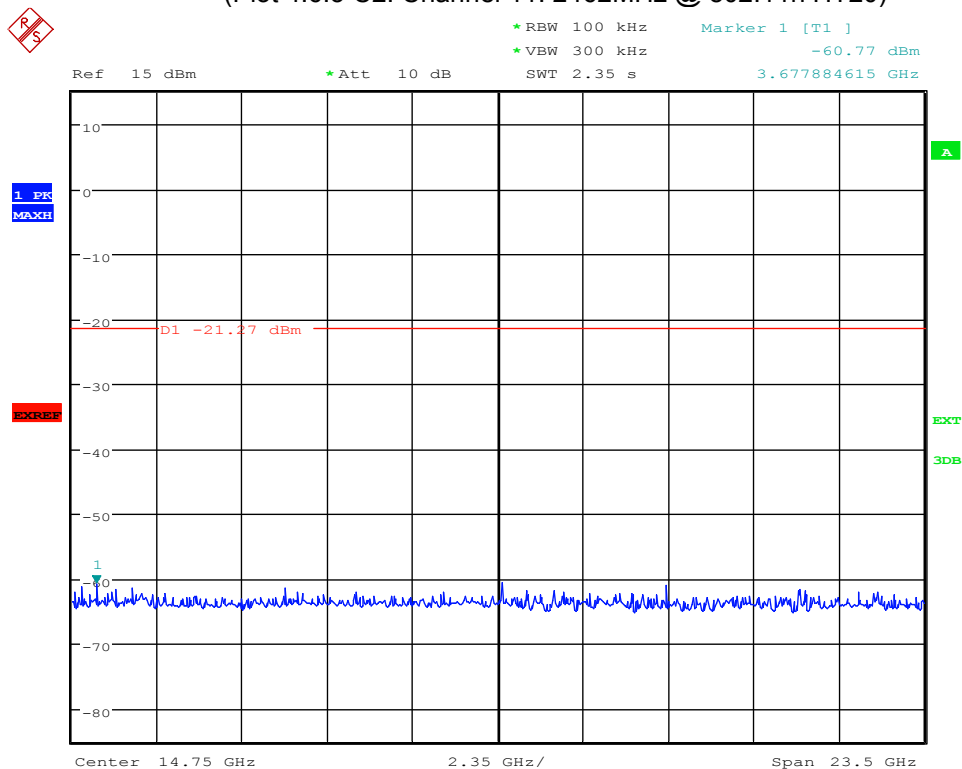
(Plot 4.6.3 C2: Channel 11: 2462MHz @ 802.11n HT20)
