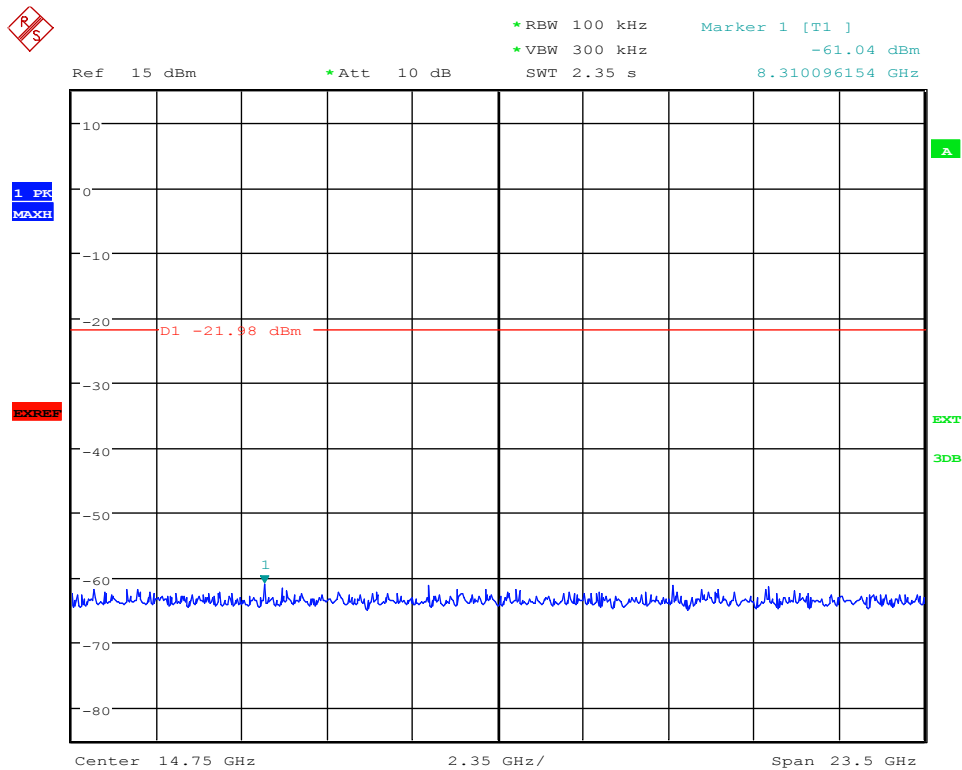
(Plot 4.6.3 A2: Channel 1: 2412MHz @ 802.11n HT20)
