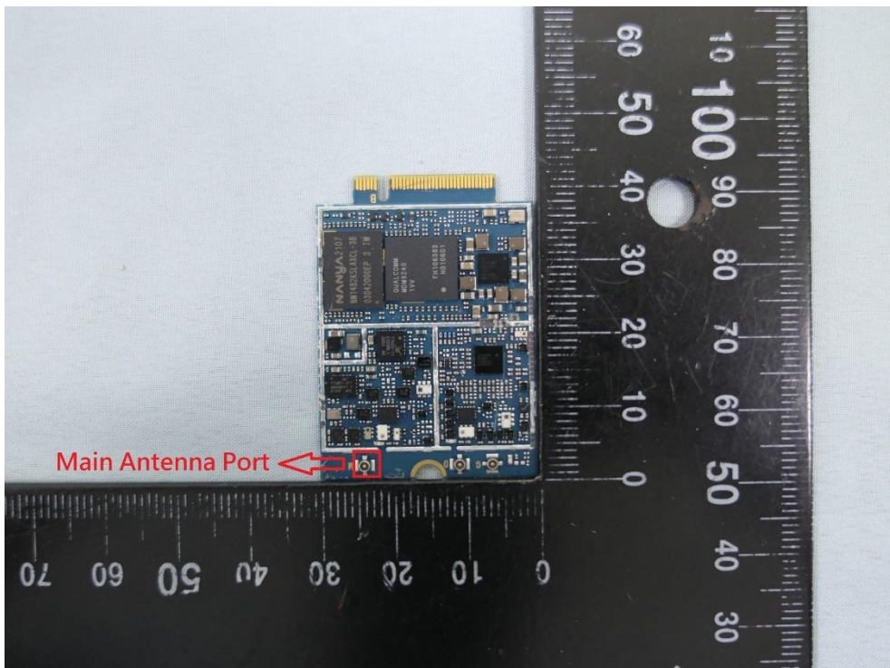
(32) EUT Photo
