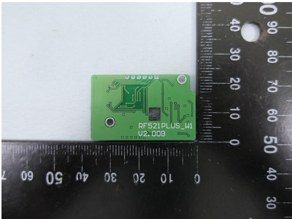
(38) EUT Photo
