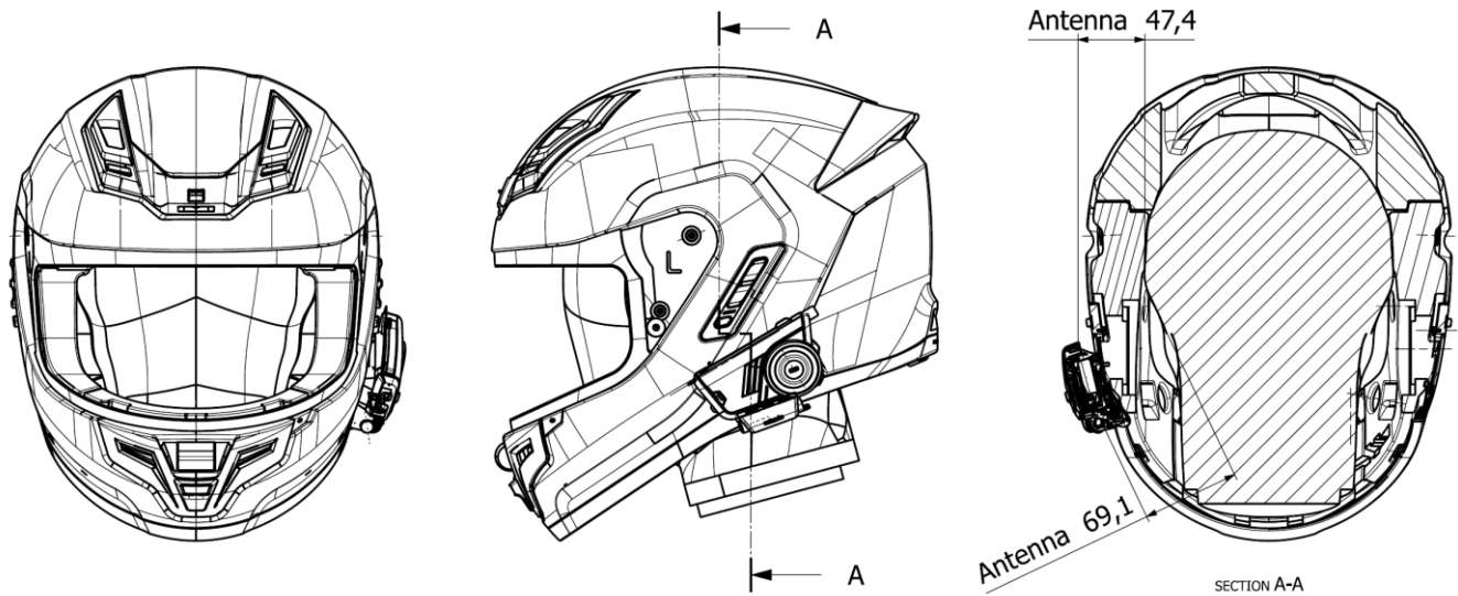
Figure E-1 Antenna Location
