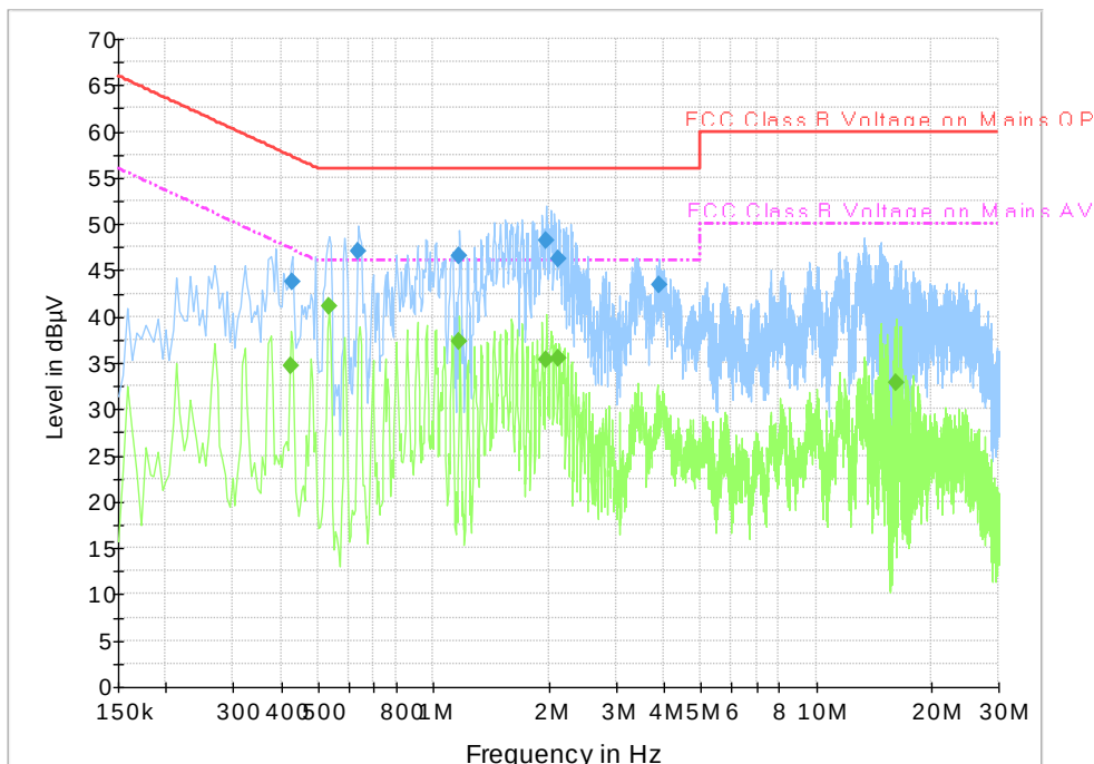
Fig.A.7.2 AC Powerline Conducted Emission-Idle
