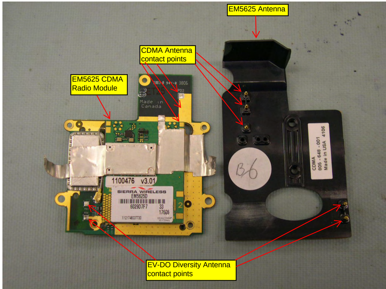
EM5625 module on support board and Antenna
