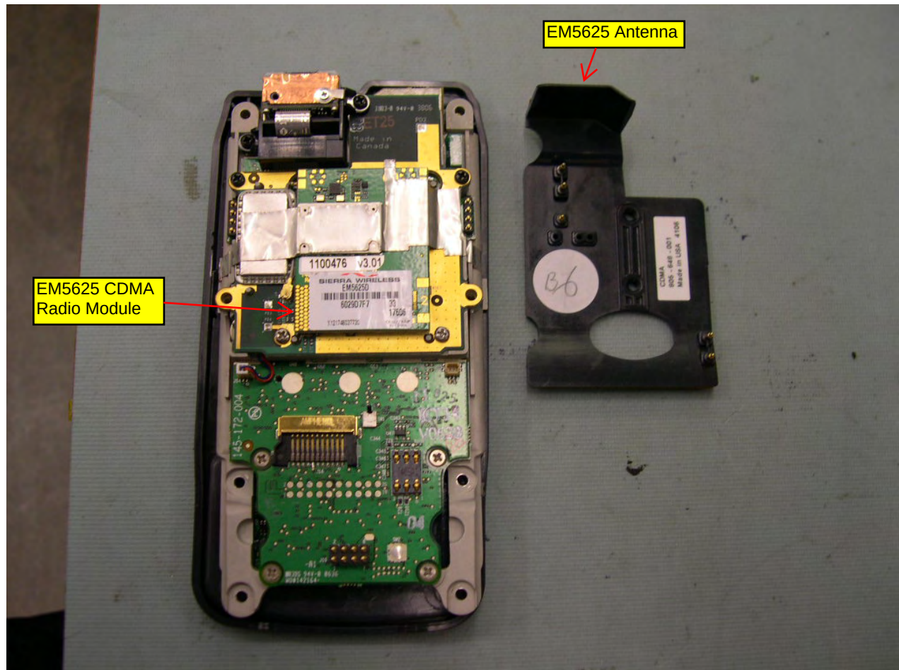
CN3 Case Back with EM5625 and Antenna removed from case
