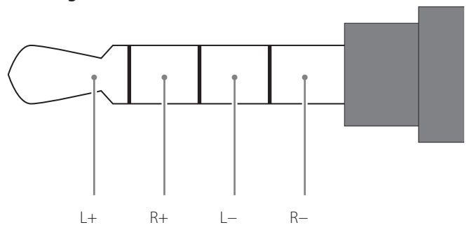
Wiring illustration
