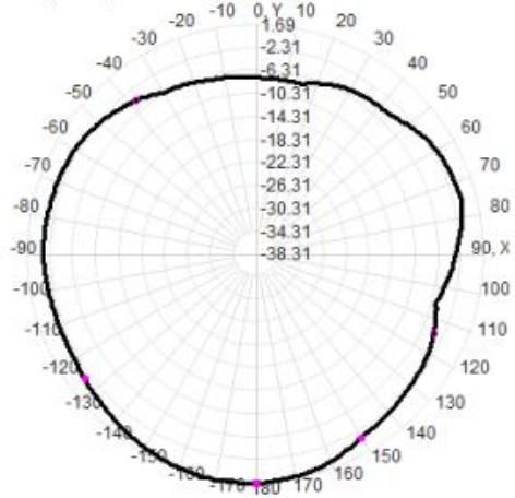
Total(H-XY), Max= 1.69dBi, CirD=9.36
