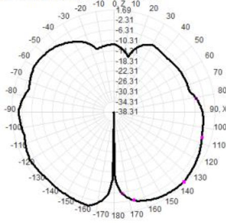
2470.0MHz Total(E1-XZ), Max= 0.62dBi
