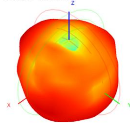
2460.0MHz H+V, Eff: 56.8%
