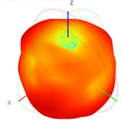
2460.0MHz H+V, Eff: 56.4%
