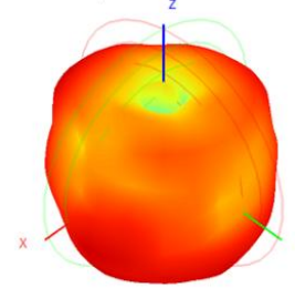
2470.0MHz H+V, Eff: 56.9%
