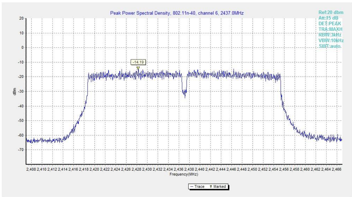
Fig.A.3.35 Power Spectral Density (802.11n-HT40, Ch 6)
