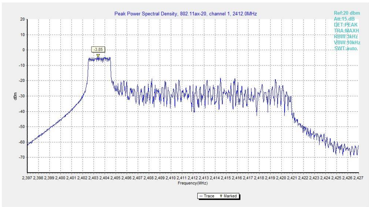
Fig.A.3.25 Power Spectral Density (802.11ax-HE20 RU26-index0, Ch 1)
