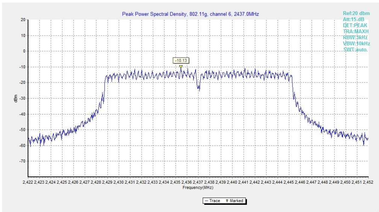
Fig.A.3.23 Power Spectral Density (802.11g, Ch 6)
