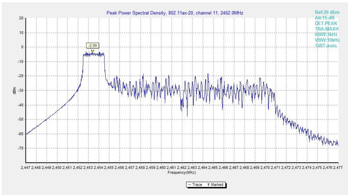
Fig.A.3.15 Power Spectral Density (802.11ax-HE20 RU26-index0, Ch 11)
