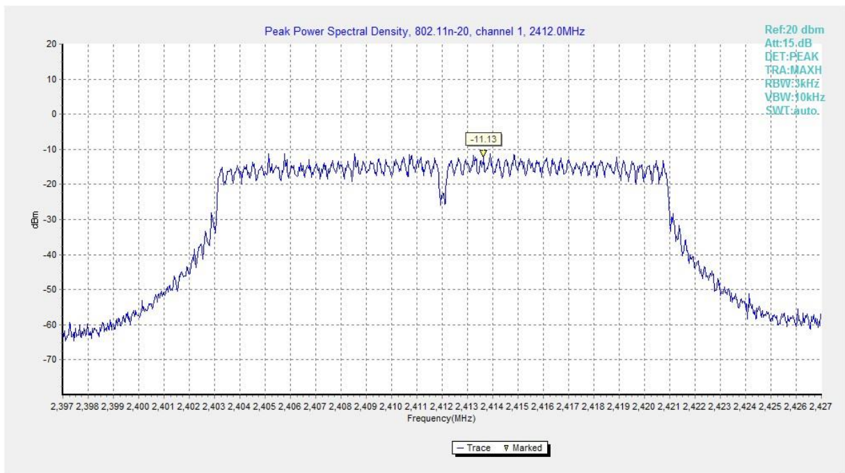
Fig.A.3.31 Power Spectral Density (802.11n-HT20, Ch 1)
