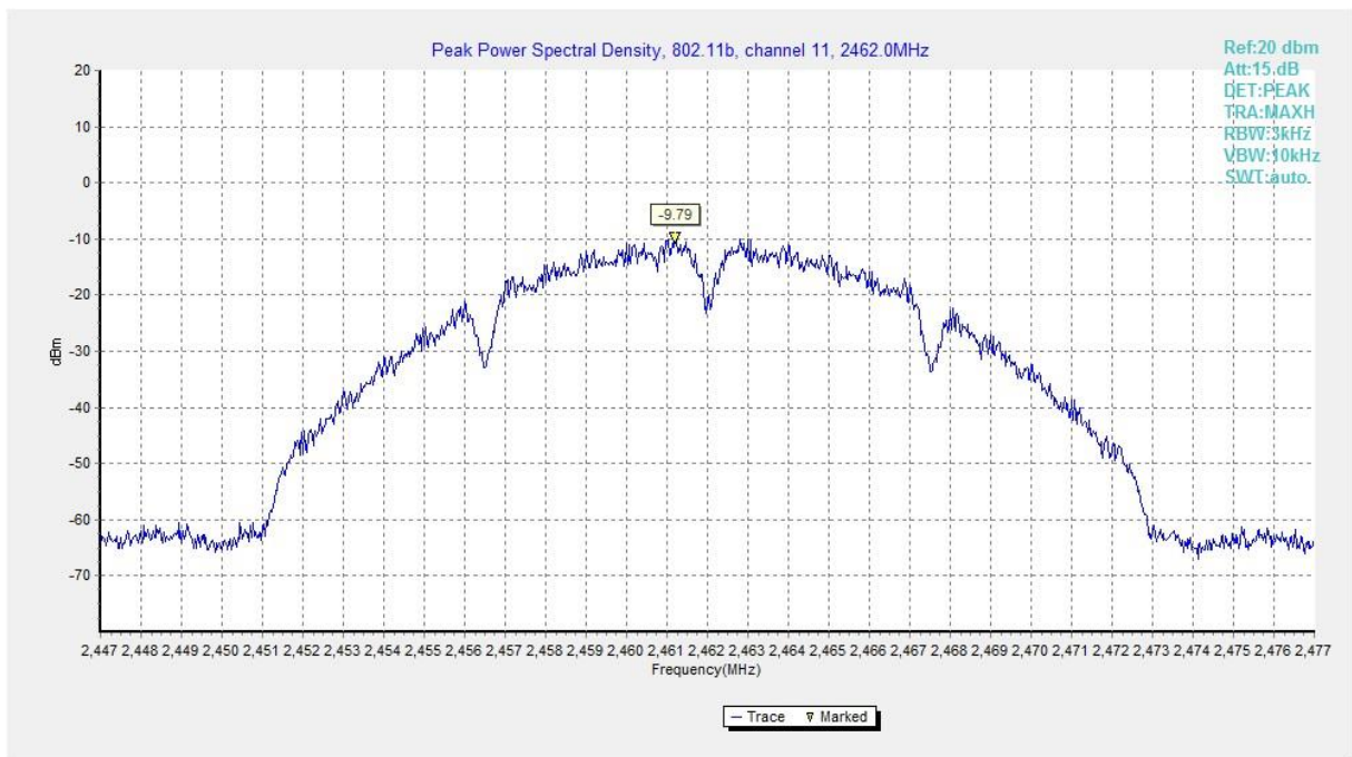
Fig.A.3.21 Power Spectral Density (802.11b, Ch 11)
