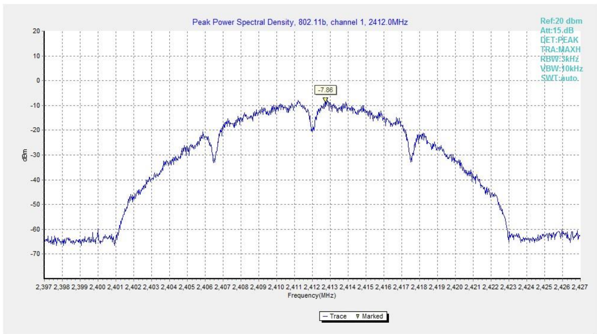
Fig.A.3.19 Power Spectral Density(802.11b,Ch1)
