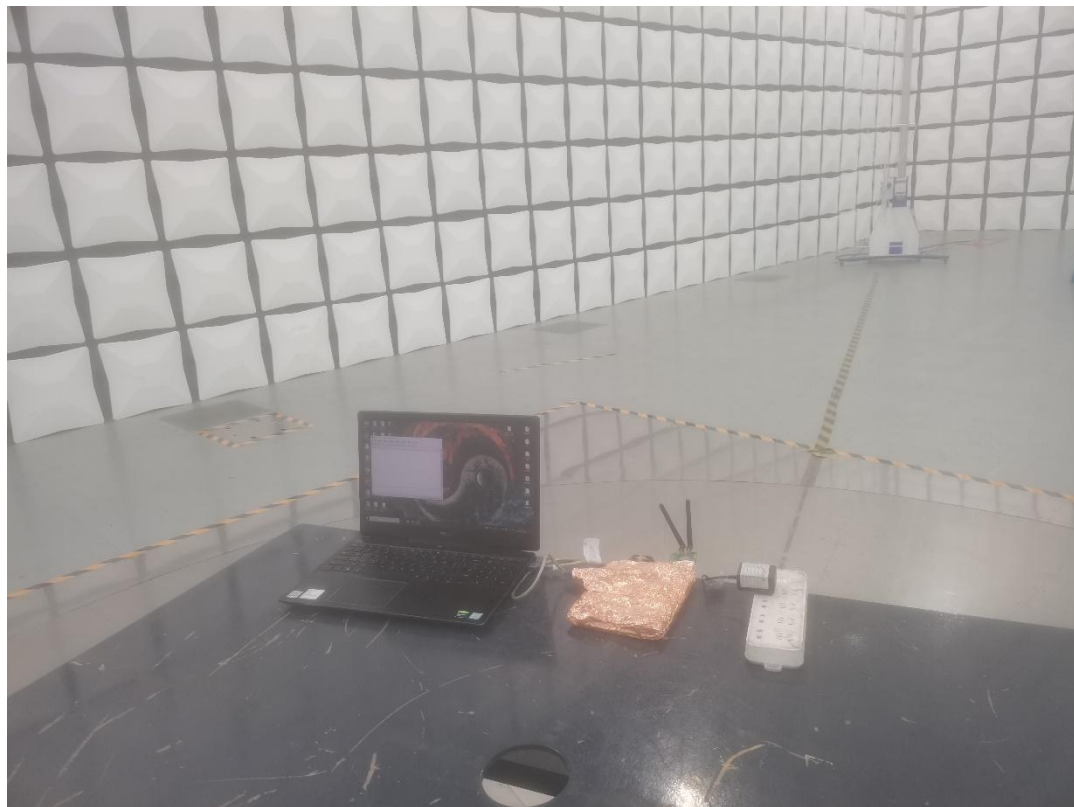
30MHz~1GHz
