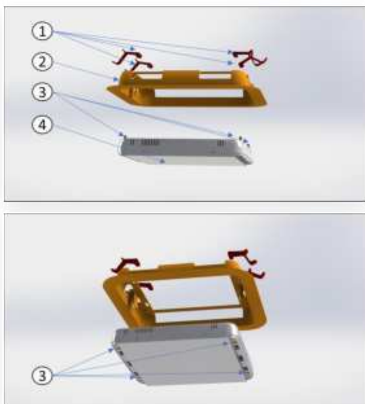
Figure 9 - Flush mounting kit – Installation illustration
