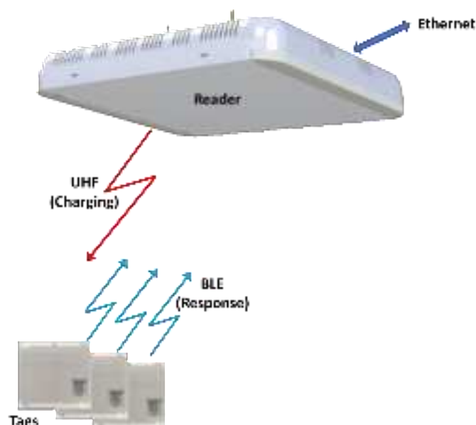
Figure 2 - Reader's functionality
