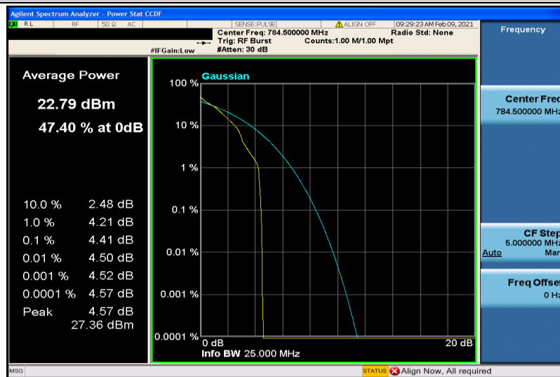
Band13-5MHz-QPSK-23255-1RB#0
