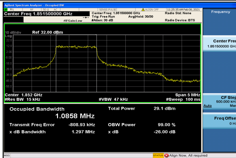
Band2-3MHz-QPSK-18615-6RB#0-1.0858
