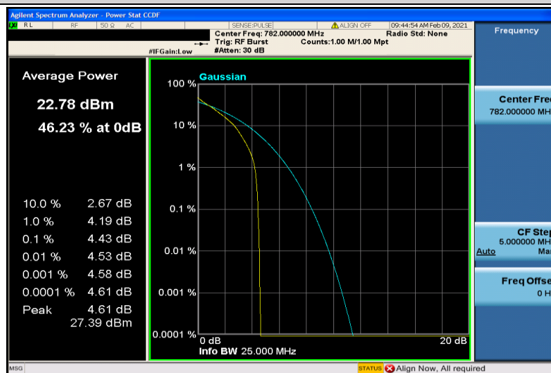
Band13-10MHz-QPSK-23230-6RB#0
