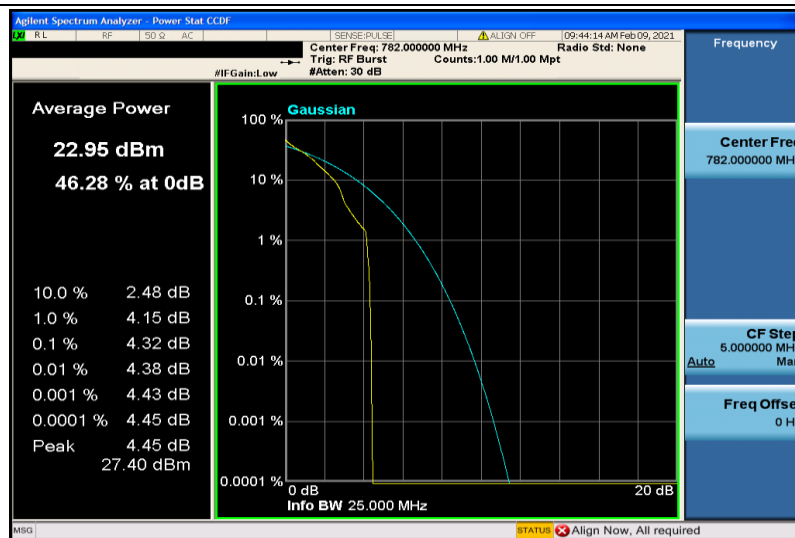
Band13-10MHz-QPSK-23230-1RB#0
