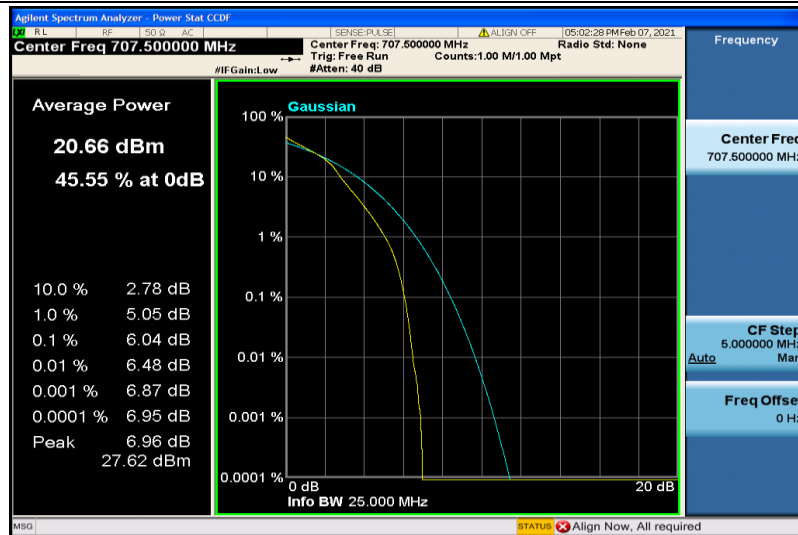
Band12-5MHz-16QAM-23095-6RB#0
