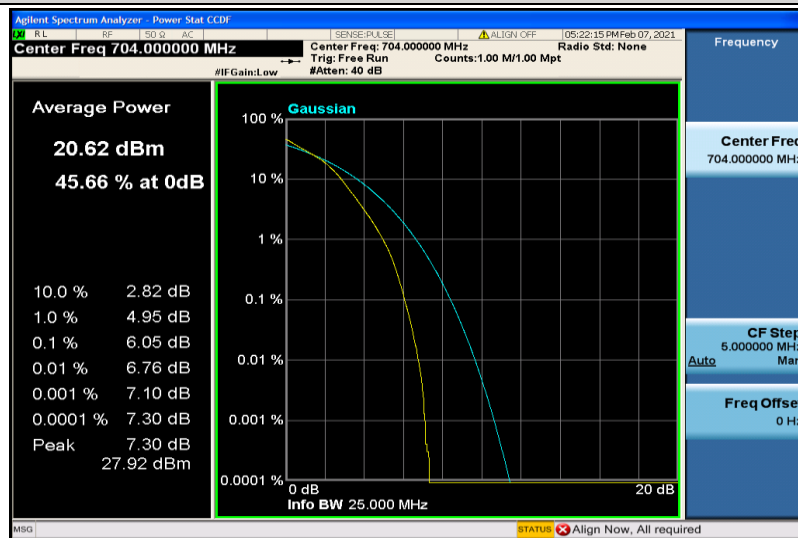
Band12-10MHz-16QAM-23060-6RB#0
