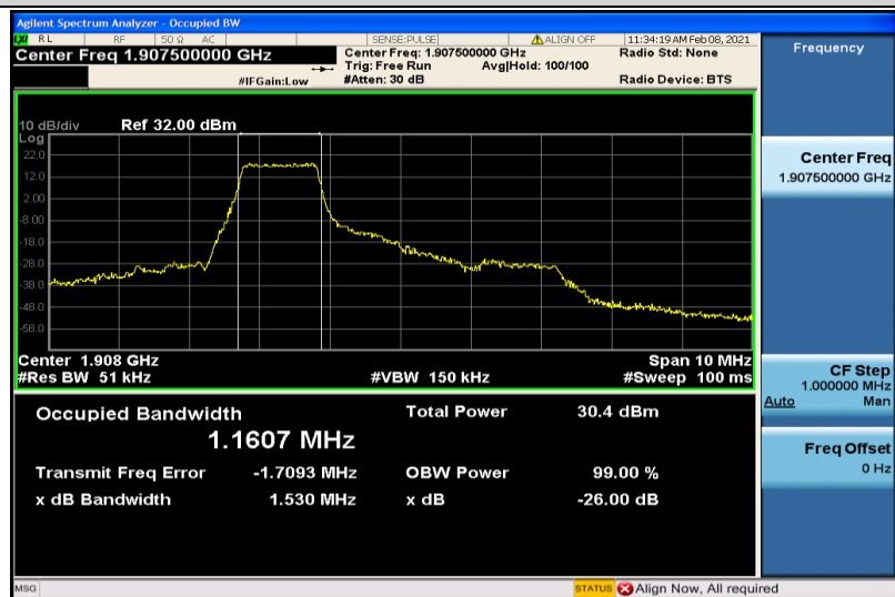
Band2-5MHz-QPSK-19175-6RB#0-1.1607
