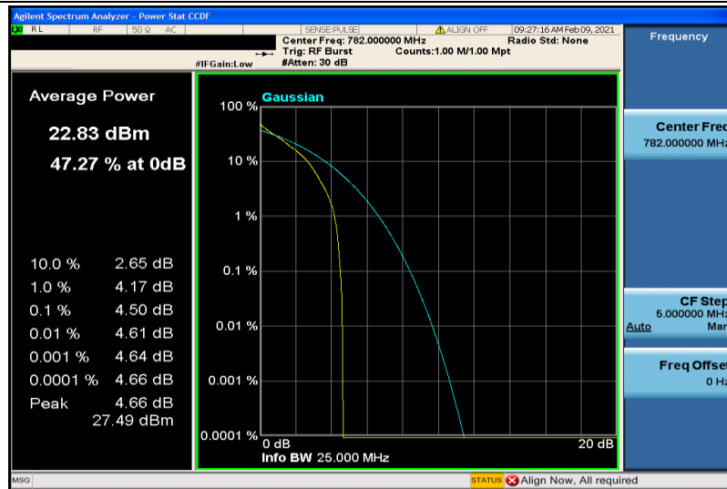
Band13-5MHz-QPSK-23230-6RB#0
