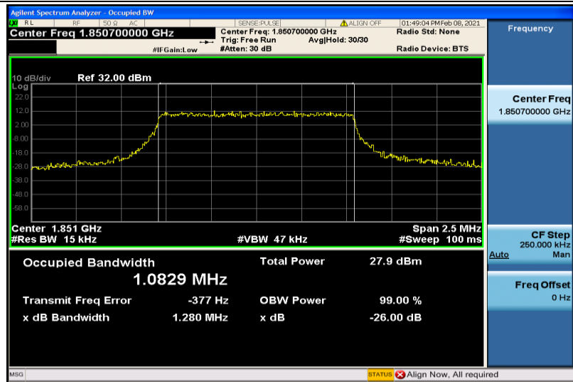
Band2-1.4MHz-16QAM-18607-6RB#0-1.0829
