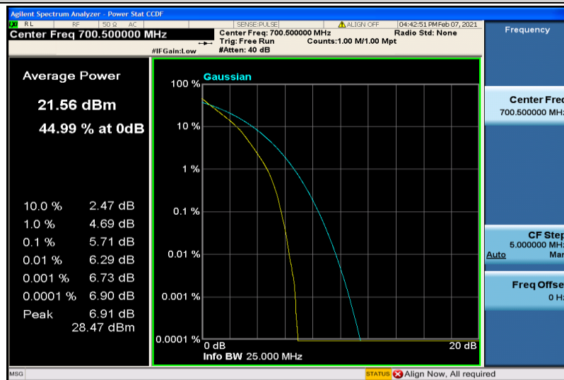
Band12-3MHz-QPSK-23025-6RB#0
