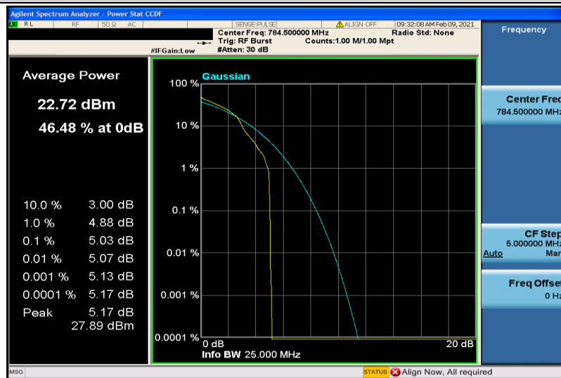
Band13-5MHz-16QAM-23255-1RB#0
