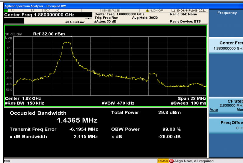
Band2-15MHz-16QAM-18900-6RB#0-1.4365
