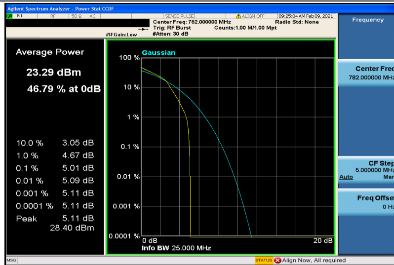
Band13-5MHz-16QAM-23230-6RB#0
