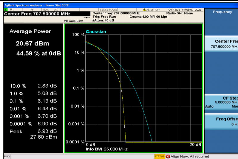
Band12-3MHz-16QAM-23095-6RB#0
