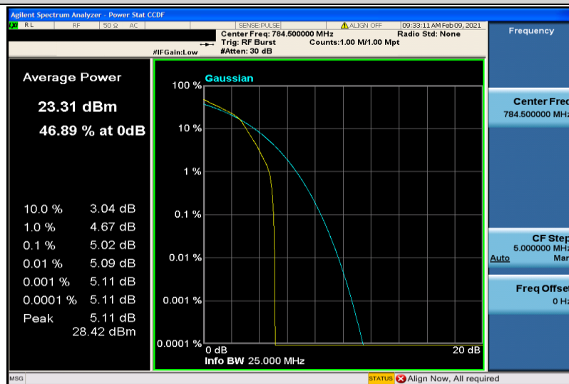
Band13-5MHz-16QAM-23255-6RB#0
