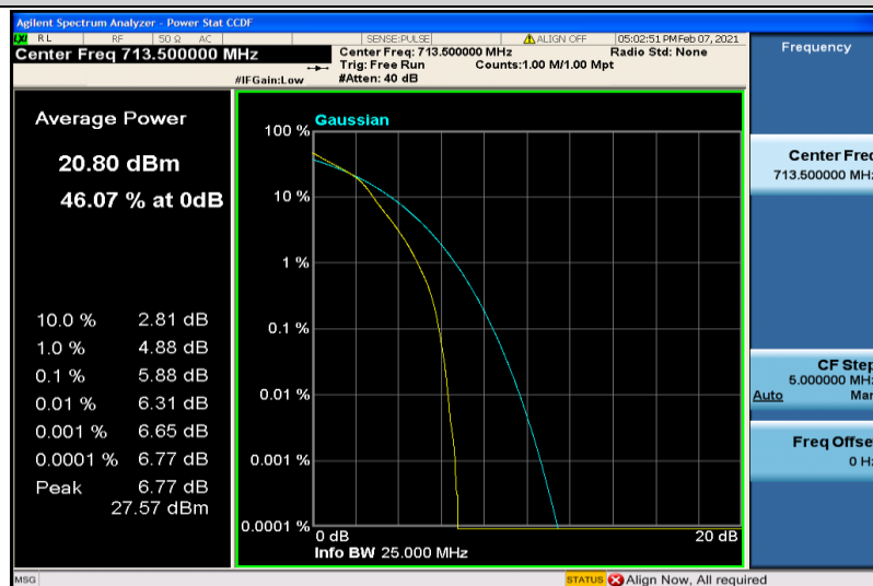
Band12-5MHz-16QAM-23155-6RB#0
