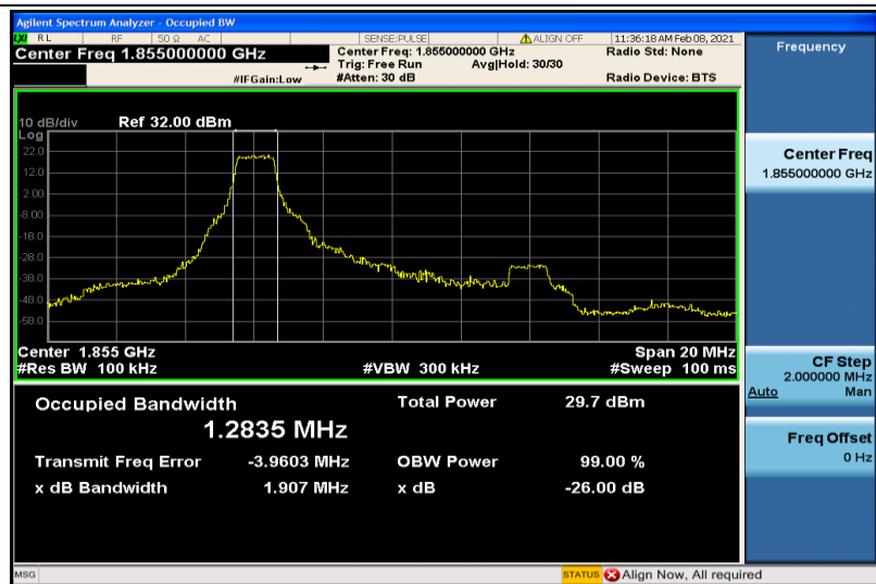
Band2-10MHz-16QAM-18650-6RB#0-1.2835
