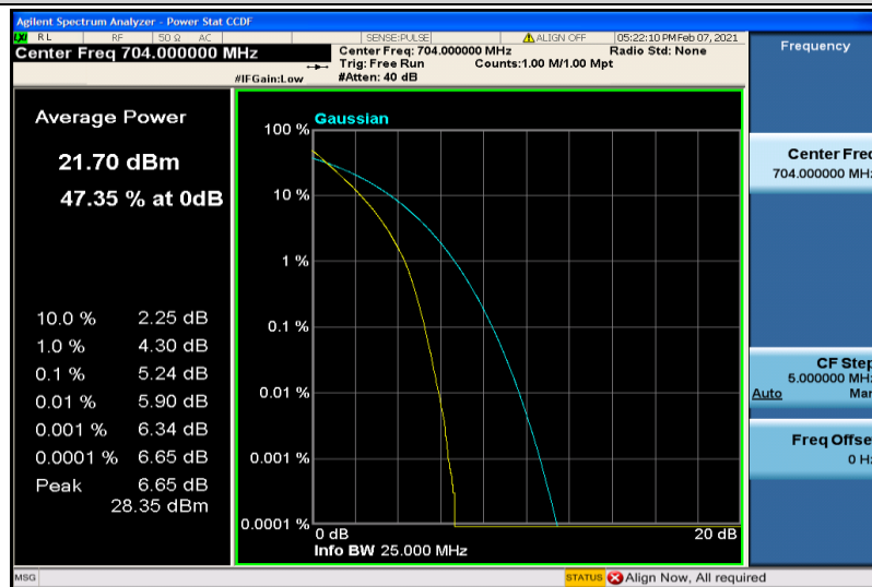
Band12-10MHz-QPSK-23060-6RB#0
