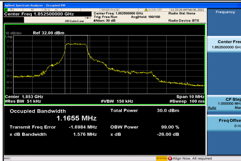
Band2-5MHz-16QAM-18625-6RB#0-1.1655
