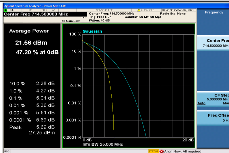
Band12-3MHz-QPSK-23165-6RB#0
