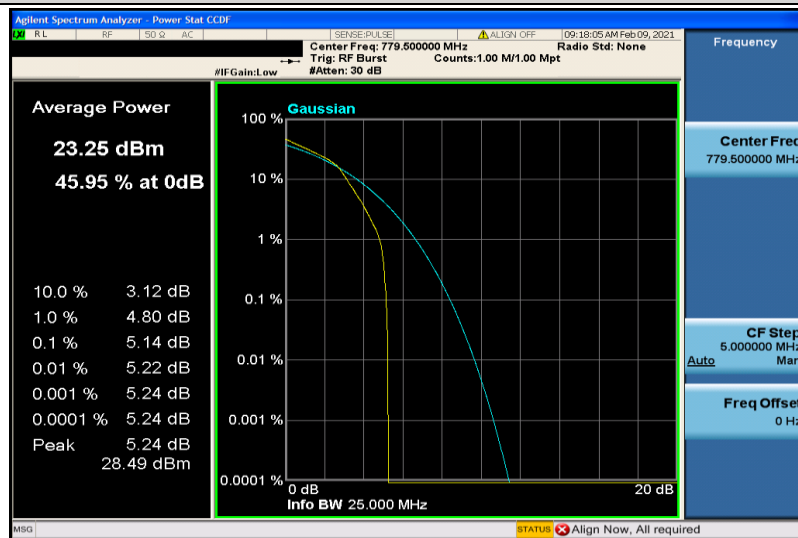
Band13-5MHz-16QAM-23205-6RB#0
