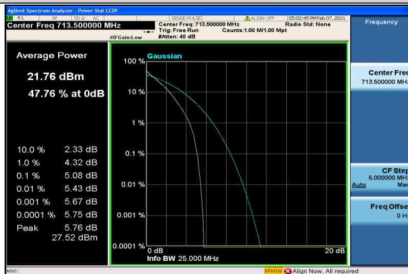
Band12-5MHz-QPSK-23155-6RB#0
