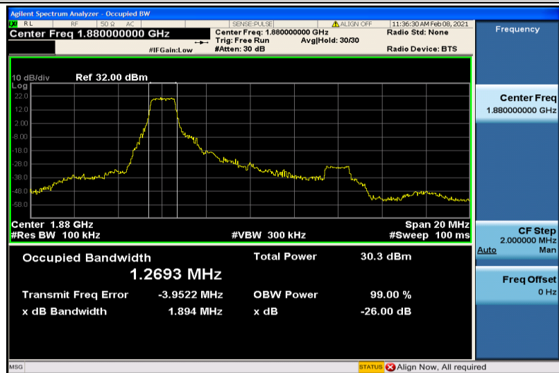
Band2-10MHz-QPSK-18900-6RB#0-1.2693
