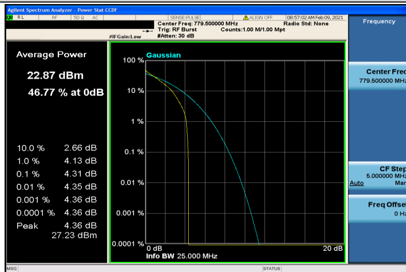
Band13-5MHz-QPSK-23205-6RB#0
