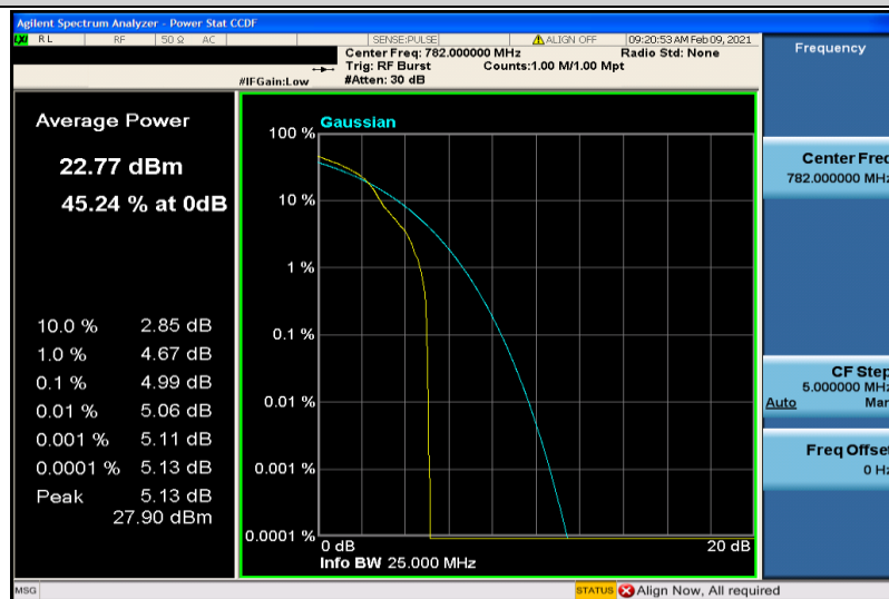
Band13-5MHz-16QAM-23230-1RB#0
