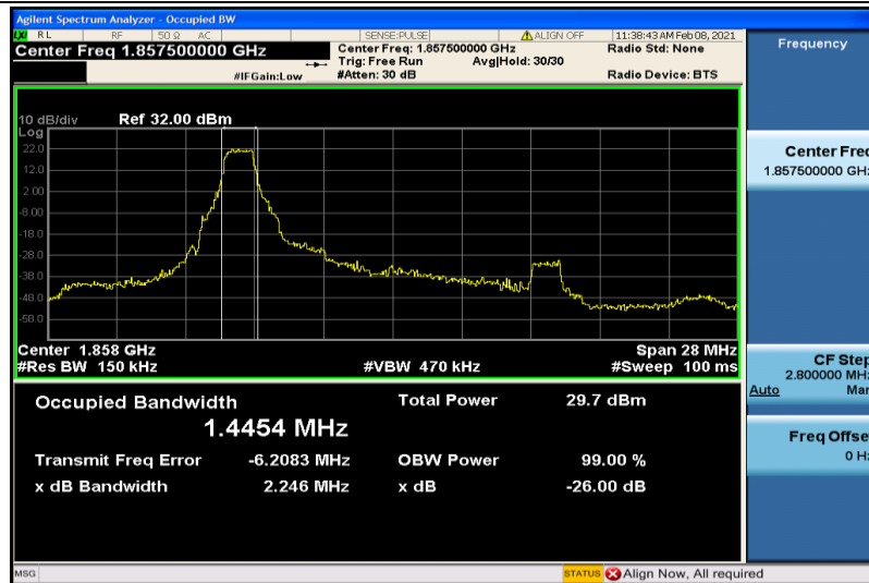
Band2-15MHz-16QAM-18675-6RB#0-1.4454
