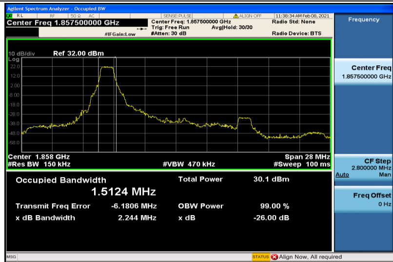
Band2-15MHz-QPSK-18675-6RB#0-1.5124
