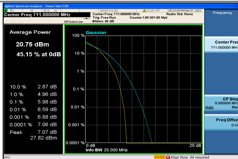
Band12-10MHz-16QAM-23130-6RB#0
