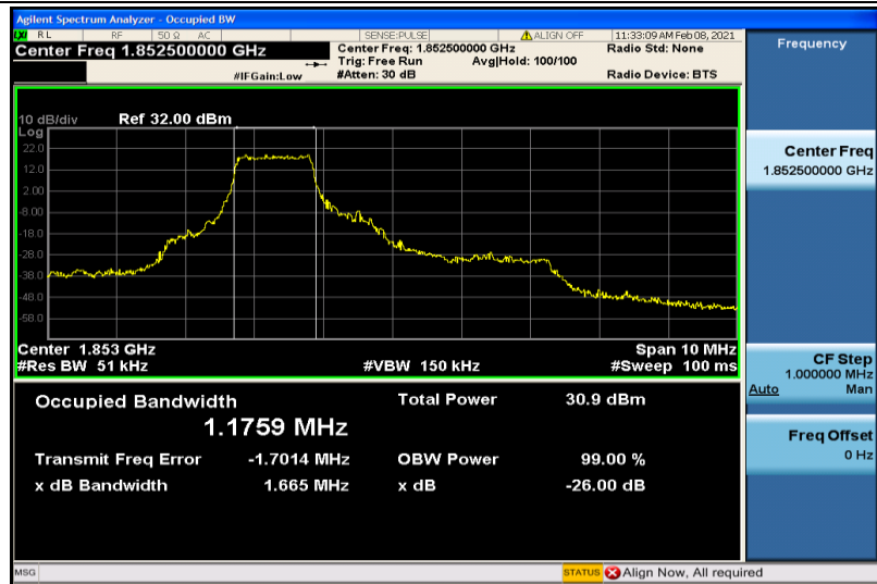
Band2-5MHz-QPSK-18625-6RB#0-1.1759
