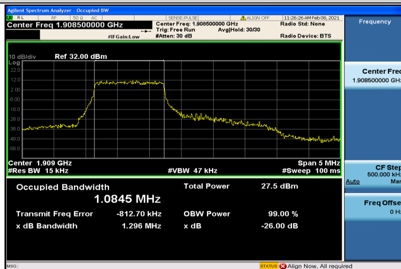
Band2-3MHz-16QAM-19185-6RB#0-1.0845
