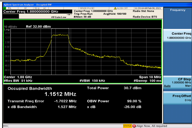
Band2-5MHz-QPSK-18900-6RB#0-1.1512
