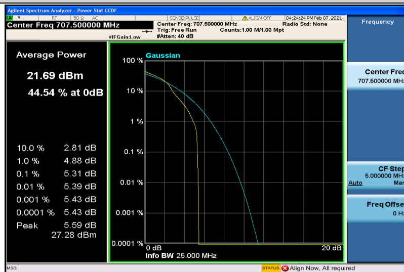
Band12-1.4MHz-16QAM-23095-1RB#0
