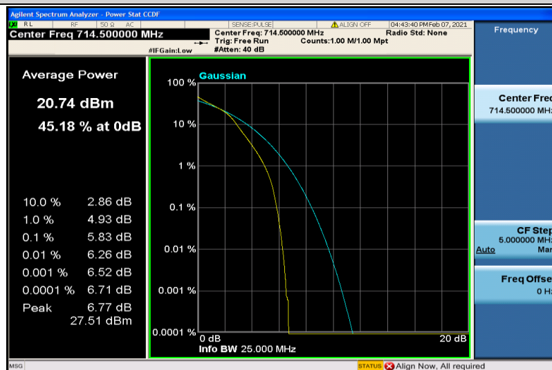
Band12-3MHz-16QAM-23165-6RB#0
