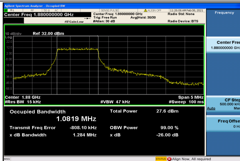
Band2-3MHz-16QAM-18900-6RB#0-1.0819
