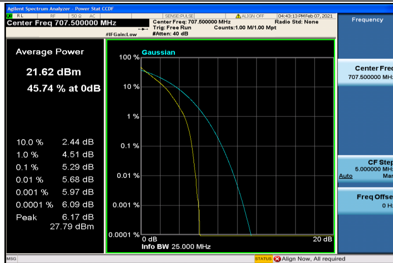
Band12-3MHz-QPSK-23095-6RB#0
