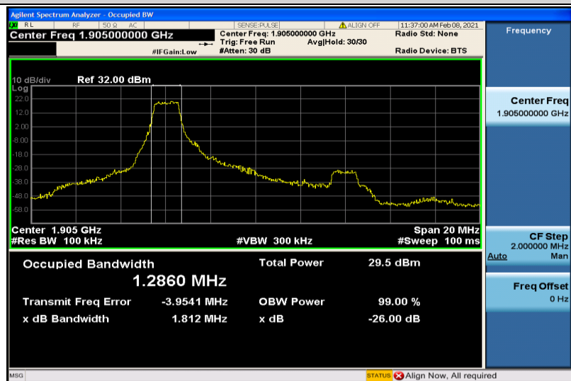
Band2-10MHz-16QAM-19150-6RB#0-1.2860
