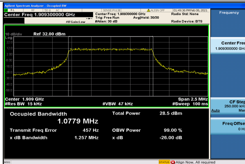
Band2-1.4MHz-QPSK-19193-6RB#0-1.0779
