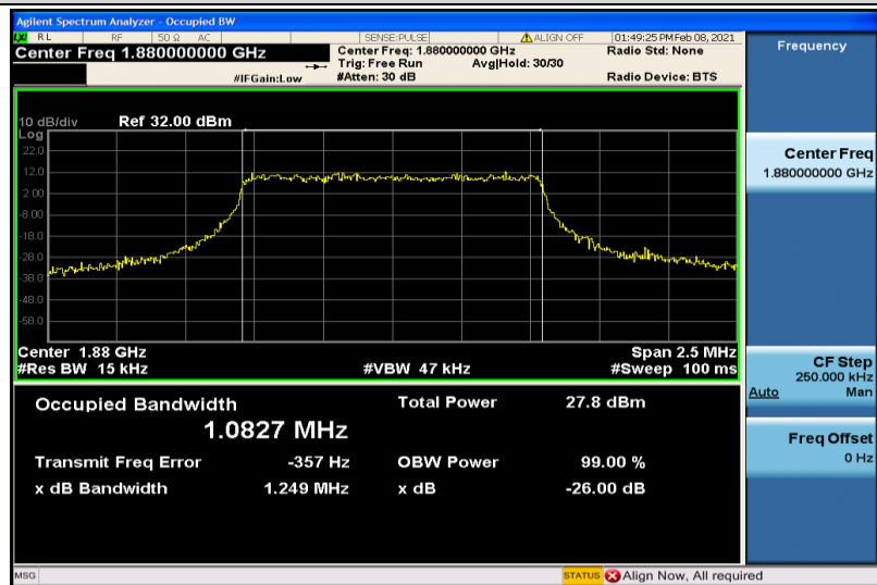
Band2-1.4MHz-16QAM-18900-6RB#0-1.0827
