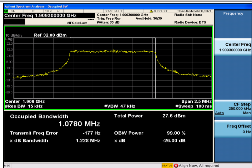
Band2-1.4MHz-16QAM-19193-6RB#0-1.0780
