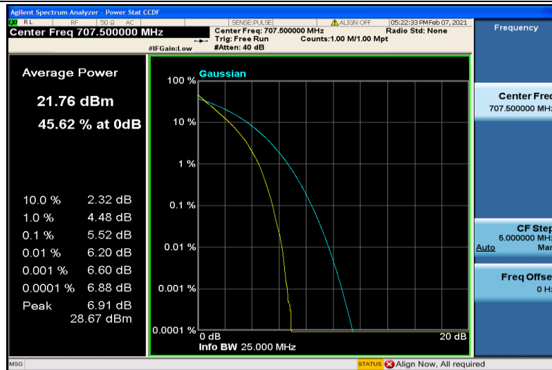
Band12-10MHz-QPSK-23095-6RB#0
