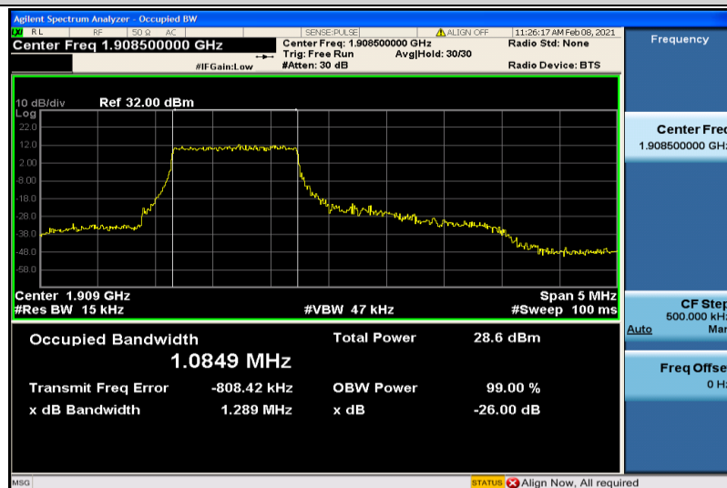
Band2-3MHz-QPSK-19185-6RB#0-1.0849
