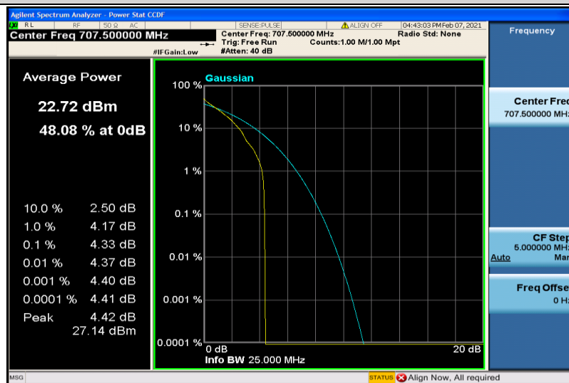
Band12-3MHz-QPSK-23095-1RB#0
