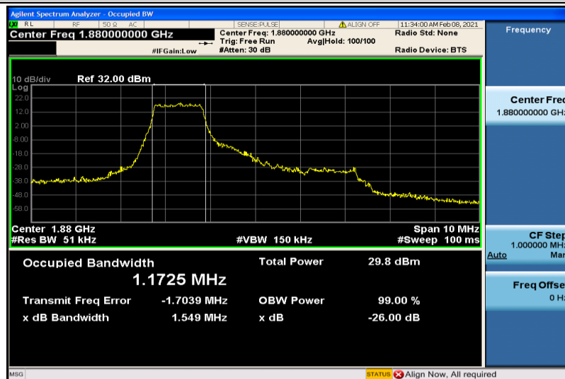
Band2-5MHz-16QAM-18900-6RB#0-1.1725
