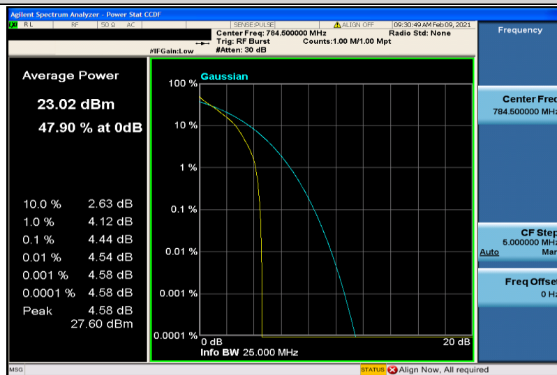
Band13-5MHz-QPSK-23255-6RB#0
