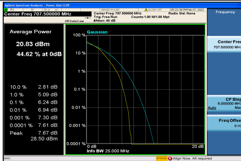
Band12-10MHz-16QAM-23095-6RB#0
