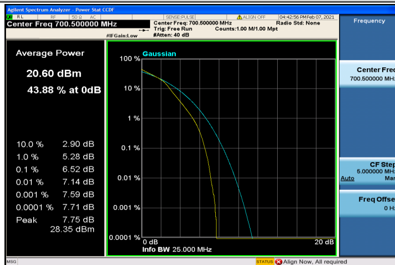
Band12-3MHz-16QAM-23025-6RB#0
