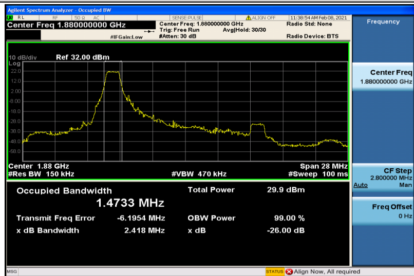
Band2-15MHz-QPSK-18900-6RB#0-1.4733
