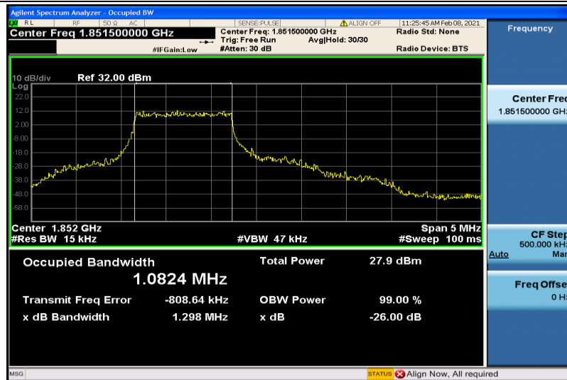
Band2-3MHz-16QAM-18615-6RB#0-1.0824
