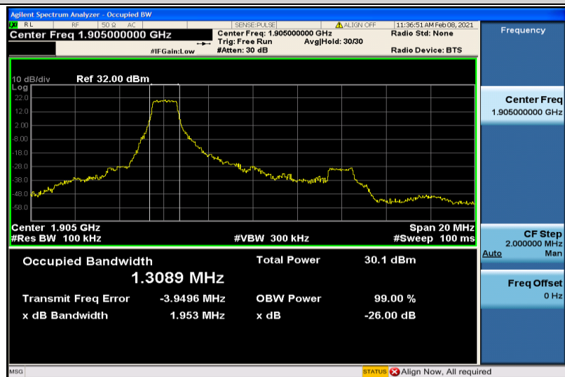
Band2-10MHz-QPSK-19150-6RB#0-1.3089
