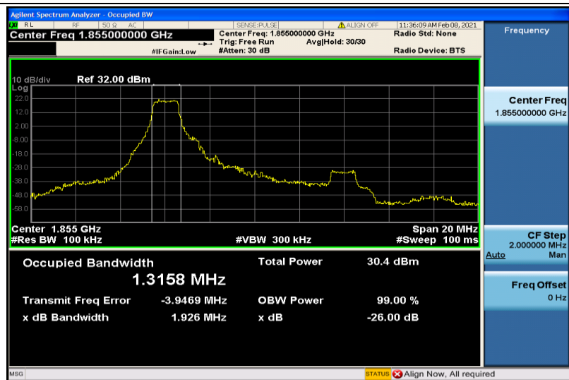
Band2-10MHz-QPSK-18650-6RB#0-1.3158
