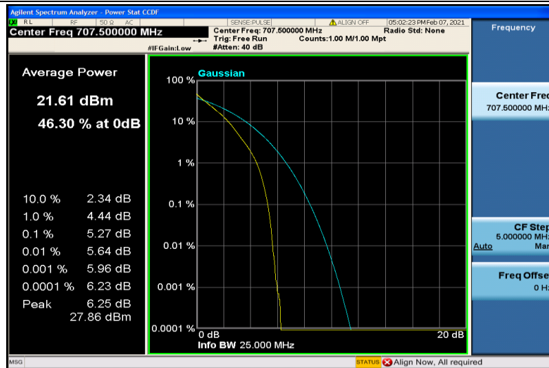
Band12-5MHz-QPSK-23095-6RB#0
