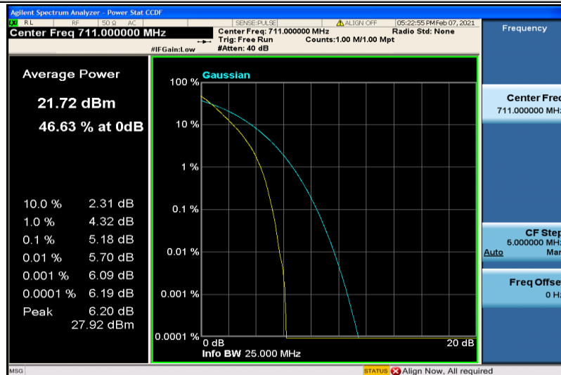
Band12-10MHz-QPSK-23130-6RB#0
