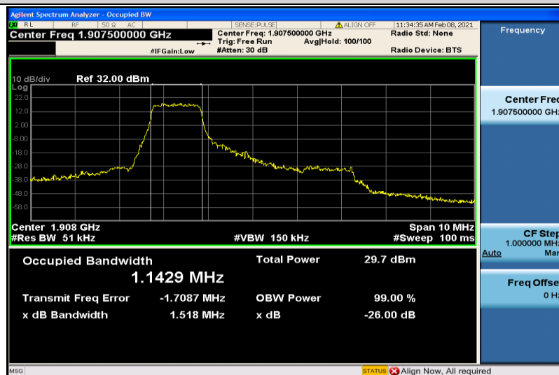
Band2-5MHz-16QAM-19175-6RB#0-1.1429
