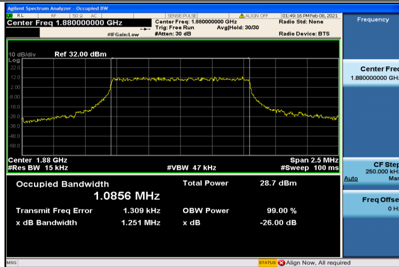
Band2-1.4MHz-QPSK-18900-6RB#0-1.0856
