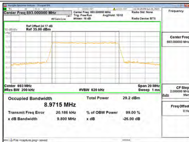
Band71 / 10MHz / 16QAM/ High CH
