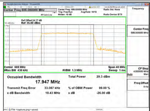
Band71 / 20MHz / 64QAM/ High CH
