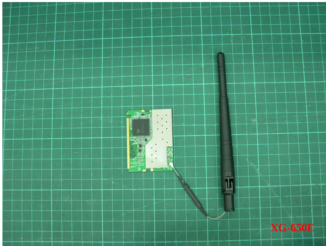
Antenna 2
