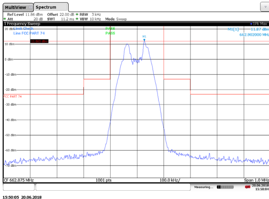
Plot 5: 662.875 MHz, spectrum mask
