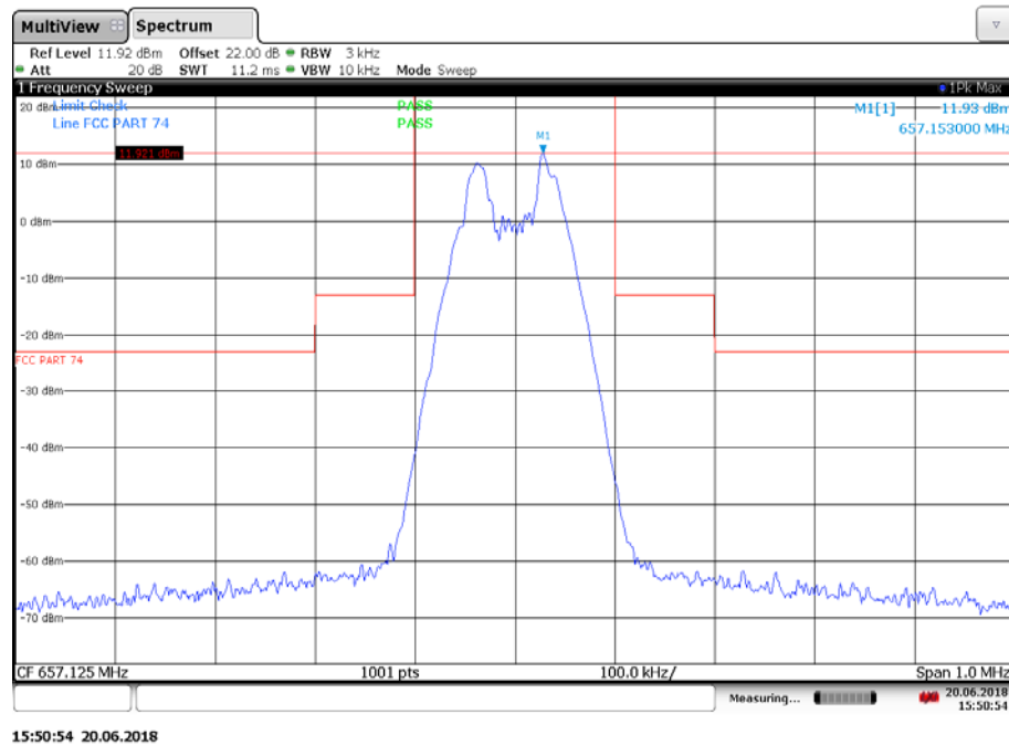
Plot 4: 657.125 MHz, spectrum mask
