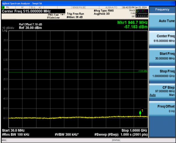
Band4_20MHz_QPSK_20300_1RB#0_30~1000_30~1000
