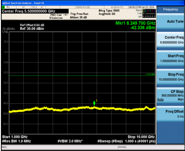
Band5_5MHz_16QAM_20525_1RB#0_1000~10000_1000~10000
