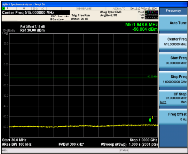
Band4_15MHz_QPSK_2025_1RB#0_30~1000_30~1000
