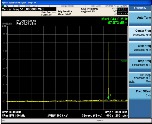
Band5_1.4MHz_QPSK_20643_1RB#0_30~1000_30~1000
