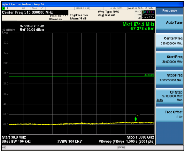
Band4_20MHz_16QAM_20175_1RB#0_30~1000_30~1000
