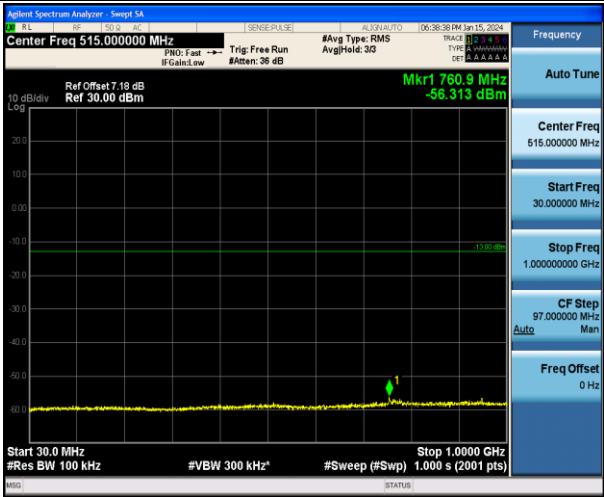
Band4_20MHz_QPSK_20050_1RB#0_30~1000_30~1000
