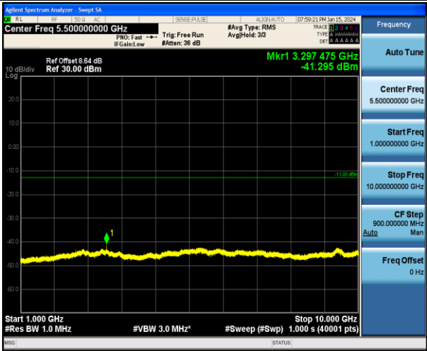
Band5_5MHz_16QAM_20425_1RB#0_1000~10000_1000~10000
