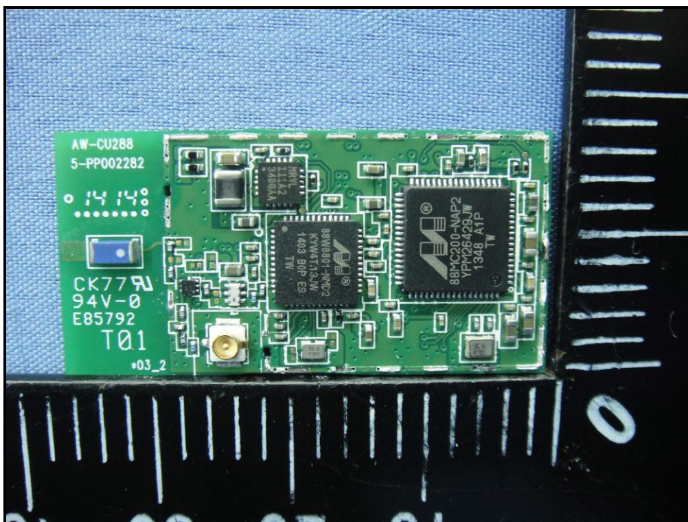
Antenna: ANT3216LL00R2400A
